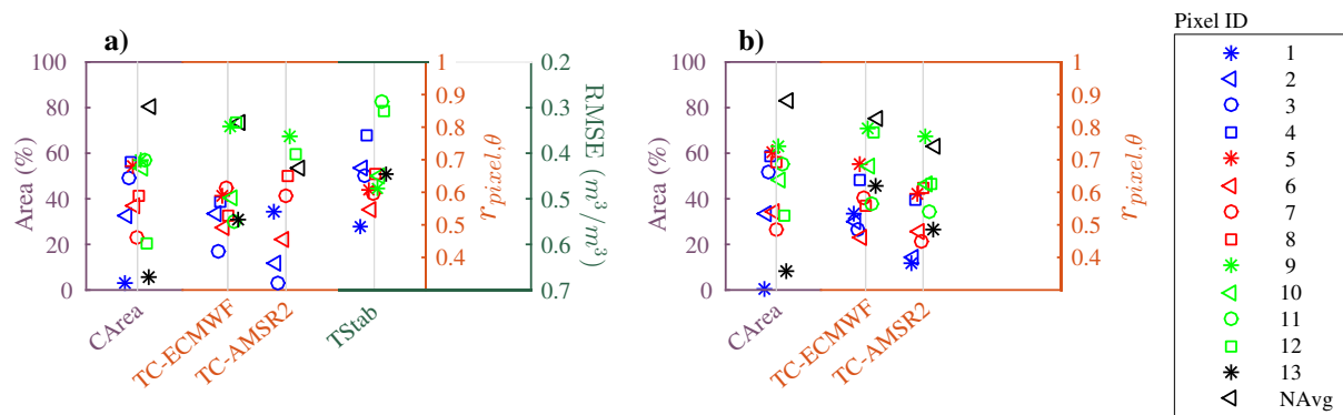
Figure 4.5 – Spatial representativeness scores (vertical axis) from different methods (horizontal axis) for different pixels of the gridded SM dataset. The representativeness is evaluated on a) full series and on b) detrended series (components > 32 days are removed). The CArea correlation threshold is 0.55. Source: (Molero et al., 2018)
