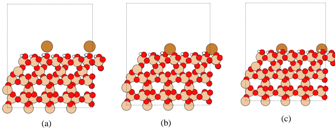
Figure 4- 13 Different adsorption sites of copper on \text{SiO}_2 , top site (a), bridge site (b) and hollow site (c)
