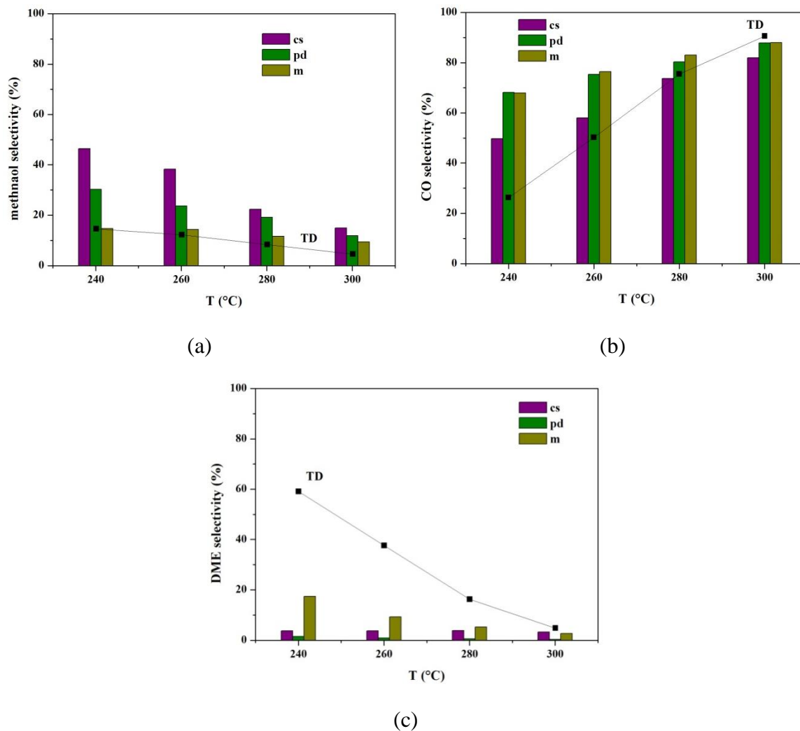
Figure 5-9Methanol (a), CO (b) and DME (c) selectivity
