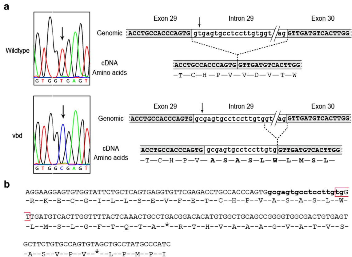
Fig. 4 Sequence analysis spanning the vbd mutation site. a (Left) Sequence chromatograph of the otog gene at the level of the splicing site exon 29/intron 29 showing the T > C transition (arrows); (right) partial genomic sequence of the region spanning exon 29 to exon 30 with the corresponding cDNA and amino acid sequence. Top: wildtype; bottom: Otog vbd/vbd mutant. b cDNA sequence surrounding the vbd mutation showing the insertion of 17 bp (lowercase bases in bold) including a new splicing site (open red box). The resulting reading frame shift leads to a premature stop codon in the amino acid sequence between VWFD 3 and VWFD 4 domain (uniprot)
