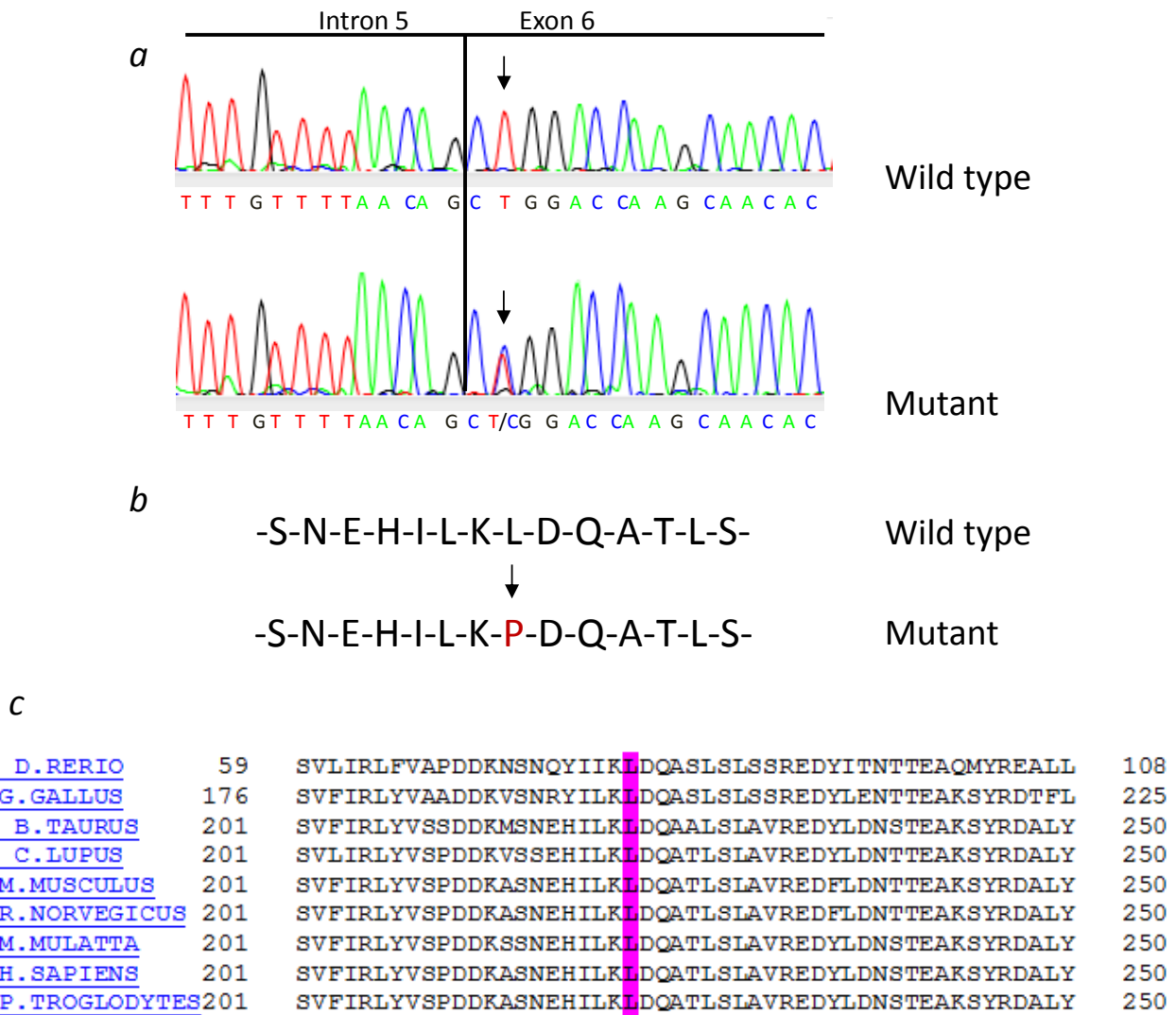
Figure 4: Sequence analysis spanning Phex L222P mutation site in a female. (a) Sequence chromatograph of the Phex gene at the level of the splicing site intron5/exon6 showing the T > C transition (arrows) with the corresponding amino acid sequence (b). (b) The resulting PHEX amino acids sequence with the changed amino acid coloured in red. (c) Partial protein alignment of PHEX gene from different species around the mutation position (amino acid 222 in mice) executed with Homologene database. The Leucine residue at position 222, colored in magenta, is highly conserved between the species.
