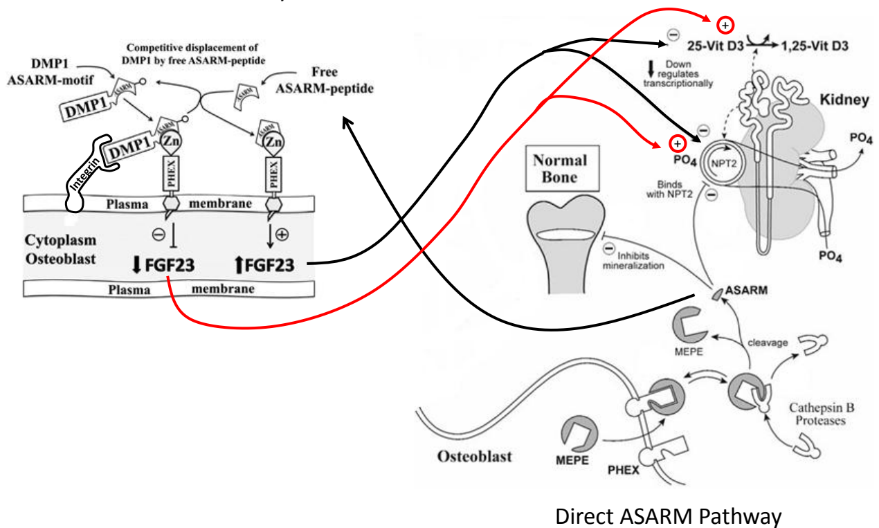
Figure 7: Predicted ASARM pathway in PHEX regulation of bone mineral and renal phosphate reabsorption. Phosphorylation of DMP1-ASARM motif is requisite for the formation of a PHEX/DMP1/ \alpha 5\beta 3 -integrin complex on the surface of osteocytes or osteoblasts. This induces a down regulation of FGF23 and affects, in turn, renal PO 4 handling by increasing renal NPT2 (Na-Pi IIa renal cotransporter) and 1 \alpha hydroxylase expression. 1 \alpha hydroxylase is necessary for the transformation of 25-Vitamin D3 to its active form (1.25-Vit D3). PHEX also sequesters and, thus, transiently protects MEPE from extracellular-matrix Cathepsin B protease which cleaves MEPE and releases a free ASARM peptide. Free ASARM peptide could directly inhibit bone mineralization, by reducing renal phosphate reabsorption through a direct reduction of NPT2 expression or indirectly through the increasing of FGF23 expression by binding to PHEX. Thus, FGF23 increased level will decrease NPT2 and 1 \alpha hydroxylase expression. Modified from Rowe 2004; David et al. 2011
