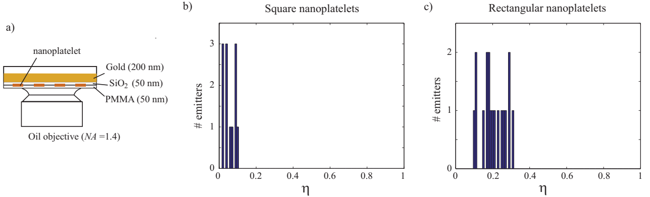
FIGURE 5.21: (a) Schematic of the investigated objective-sample configuration. Histogram of the dipolar asymmetric factor \eta measured for (b) 13 square platelets and (c) for 18 rectangular platelets.
