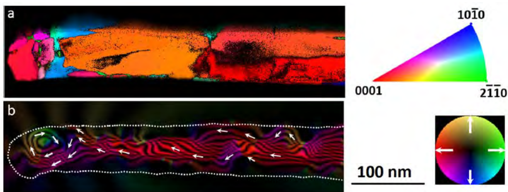
Figure 4.1.2. a) Crystal orientation and b) magnetic phase contour maps of the Co nanowire. The crystal orientation map is displayed with respect to the direction of observation z (color key code displayed on the right) and is over-layered with the reliability map to reveal zones where crystallites overlap. The magnetic phase contour map is obtained by amplifying 3 times the cosine of the unwrapped magnetic phase (magnetic flux direction color-wheel displayed on the right). The outline of the nanowire is marked by the thin white line.
