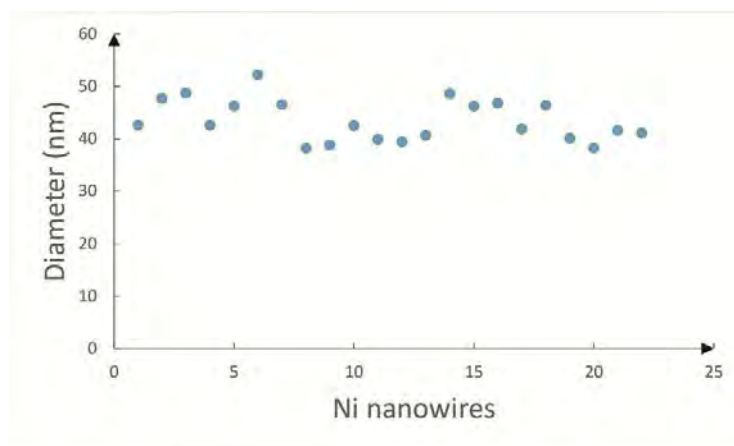
Figure 3.2.10. Distribution of diameters for Ni NWs
