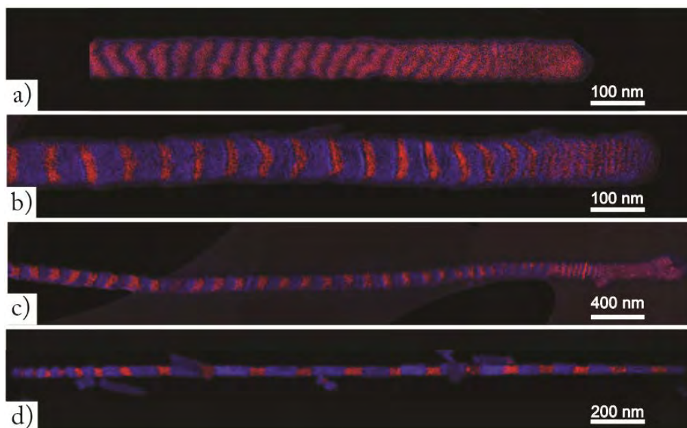
Figure 4.4.6. EFTEM elemental maps, in red Co and Cu in blue for Co/Cu NWs with configurations of: a) 25/15, b) 25/45, c) 50/50 and d) 100/100. The NWs ends show a decreasing of the thickness layer compare to its central part.
