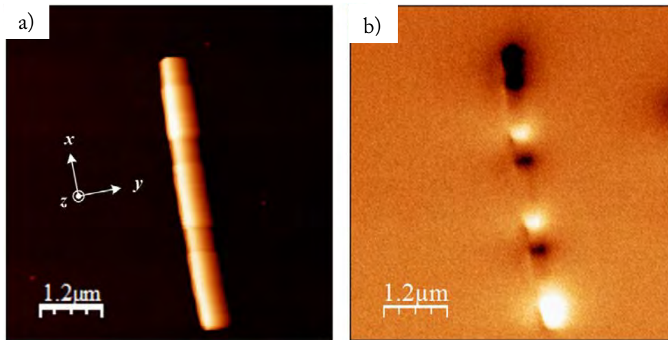
Figure 5.4.1. a) Topographic and b) MFM images for a DM FeCoCu NW of intermediate length.
