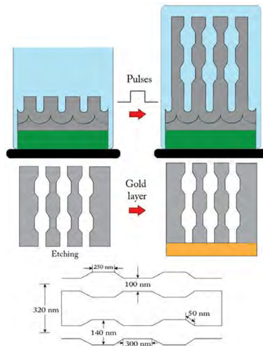
Figure 5.2.2. Scheme of the pores formation and the preparation to deposit the NWs. The last part of the figure details the geometrical parameters of the pores.
