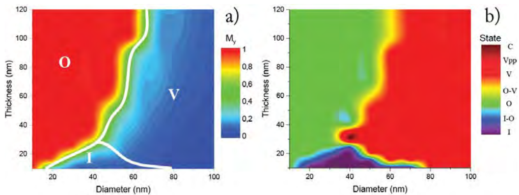
Figure 4.6.3. Phase diagram for Co nanocylinders with a magnetocrystalline anisotropy of 100 \times 10^3 \text{ J/m}^3 oriented 20^\circ respect to the wire axis and absence of a magnetic field: a) Colour representation with the Y component of the magnetization, b) Colour representation of the main magnetic states and intermedia states.
