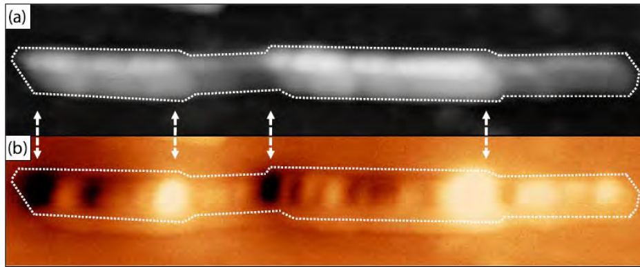
Figure 5.1.2. a) Topography and b) MFM images of a single FeCoCu NW in remanence. Extracted from [29].
