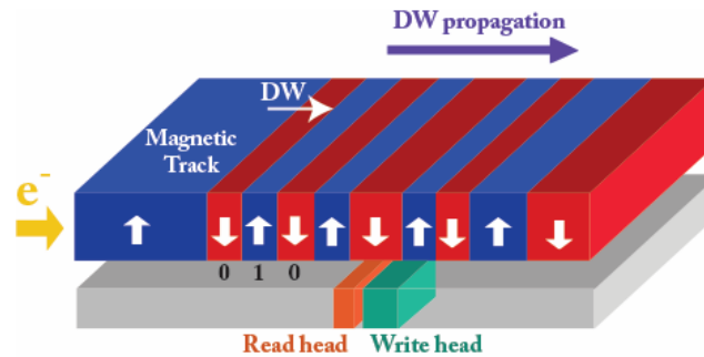
Figure 2. Racetrack memory proposed by S.S. Parkin et al. [66].
