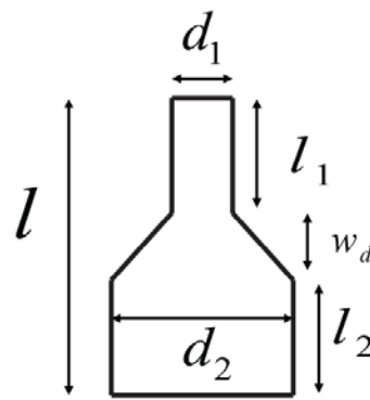
Figure 5.1.1. Diameter-modulated NW studied by Allende et al. Extracted from [17].
