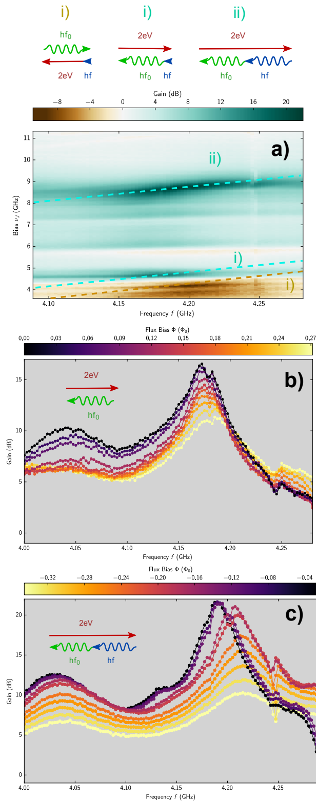
Figure 6.4 The ICTA gain: a) The gain as a function of the voltage bias \nu_J and the frequency f for a flux bias \Phi = -0.04\Phi_0 . The green lines show the amplification processes. The brown lines show the conversion process b) The ICTA gain as a function of the frequency at the resonance condition of the one photon peak at \nu_J = 4.6 GHz for various flux biases. c) The ICTA gain as function of the frequency at the resonance condition of the two photon peak at \nu_J = 8.8 GHz for various flux biases.
