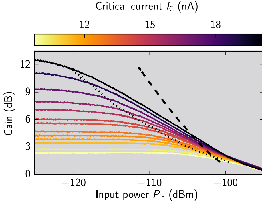
Figure 3.6 Dynamic range: Gain as a function of the input power P_{in} for different Josephson energies at \nu_J = 12.15 GHz and f = 6.05 GHz. The dotted line represents the input 1 dB compression points.
