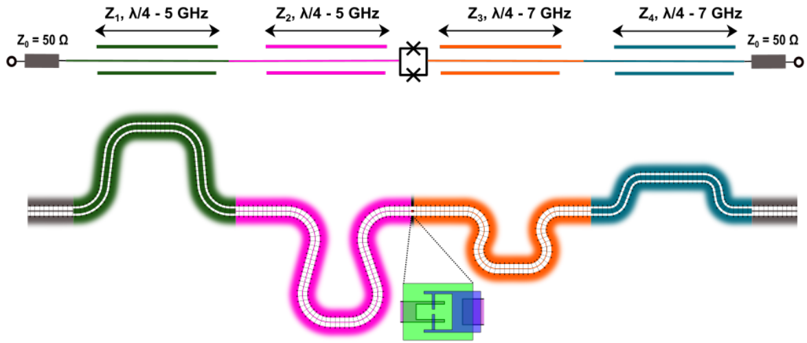
Figure 4.5 "Canonical" non-degenerate amplifier with two separate modes ( S_1 ) : For better visibility the color scheme is chosen differently than in the rest of this work. we associate one color for each quarter-wave resonator to show the coupling between the resonators. The green and the fuchsia resonators, together, form the signal mode at 5 GHz. The orange and the blue resonators, together, form the idler mode at 7 GHz. A zoom on the entire SQUID is located in the bottom of the image. For the SQUID, we kept the same color than the rest of this work. The violet color indicates the trilayer, the blue color indicates the NbN Top wiring and finally the green color indicates the area where we etch the \text{Si}_3\text{N}_4 dielectric. Table 4.1 indicates values of the four quarter-wave segments we have implemented.
