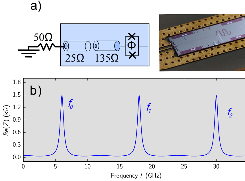
Figure 3.1 Re Z(f) : a) Representation of the device: Two quarter wave resonators in series with characteristics impedance 25\ \Omega and 135\ \Omega , are coupled to an Al/AIO x /Al SQUID with a maximum critical current I_c = 17.5\ \text{nA} . These two transmission lines are designed for a resonance frequency of 6 GHz. b) The real part of the impedance \text{Re } Z(f) seen by the junction, calculated from the resonator geometry. \text{Re } Z(f) shows peaks at f_n = (2n+1)6\ \text{GHz} ; n=0,1,2,\dots
