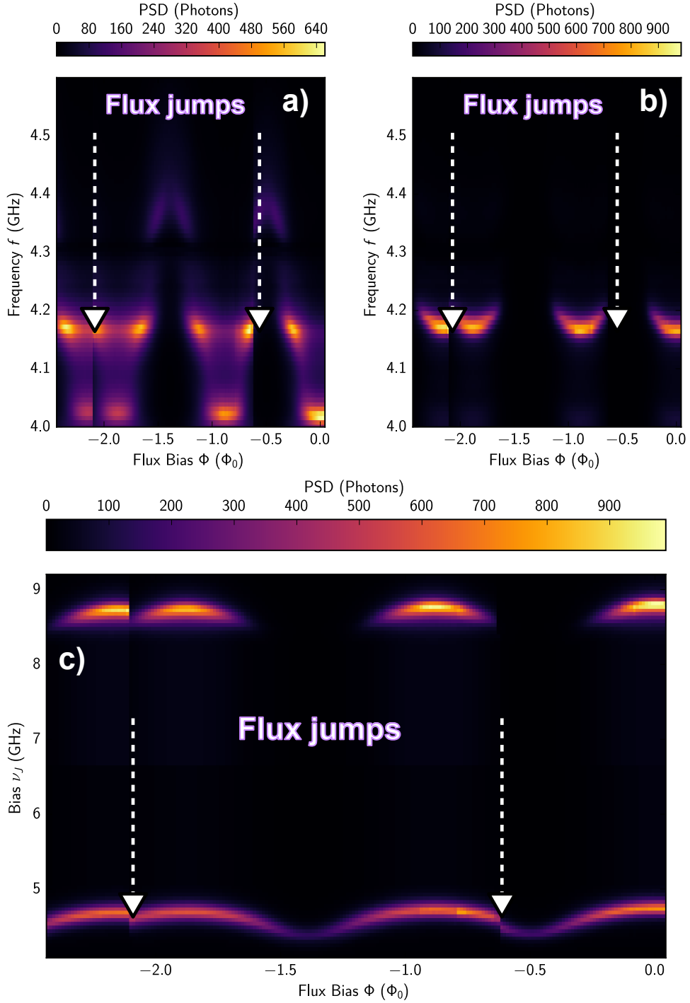
Figure 6.3 Flux modulation The power spectral density as a function of the flux bias \Phi and the frequency f at voltage biases a) \nu_J = 4.58 GHz around one photon process b) \nu_J = 8.2 GHz around two photons process. c) The power spectral density as function of the voltage bias \nu_J and the flux bias \Phi at a frequency f = 4.18 GHz. The dashed white lines show where the flux jumped.
