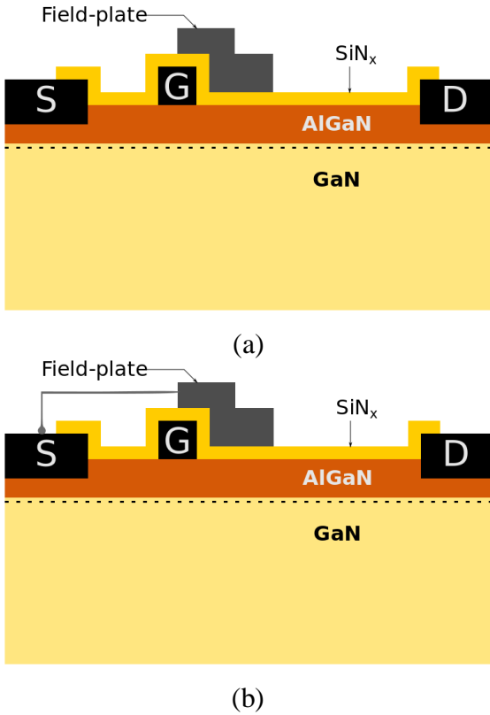
Fig. 1.8. Modified field plate structure of AlGaIn/GaN HEMT device (a) gate connected (b) source connected.
