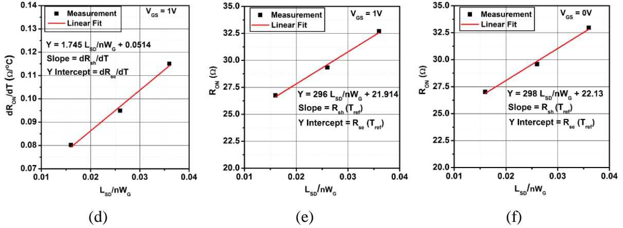
Fig. 4.16. LF S-parameters measurement at T_{ref} = 0^{\circ}\text{C} and V_{GS} = 1\text{ V} : extraction of dR_{ON}/dT [(a), (b) and (c)] for different gate-drain distance, L_{GD} = 1, 2 and 3.0\ \mu\text{m} , respectively, extraction of dR_{sh}/dT (d) and Extraction of R_{sh} and R_{se} : at V_{GS} = 1\text{ V} (e) and 0\text{ V} (f). Device dimensions: W_G = 2 \times 50\ \mu\text{m} , L_G = 0.2\ \mu\text{m} , L_{SG} = 0.4\ \mu\text{m} , and L_{GD} = 2\ \mu\text{m} .
