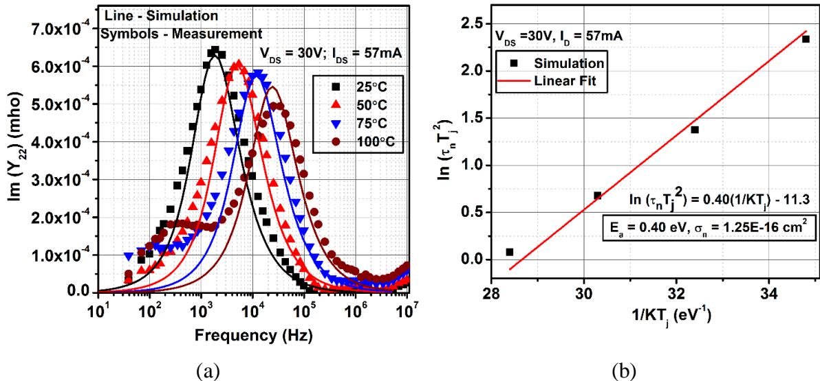
Fig. 3.14. 8 \times 75 \mu\text{m} device: (a) Imaginary part of the simulated (lines) and measured (symbols) Y_{22} -parameter vs. frequency for different T_{chuck} ranging between 25^\circ\text{C} and 100^\circ\text{C} . Bias conditions: V_{DS} = 30 \text{ V} and I_D = 57 \text{ mA} . (b) Extracted Arrhenius plot using the simulated Y_{22} -parameter.
