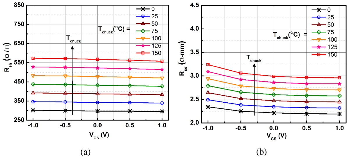
Fig. 4.17. Extracted (a) channel sheet resistance R_{sh} and (b) series contact resistance R_{se} as function of V_{GS} and T_{chuck} using LF measurements. Device dimensions: W_G = 2 \times 50\ \mu\text{m} , L_G = 0.2\ \mu\text{m} , L_{SG} = 0.4\ \mu\text{m} , and L_{GD} = 2\ \mu\text{m} .
