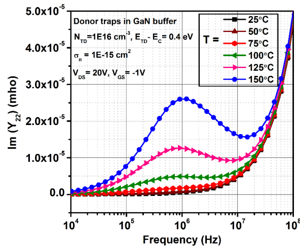
Fig. 3.17. Imaginary part of the simulated 8 \times 75 \mu\text{m} device Y_{22} -parameter vs. frequency for different T_{\text{chuck}} and with donor-like traps in the GaN buffer. Bias conditions: V_{GS} = -1 \text{ V} and V_{DS} = 20 \text{ V} . Donor-like traps in the device cause the peak amplitude increases as the device temperature increases.
