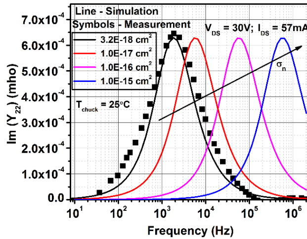
Fig. 3.13. 8 \times 75 \mu\text{m} device: Imaginary part of the simulated (lines) and measured (symbols) Y_{22} -parameter vs. frequency for T_{chuck} = 25^\circ\text{C} and for different electron cross section parameters ( \sigma_n ). Bias conditions: V_{DS} = 30 \text{ V} and I_D = 57 \text{ mA} . Activation energy E_a = 0.4 \text{ eV} , introduced in the simulation.
