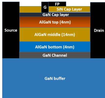
Fig. 3.36. Schematic of the GaN/AlGaIn/GaN HEMT used for transient gate lag simulations.
