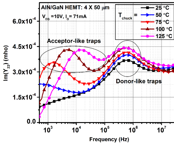
Fig. 3.18. Imaginary part of the measured 4 \times 50 \mu\text{m} AlN/GaN HEMT device Y_{22} -parameter vs. frequency for different T_{\text{chuck}} , illustrating the existence of both acceptor and donor-like traps in the device.
