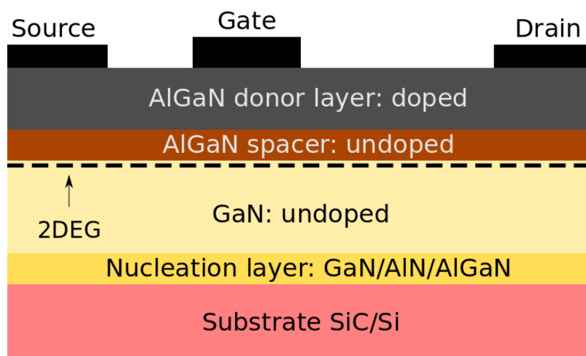
Fig. 1.7. Schematic cross section of conventional AlGaIn/GaN HEMT.
