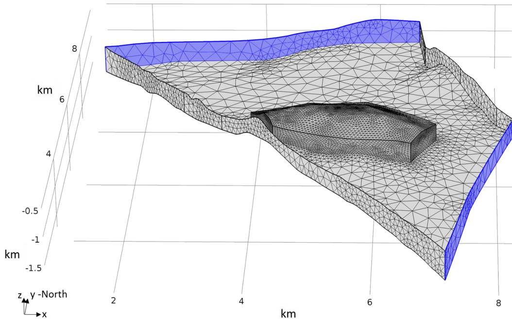
Figure 4-3. Spatial discretization of the modelled 3D structure. A refined tetrahedral grid is used in the axial part of the dome. Results are plotted focusing in this refined area. Blue limits indicate where Dirichlet conditions are imposed.
