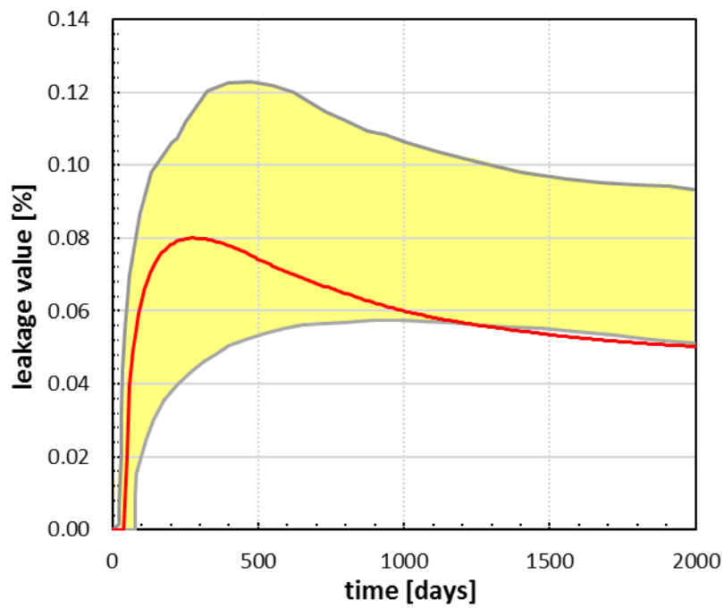
Figure 2-7. Leakage rates through leakage well for problem B. Model result (red) is compared with the values obtained by various models in Class et al. (2009) (yellow area).
