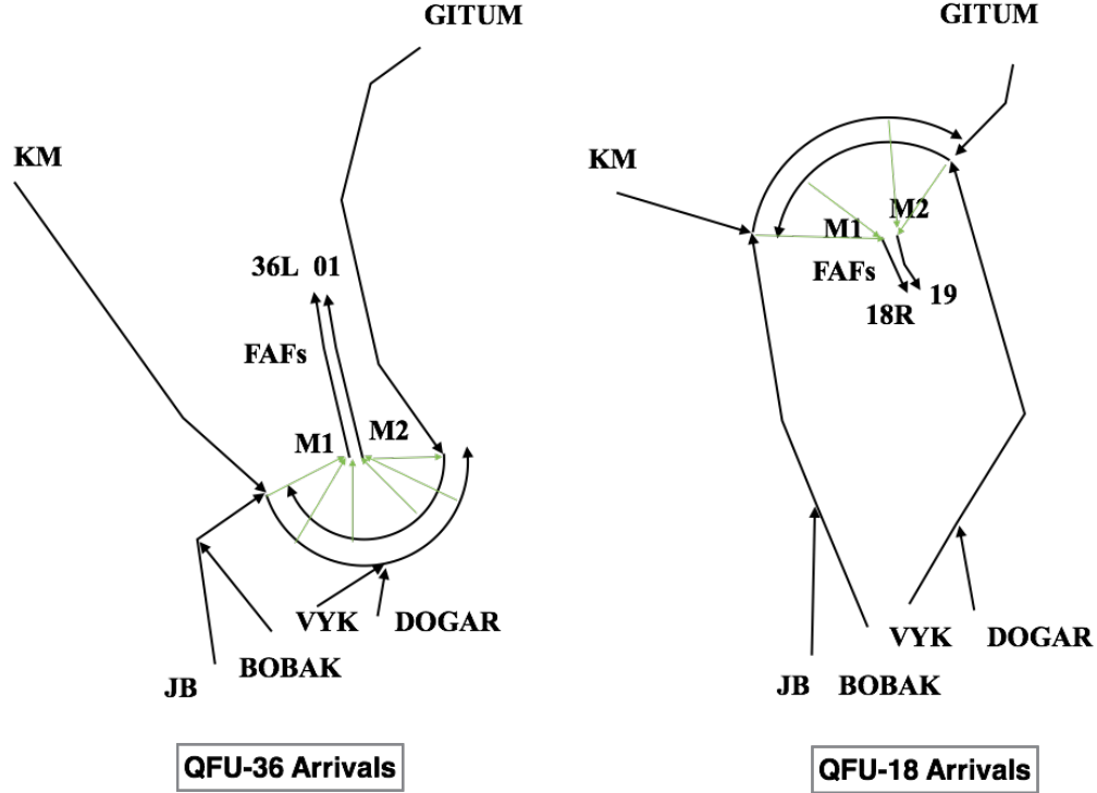
Figure 5.1: ML-PM based STAR design for BCIA
