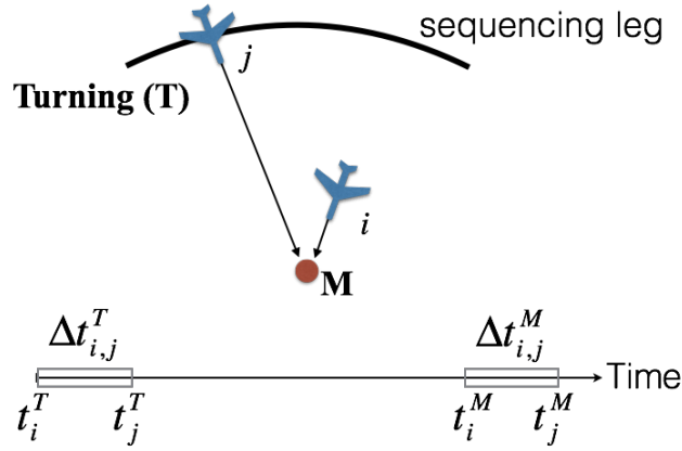
Figure 4.9: Example of conflict detection in merging zone
