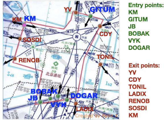
Figure 2.8: TMA of BCIA
