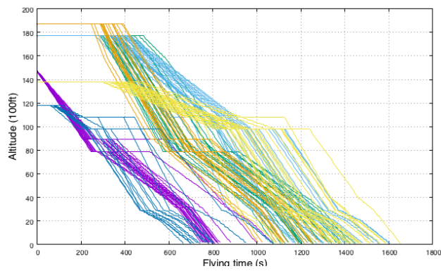
(a) Vertical view of all trajectories
