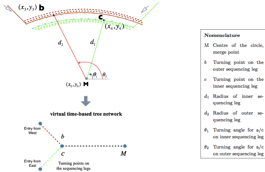
Figure 4.10: Sequencing legs equidistant from single merge point
