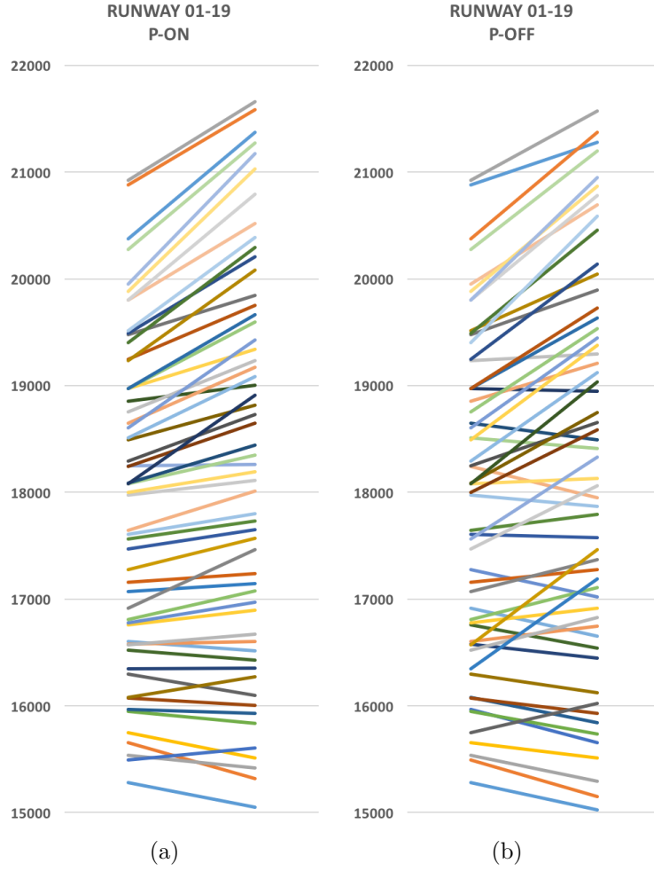
Figure 5.16: Runway 01-19 sequencing with minimizing position shift P ON/OFF
