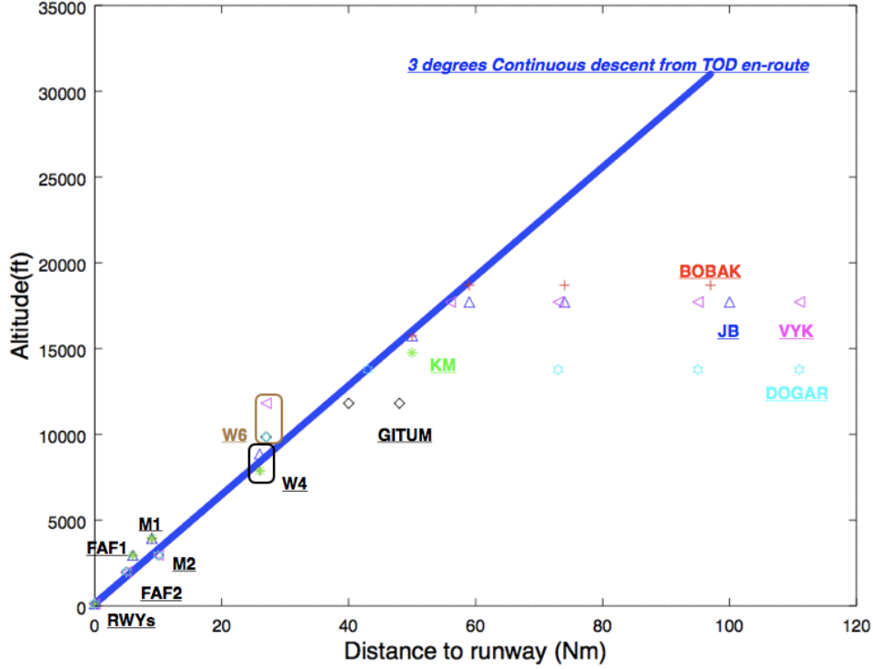
Figure 5.4: Optimized descent profiles and 3° near-CDA descent profile
