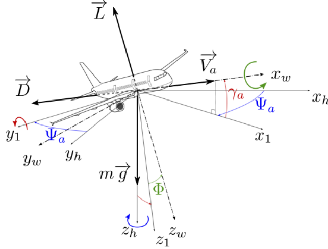
Figure 4.5: Motion of aircraft
