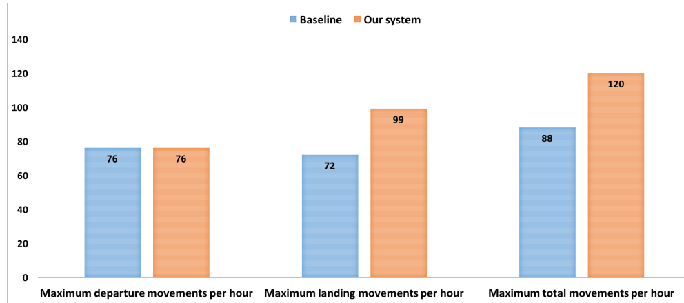
Figure 5.22: Hourly movements comparison between baseline and our system
