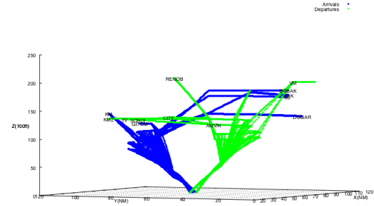
(a) Top view of integrated departures and arrivals (b) Vertical view of integrated departures and arrivals
