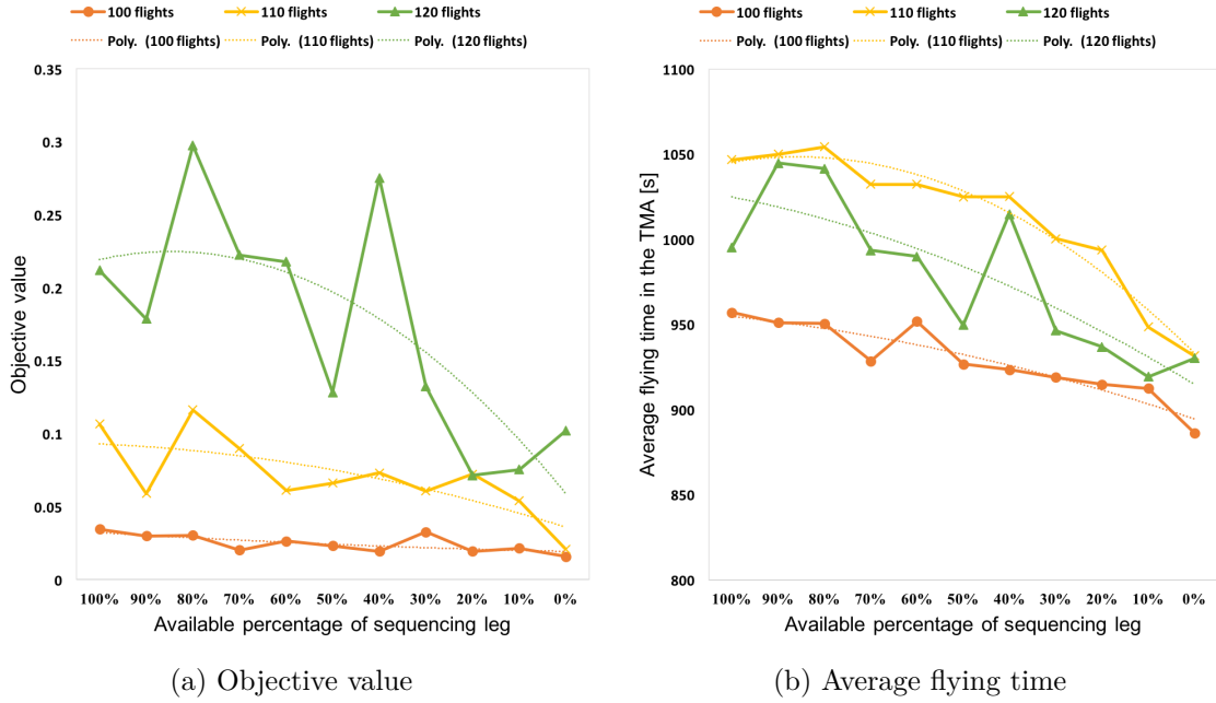
Figure 5.23: Performance with different traffic demand and available sequencing length
