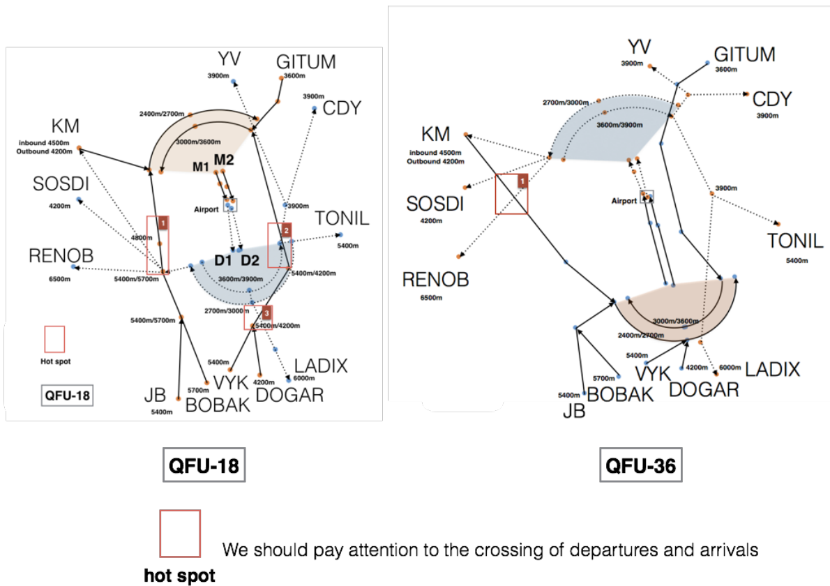
Figure 5.3: STAR and SID design for BCIA
