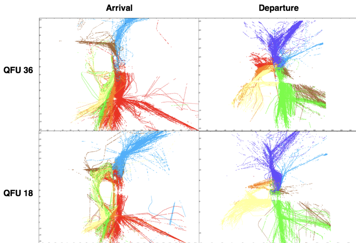
Figure 2.12: Four kinds of traffic pattern with real traffic data
