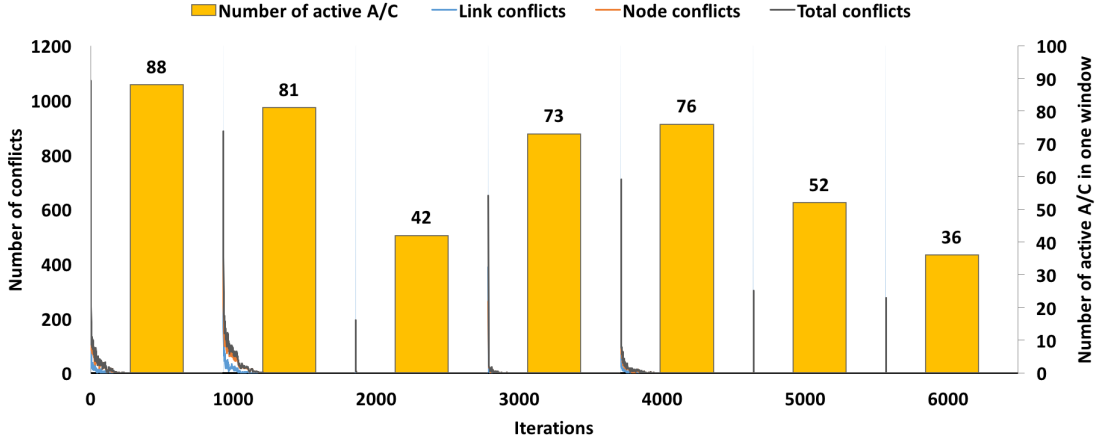
Figure 5.7: De-conflict performance in period (6:00-12:00)
