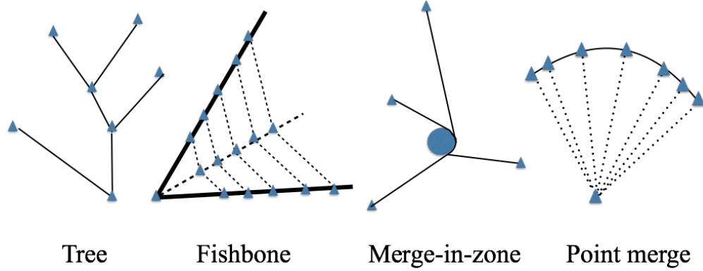
Figure 2.3: Examples of merge topology
