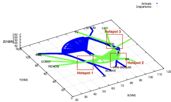
(a) Top view of integrated departures and arrivals (b) Vertical view of integrated departures and arrivals
