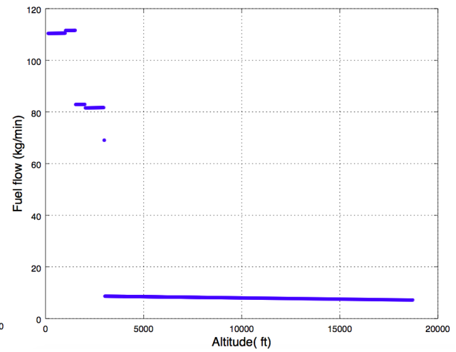
(b) Fuel flow profile
