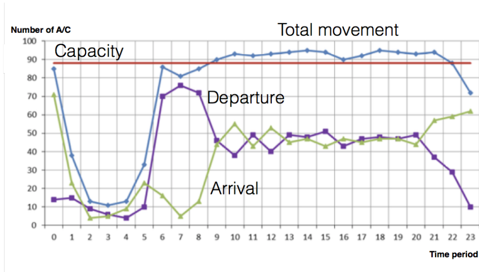
Figure 2.7: Hourly movements at BCIA on 07/09/2015
