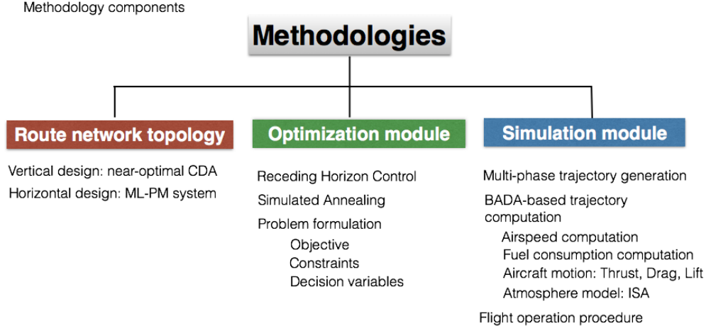
Figure 3.1: Optimization framework
