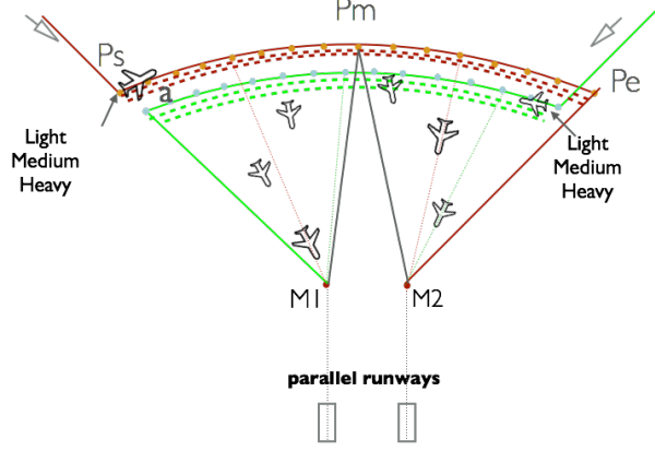
Figure 4.3: Flight procedure in the merging zones for mixed parallel approach
