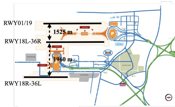
Figure 2.9: Layout of runways at BCIA
