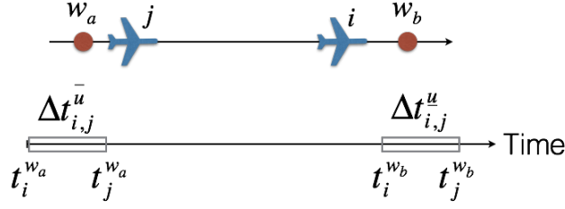
Figure 4.7: Example of link conflict detection
