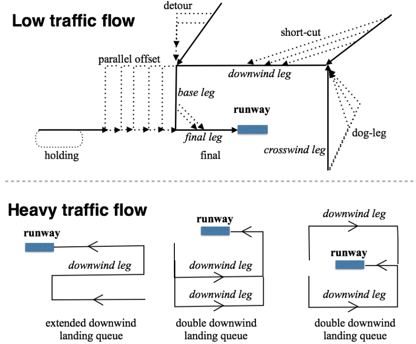
Figure 3.3: Conventional sequencing and merging in TMA
