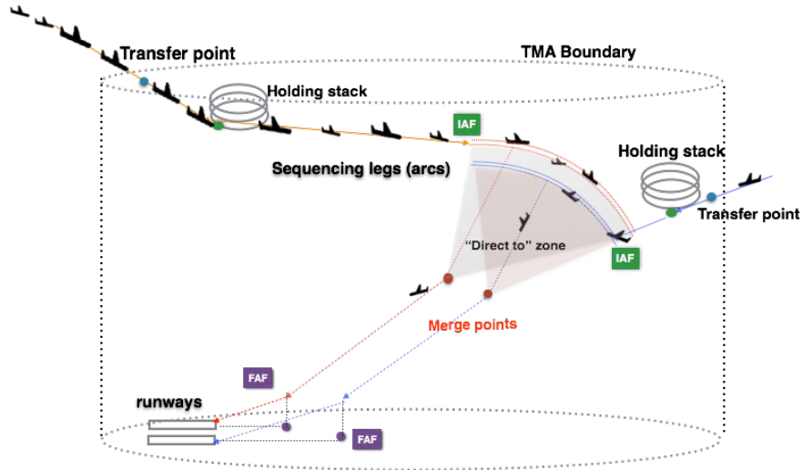
Figure 4.2: An example of ML-PM route network
