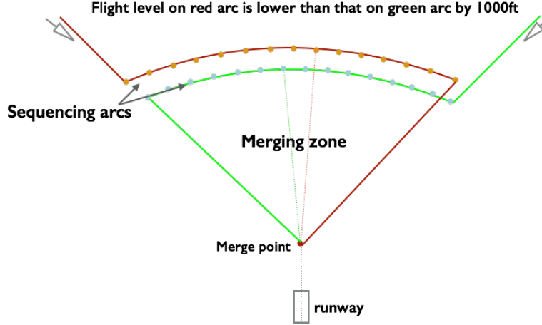
Figure 2.6: Basic PMS topology for single runway
