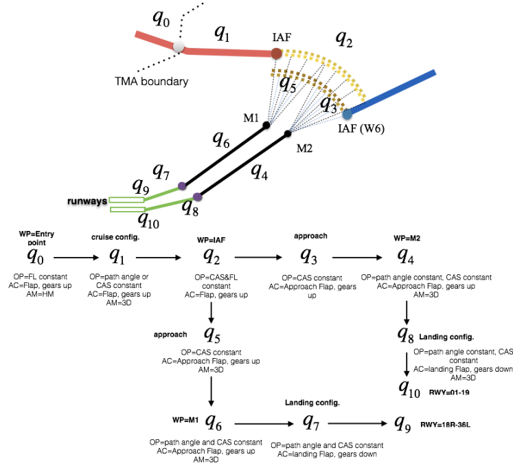
Figure 4.4: Multiphase dynamical control process
