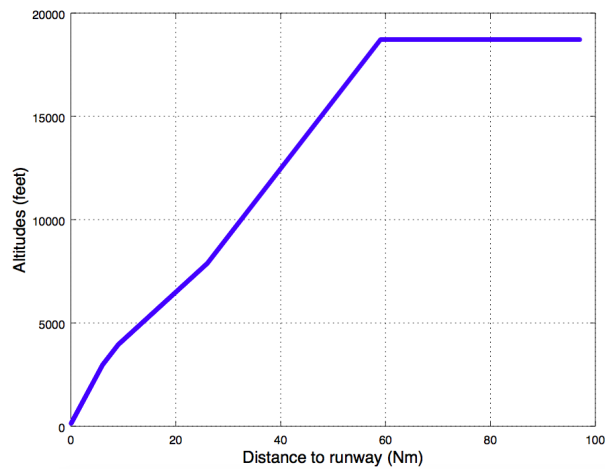
(c) Descent profile
