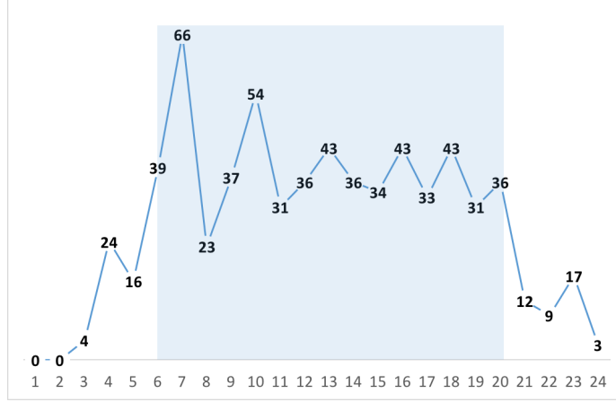
Figure 5.5: Hourly landing demand in Data 1 (Mixed parallel approach)
