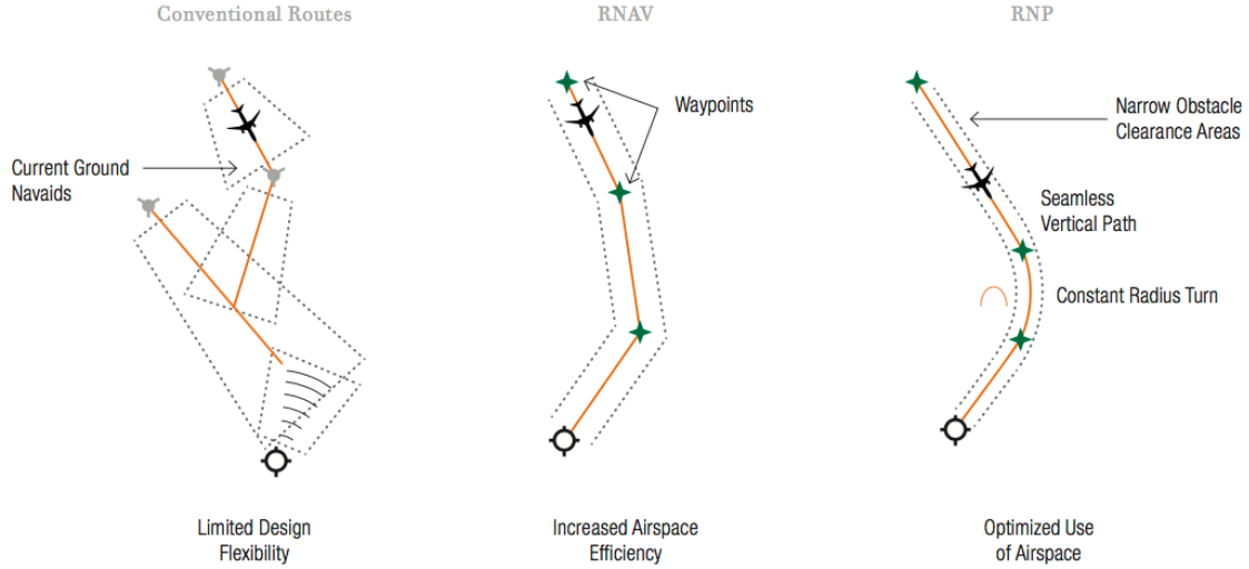
Figure 2.5: Conventional routes compared to PBN-based routes
