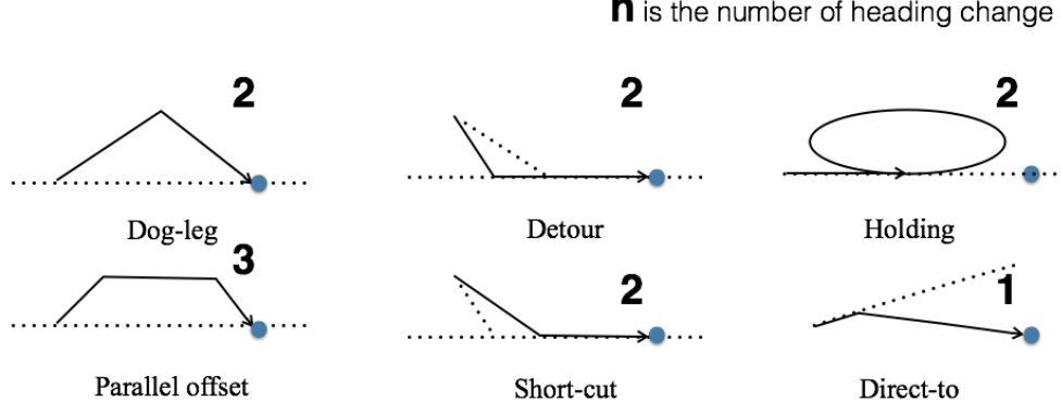
Figure 3.2: Radar vector techniques
