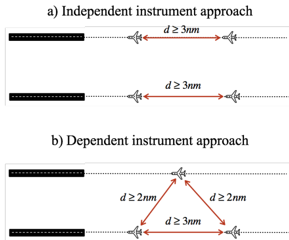
Figure 2.10: Independent and dependent parallel approaches
