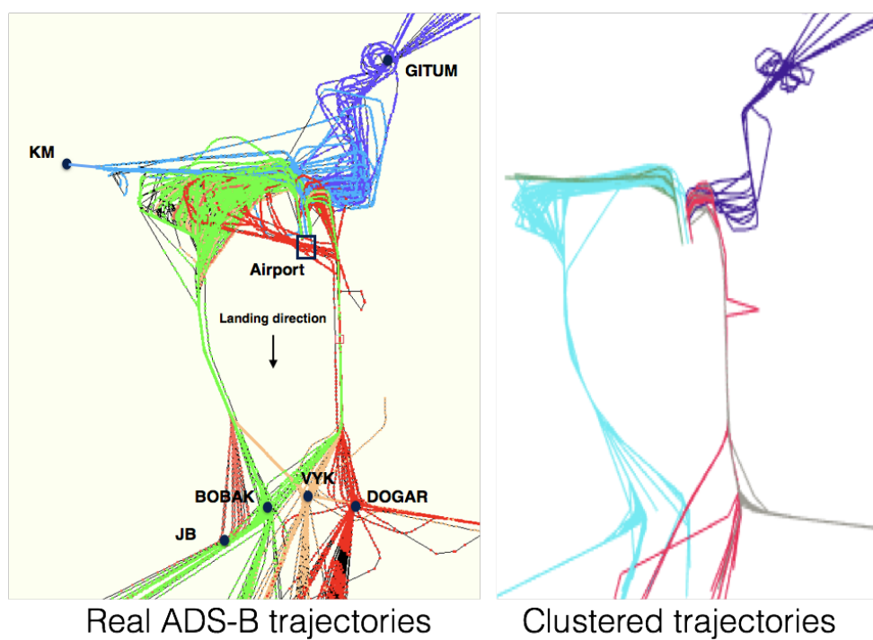
Figure 2.13: South-inbound daily real traffic and clustered traffic
