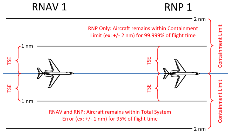
Figure A.2: Difference between RNAV 1 and RNP 1
