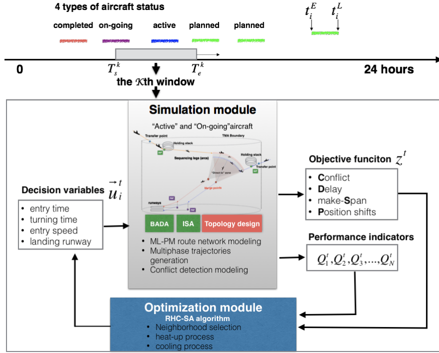
Figure 4.1: Relationship between simulation module and optimization module
