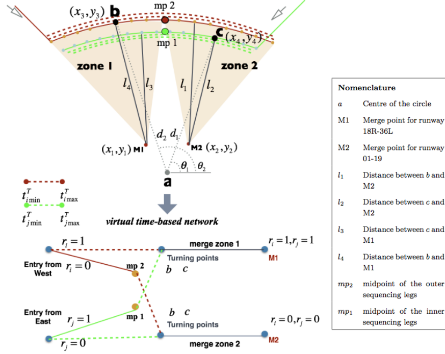
Figure 4.11: Merge conflict detection in mixed parallel approach
