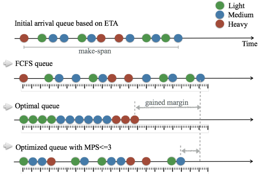
Figure 2.1: A centralized approach: sequencing problem with different solutions
