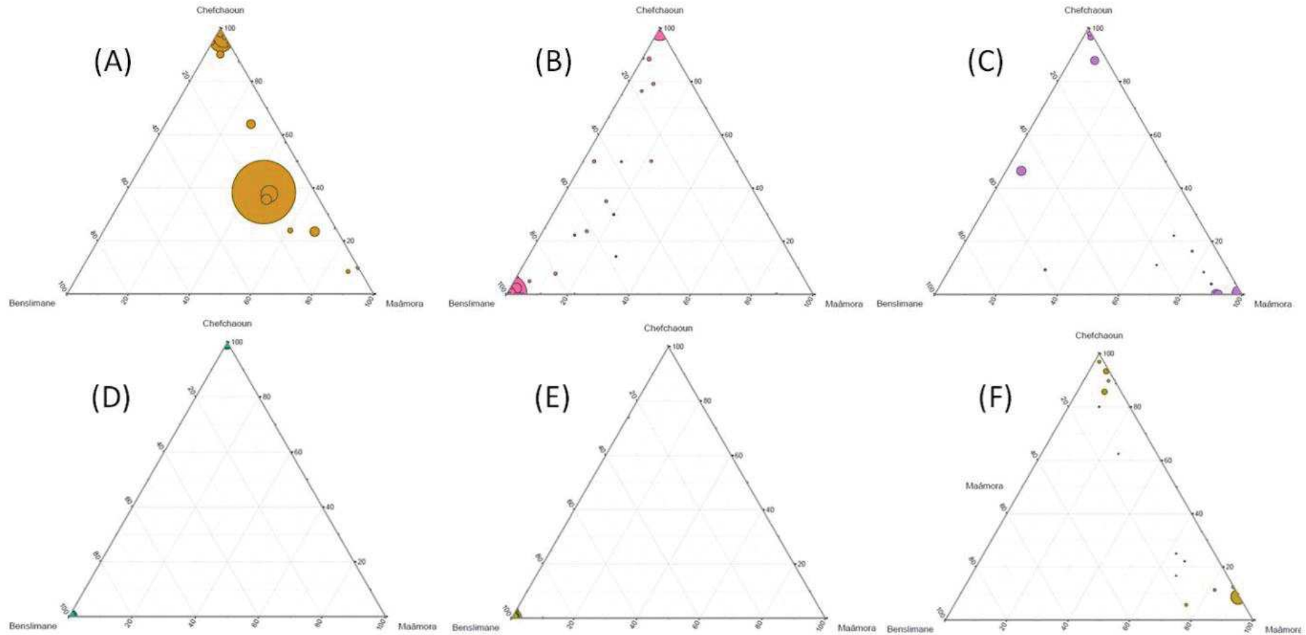
Figure II.3. Distribution of fungal OTUs among habitats (Maãmora, Benslimane, Chefchaoun) at genus level in ternary plots. The six predominant genera are indicated, (A) Cenococcum (45 OTUs, 12,516 sequences), (B) Tomentella (140 OTUs, 11605 sequences), (C) Russula (64 OTUs, 7,027 sequences), (D) Inocybe (19 OTUs, 4734 sequences), (E) Cortinarius (39 OTUs, 4,569 sequences), (F) Cladophialophora (85 OTUs, 3,042 sequences). The size of a dot represents the abundance of one OTU.
