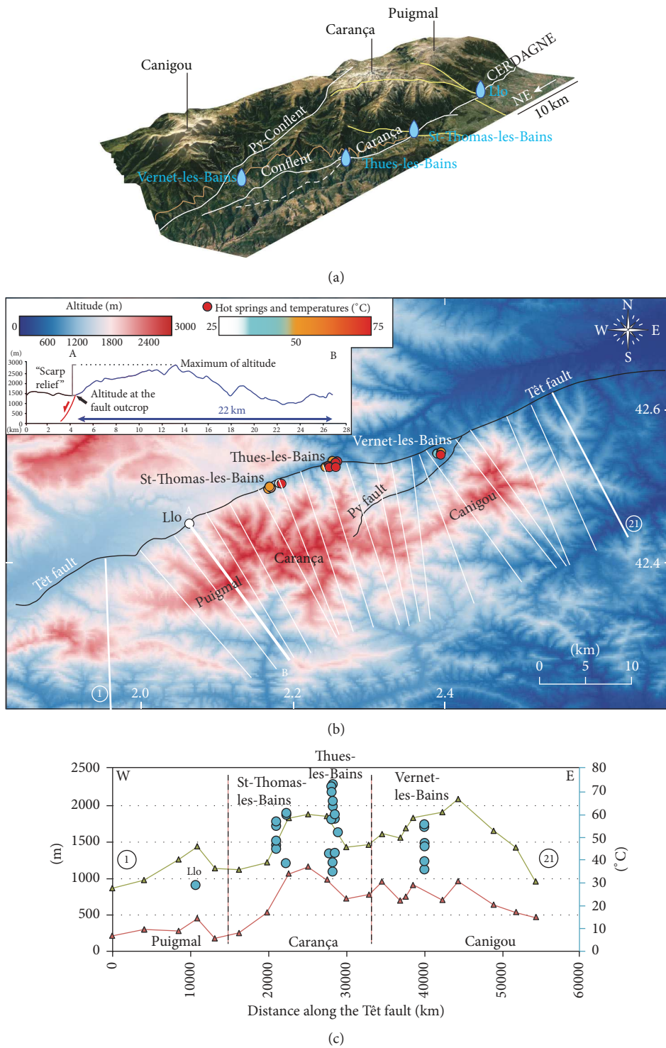
FIGURE 6: Relation between hot springs, the Têt fault segmentation, and relief. (a) Location of the main mountain ranges associated with the Têt fault segmentation (white line) and subsidiary faults (yellow line). Principal hot spring sites are indicated. (b) Altitude map including the principal ranges, the Têt and Py faults (black lines), and hot springs with temperatures (colored circles). Springs are at the bottom of high reliefs. The Carança and Puigmal Ranges, concentrating most of the hot springs with the highest temperatures, form a wide area of elevated altitudes compared with the Canigou Range. Numbered profiles used for measurements in (c) are indicated (white lines). (c) Graph along the Têt fault (E-W) of hot spring temperatures (blue circle, right axis), scarp relief (green curve, left axis), and average of normalized altitudes integrated to the range wide (red curve, left axis), calculated from topographic profile (e.g., the A-B cross-section indicated as bold white line in (b)). Profile 1 and profile 21, identified in (b), mark, respectively, the origin and the end of x-axis in (c). The highest number of springs and temperature maxima correspond to the largest scarp relief and average of altitudes.
