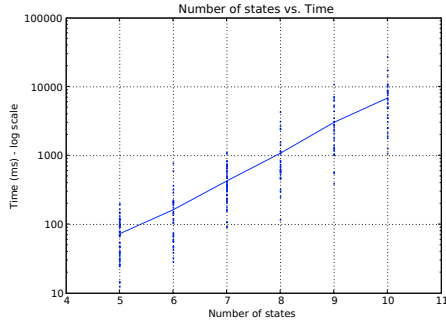
FIGURE 5.2: Scaling of ICG algorithm, number of states vs time [Regan and Boutilier, 2008]
