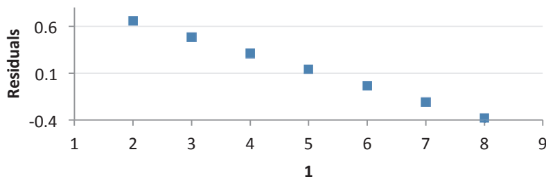
Residuals vs 1
