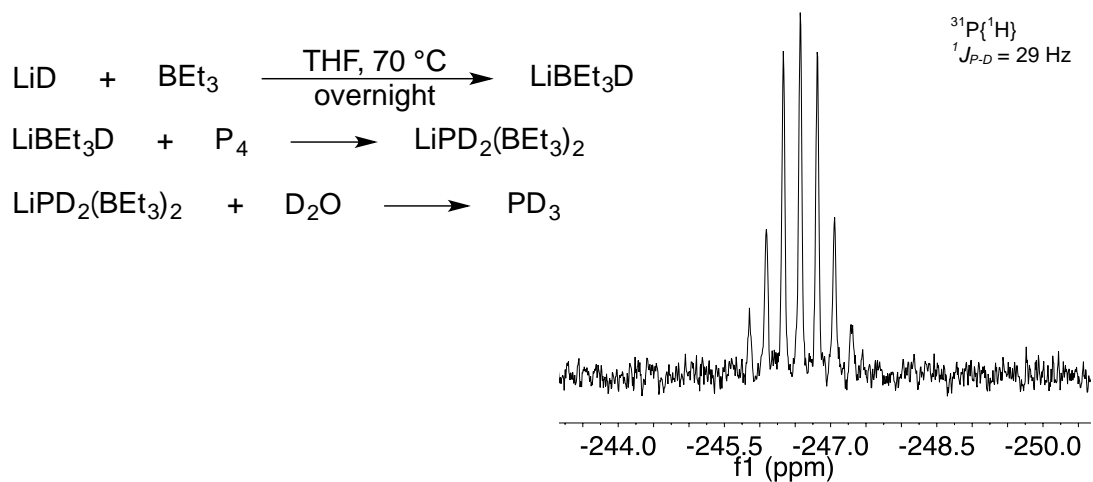
Figure V-5. Reaction of \text{LiPD}_2(\text{BEt}_3)_2 with \text{D}_2\text{O} , producing \text{PD}_3 .
