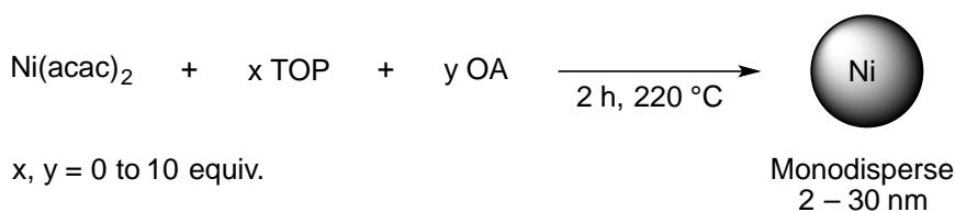
Figure I-7. Ni(0) nanoparticles from the high-temperature reduction of \text{Ni}(\text{acac})_2 by oleylamine in the presence of TOP.
