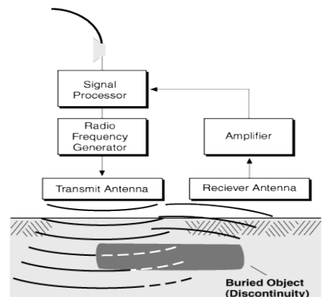
Figure 5: GPR principle
