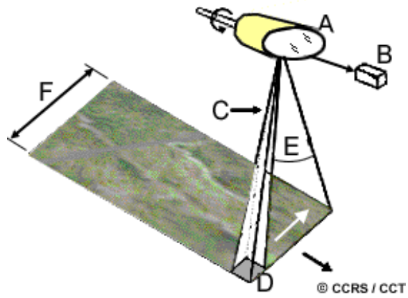
Figure 8: Wiskbroom scanning principle [132]
