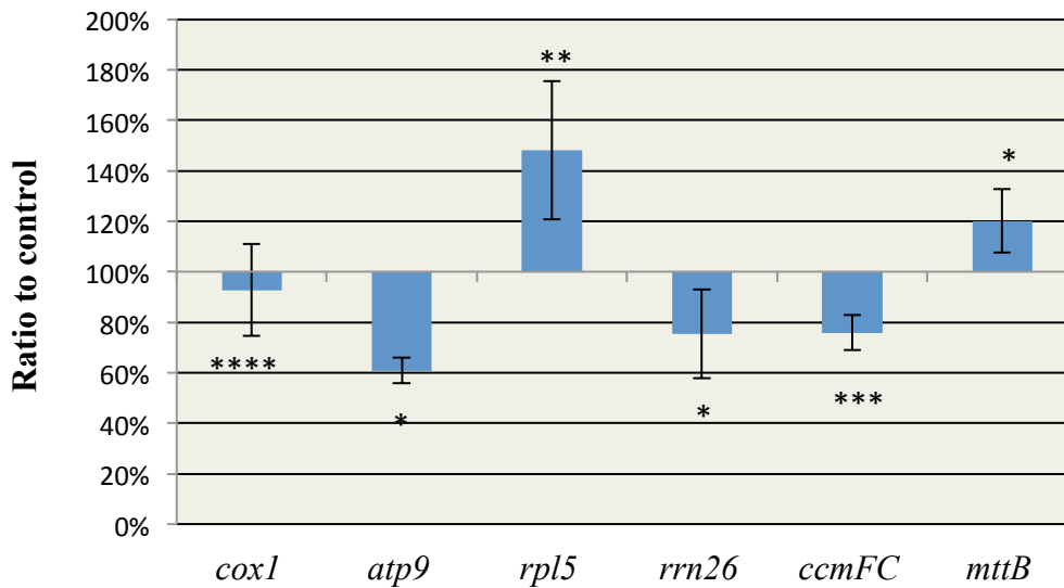
Figure 16: Effect of orf77 -PKTLS RNA expression at the mature stage of development on the level of selected mitochondrial RNAs. Analysis by RT-qPCR on total RNA. A) Results are given as the percentage of the selected mitochondrial RNAs at D3 as compared to control. B) Results are given as the percentage of the selected mitochondrial RNAs at D4 as compared to control. *= P \leq 0.05 , **= P \leq 0.01 , ***= P \leq 0.001 , ****= P \leq 0.0001 .
