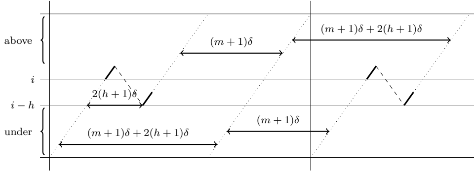
Figure 4.7: One wave
