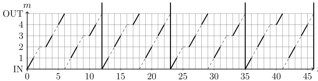
Figure 2.9: Two periods (four iterations) of \pi_{oe} operating in periodic steady state on instance J : ( m = 4 , p = 6 , \delta = 1 )
