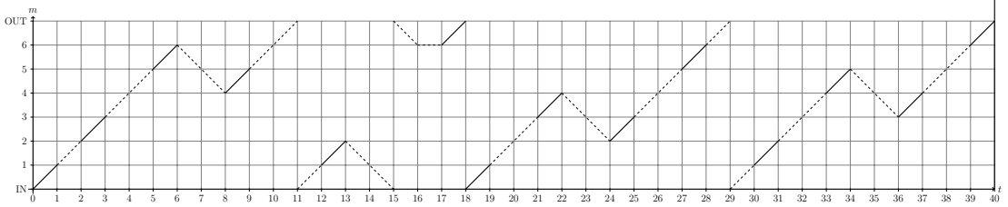
Figure 3.5: An iteration of C , for p = 11 and \delta = 1
