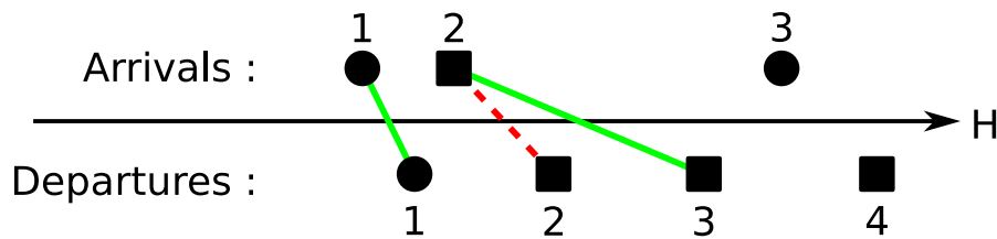
Figure 5.8: Greedy Algorithm : example
