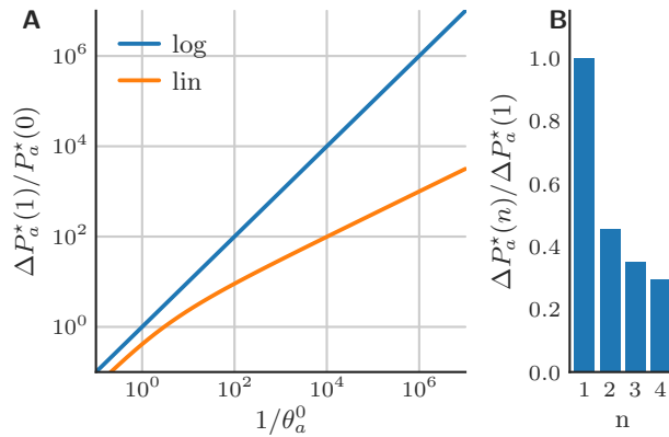
Figure 5.5: Optimal amount of memory production. (A) Change in protection \Delta P_a^*(1) upon first pathogen encounter relative to prior protection for linear and logarithmic cost functions as a function of pathogen variability. (B) Change in protection \Delta P_a^*(n) relative to change for first encounter \Delta P_a^*(1) for linear cost function in the quasistatic limit.
