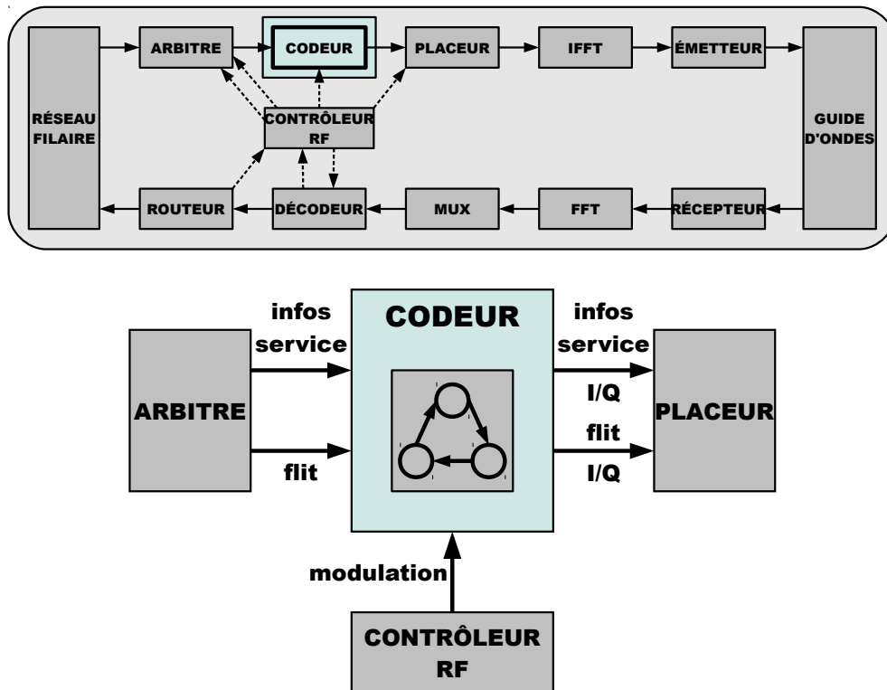
Figure 4.4 – Codeur
