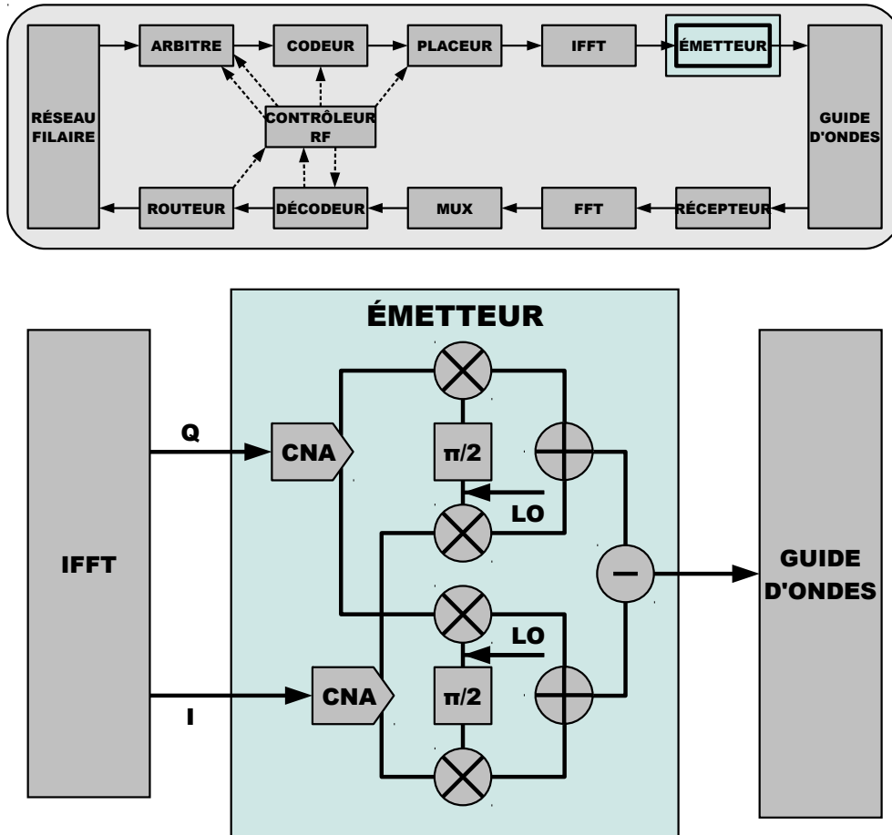
Figure 4.7 – Bloc de transmission RF
