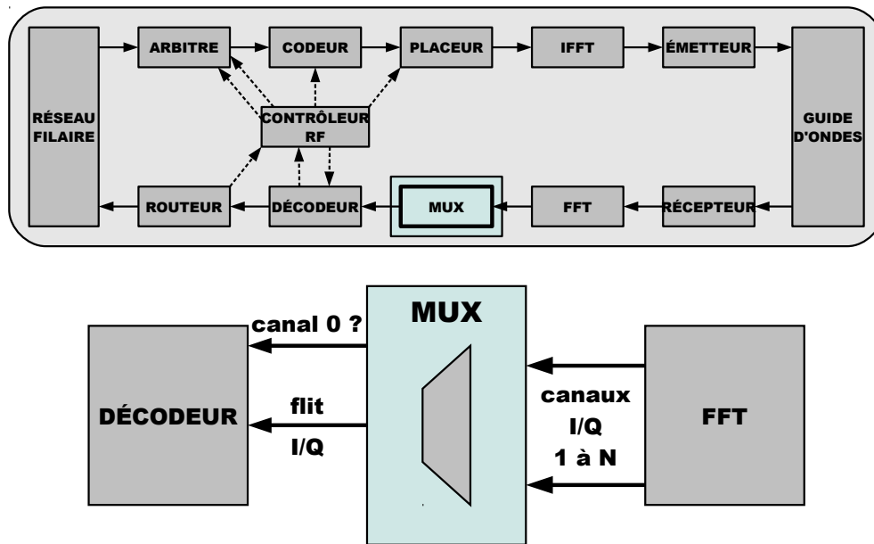
Figure 4.11 – Multiplexeur
