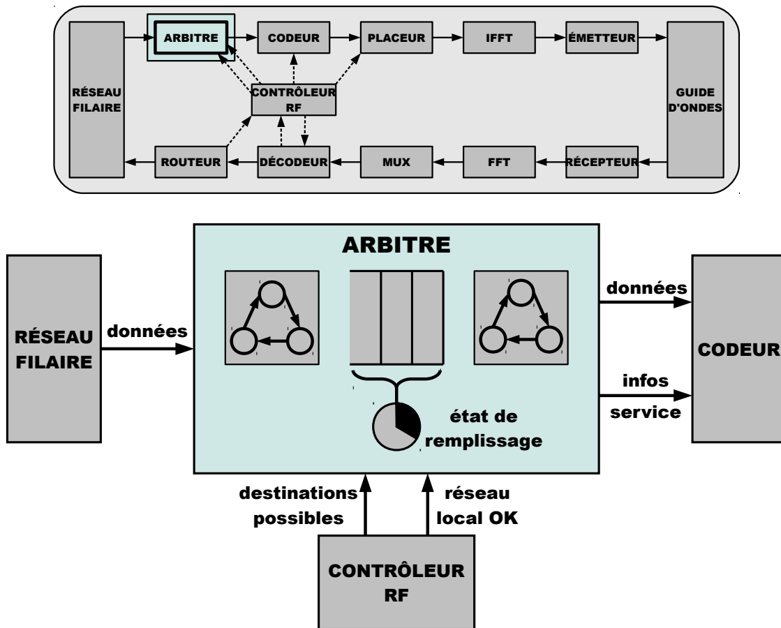
Figure 4.3 – Arbitre
