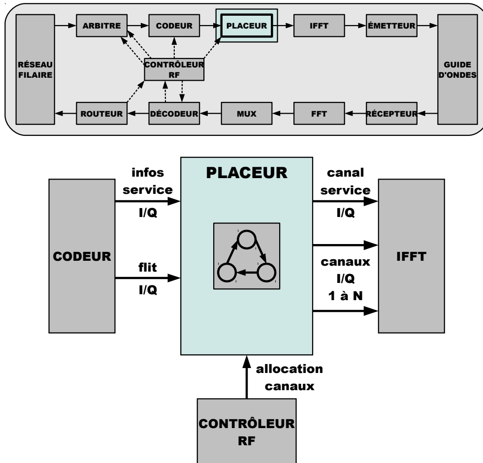
Figure 4.5 – Placeur
