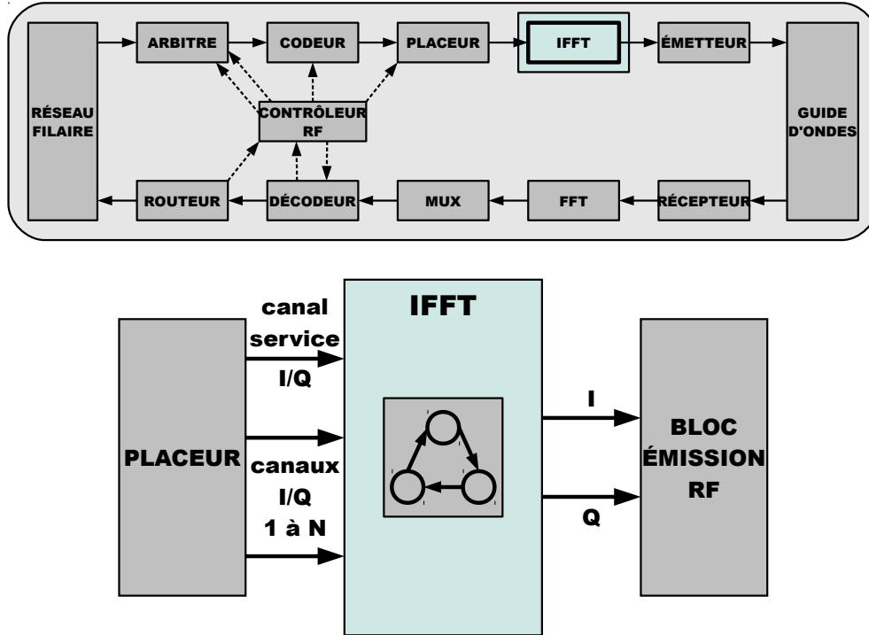
Figure 4.6 – IFFT
