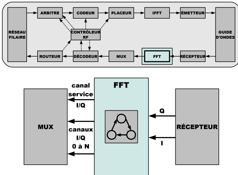
Figure 4.10 – FFT
