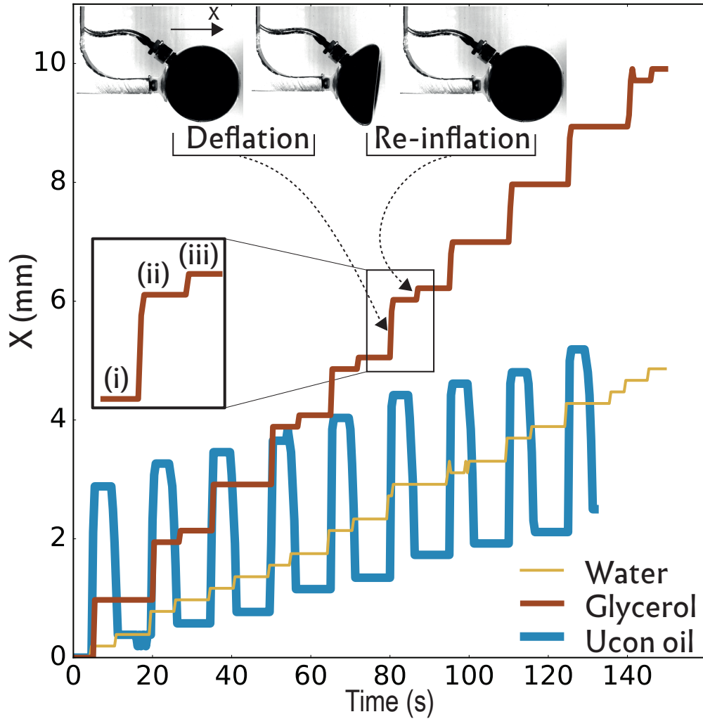
Figure 5.1: Displacement as a function of time of a shell with relative thickness d/R=0.22 in three liquids of different viscosities. Water ( \eta = 10^{-3} Pa.s), Glycerol ( \eta = 0.9 Pa.s), Ucon© oil ( \eta = 37 Pa.s). Pressure cycles of amplitude -600 to 0 mbar and period 15 s are applied. The zoomed region will be used later to explain the calculation of the displacement.
