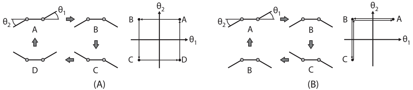
Figure 1.2: Theoretical three-link swimmer. Left sequence (A) represents a non-reciprocal series of angles, the right sequence represents a reciprocal series of angles. Image from [Peyer et al., 2012].
