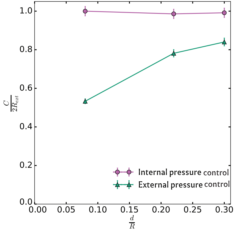
Figure 3.4: Evolution of the concavity size as a function of (\frac{d}{R}) when controlling pressure externally and internally. For internal pressure control, measurements performed by manual image treatment.
