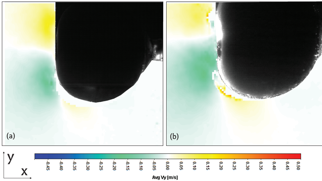
Figure 4.15: Time-averaged y-component of velocity during unbuckling phase: (a) in water;(b) in glycerol. Averaging done over a duration of \approx 15 ms. (d/R)=0.22 shell.
