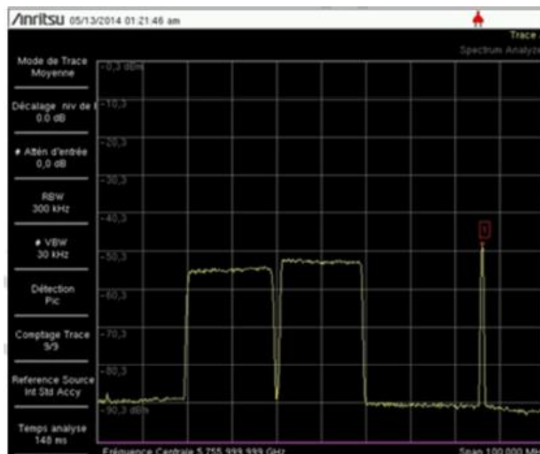
Figure II-22 : Spectrum of the wireless fronthaul signal at 5.75 GHz
