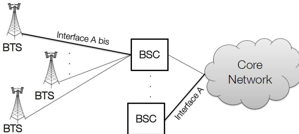
Figure I-2 : GSM architecture [5]
