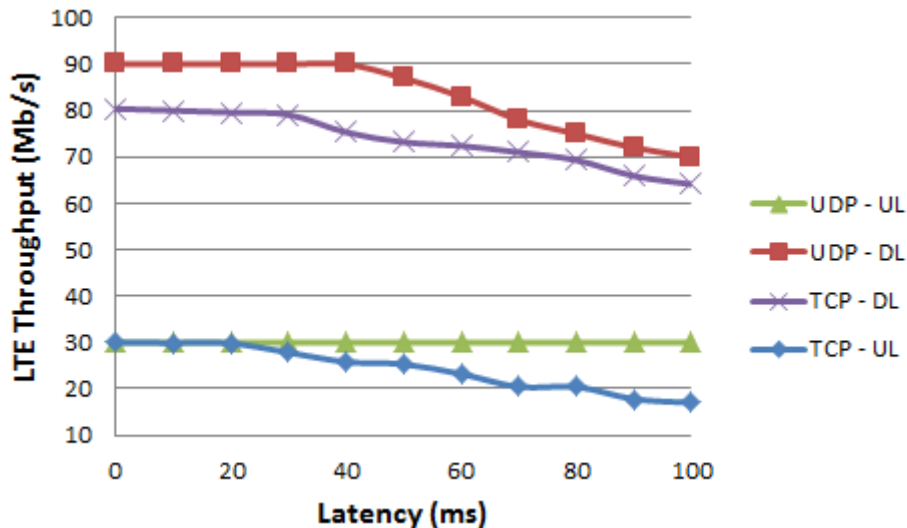
Figure V-11 : Latency (ms) vs LTE Throughput (Mbit/s)
