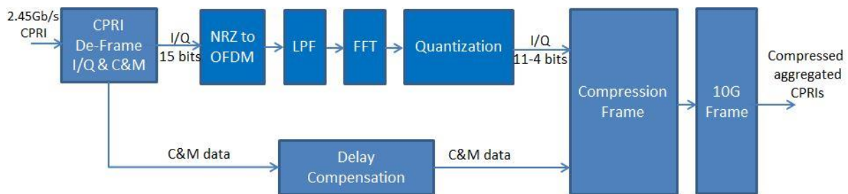
Figure IV-11 : Compression algorithm
