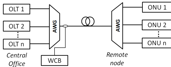
Figure II-8 : WDM-PON system architecture
