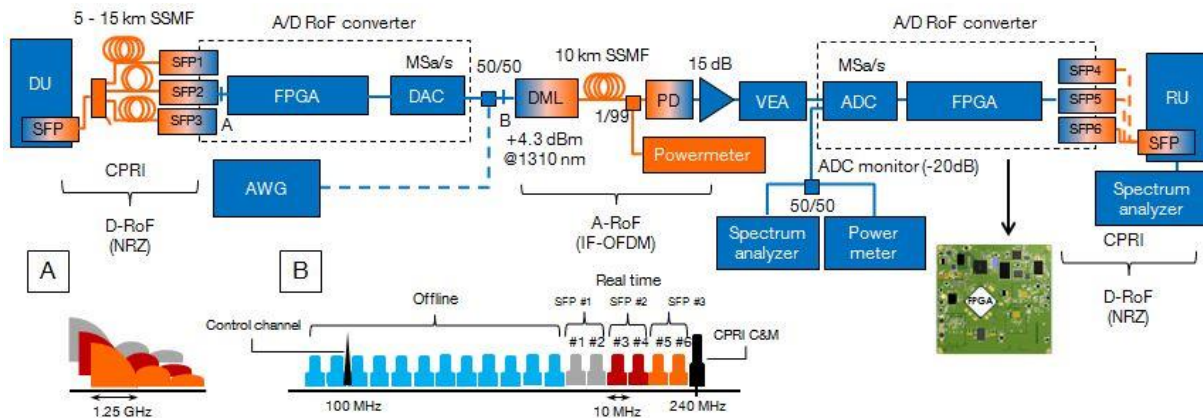
Figure III-3 : A-RoF/D-RoF experimental setup
