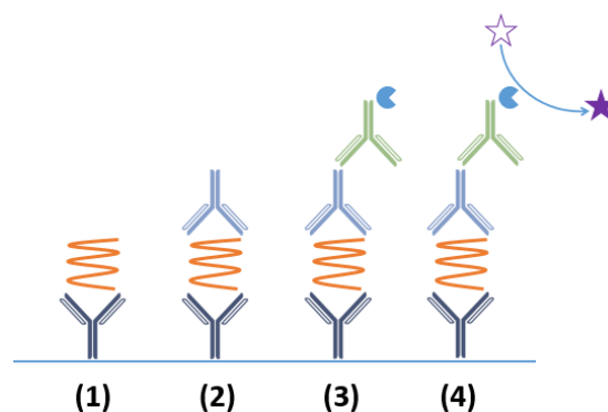
Figure 3.2. Sandwich ELISA.
