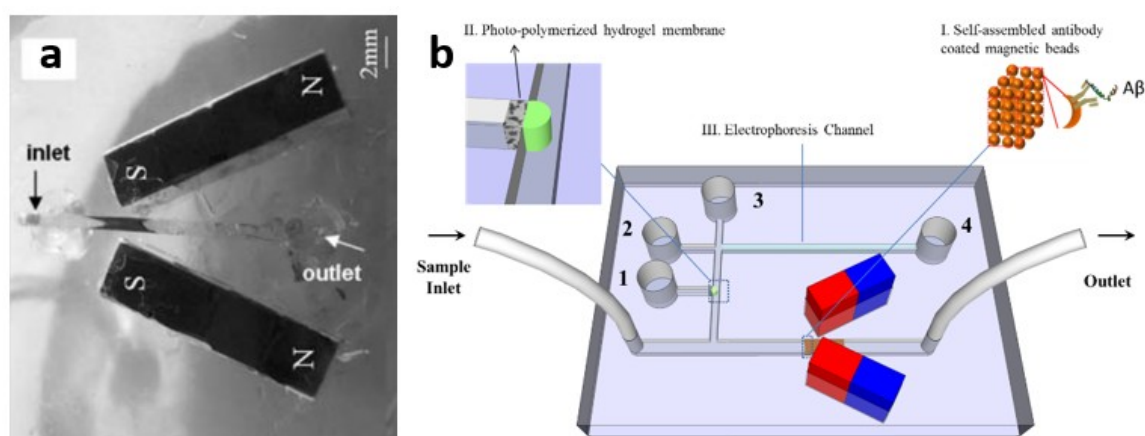
Figure 3.3. (a) Magnetic plug obtained by the injection of magnetic beads in a channel with two neodymium magnets placed on either side. (b) Integration of this system in a lab-on-chip platform for \text{A}\beta preconcentration and electrophoretic separation.
