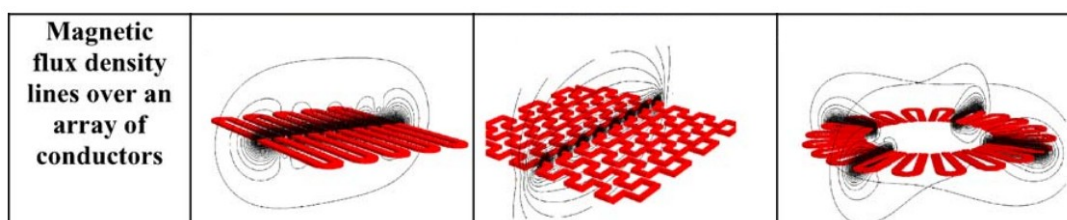
Figure 1.18. Magnetic flux density lines for micro-electromagnets of complex geometries (section 10 \times 2 \mu\text{m} ) (Ramadan et al. 2004).
