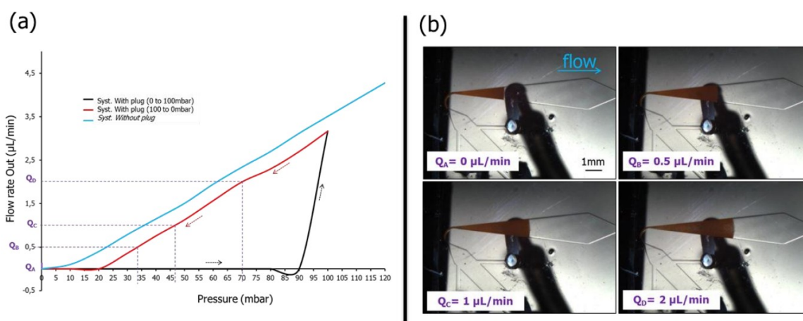
Figure 1.27. (a) Variation of the flow rate versus pressure for a fluidized bed formed by 50 \mu\text{g} of 2.8 \mu\text{m} magnetic particles and (b) pictures of the fluidized bed at different flow rates (Tabnaoui 2012).
