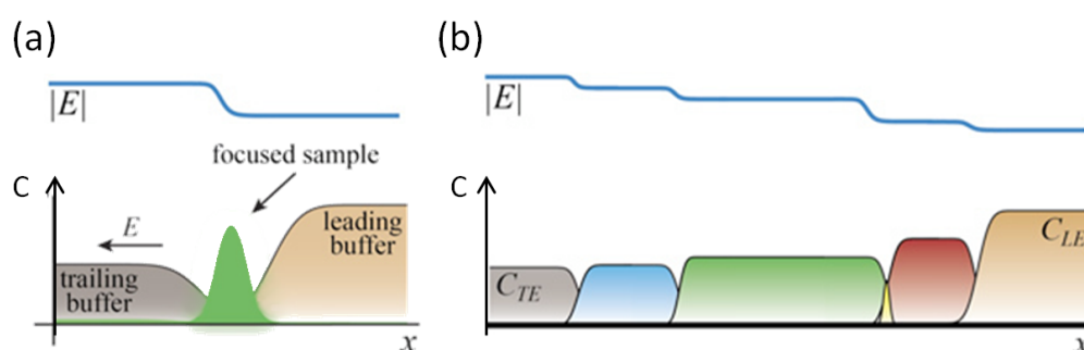
Figure 1.9. Principle of isotachophoresis, (a) the sample is focused in a peak when its concentration is not high enough to influence the local electric field, while (b) bands of different ion mobility form for higher concentrations, adapted from (Garcia-Schwarz et al. 2012).
