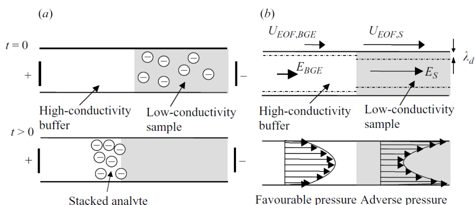
Figure 1.7. (a) Scheme showing FASS of ionic species in the idealised of a total absence of flow and (b) the more realistic case where the electric field results in an additional EOF generating a pressure gradient and lowering the efficiency of stacking. Adapted from (Bharadwaj & Santiago 2005)
