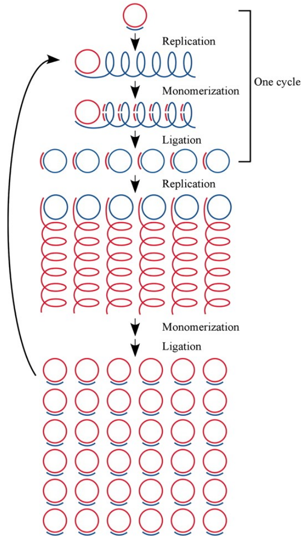
Figure 5.2. The C2CA mechanism. (Dahl et al. 2004)
