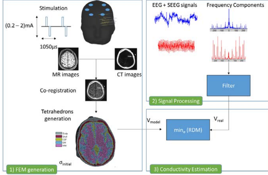
Figure 5.5: A scheme showing the procedure for estimating the conductivities in Patient(1) by considering the fundamental frequency (55 Hz) and the first two harmonics (110 and 165 Hz).
