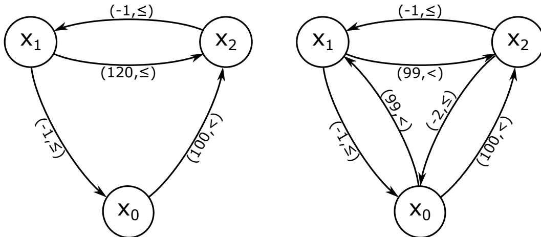
Figure 4 – Directed graph representation of D (left) and its canonical form (right).
