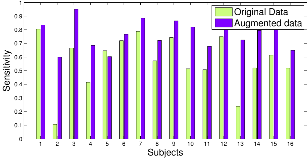
Figure 6.5: Classification performance in terms of sensitivity. For each of the 16 subjects these measures are given for classification based on training on original unbalance training set and training on augmented and balanced training set.
