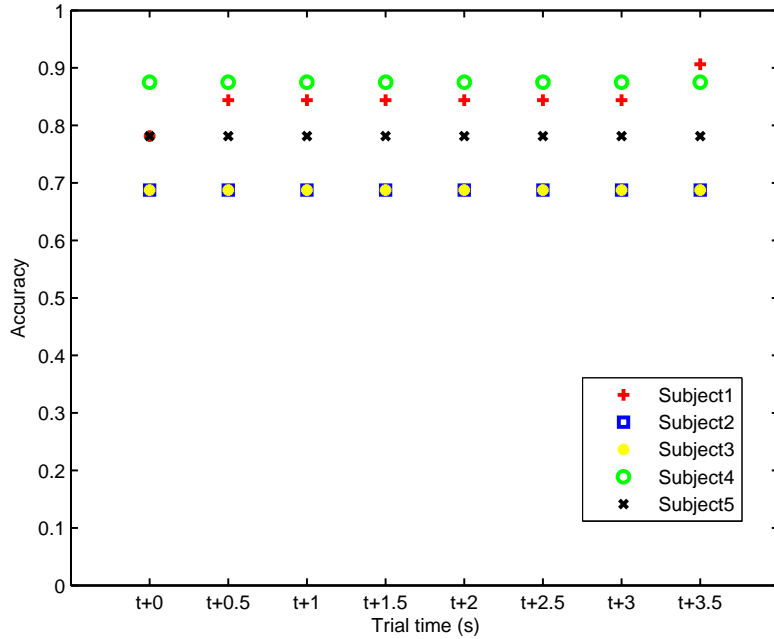
Figure 4.6: Assessment of the accuracy of classification depending on the time of the prediction. On x-axis, t+0 indicates the first prediction made three seconds after the start of a trial. The results are averaged on all trials for each subject. Subject 1 is the only one to present a slight increase of the classification accuracy. For all other subjects, the algorithm proposes a correct answer as the first prediction.
