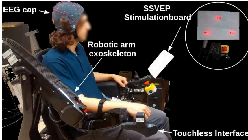
Figure 4.4: Experimental setting: subject sitting on an electric wheelchair equipped with a robotic arm exoskeleton. During offline recordings, the exoskeleton and the touchless interface are disabled; the subject performs the SSVEP task as prompted by audio cues.
