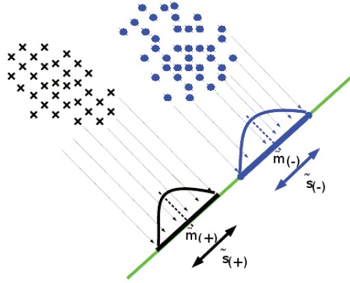
Figure 3.4: LDA mapping. The distance |\tilde{\mathbf{m}}_{(+)} - \tilde{\mathbf{m}}_{(-)}| is maximised relative to class variance such as the separability is maximised ( J(\mathbf{w}) )
