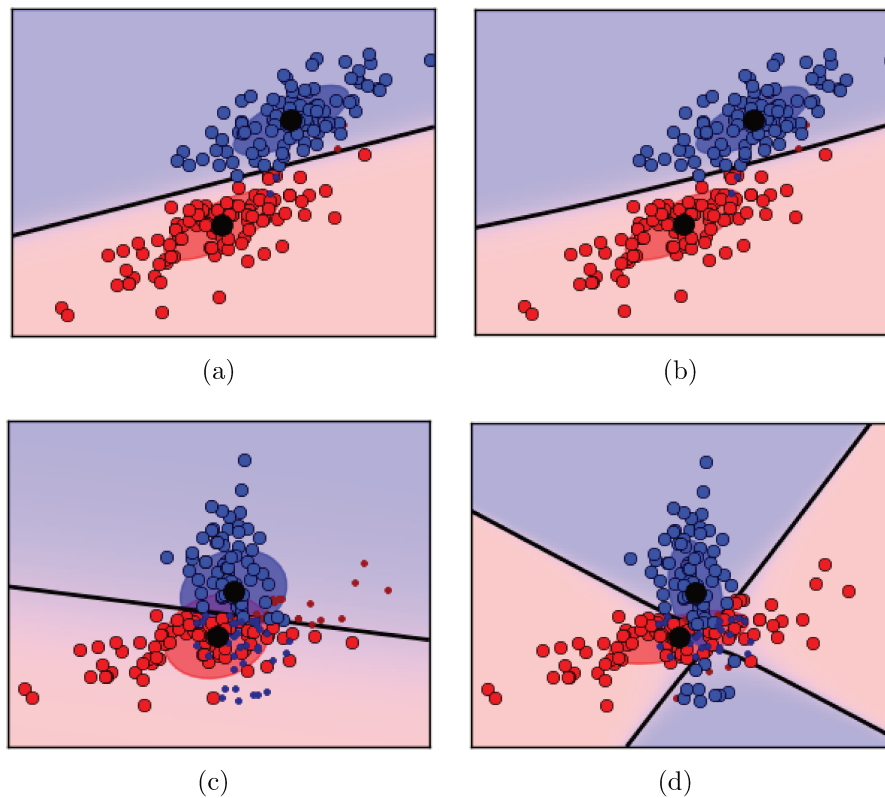
Figure 3.5: QDA versus LDA. Data from two subsets shows with red and blue circles are classified with either LDA (in (a) and (c)) or QDA (in (b) and (d)). The black lines show the classifier separation line. Wrongly classified data are shown with squares instead of circles. Class covariances are shown with ellipses of corresponding colours. In (a) and (b), the two subsets have similar covariance, while in (c) and (d) they have different covariance [Pedregosa et al., 2011]
