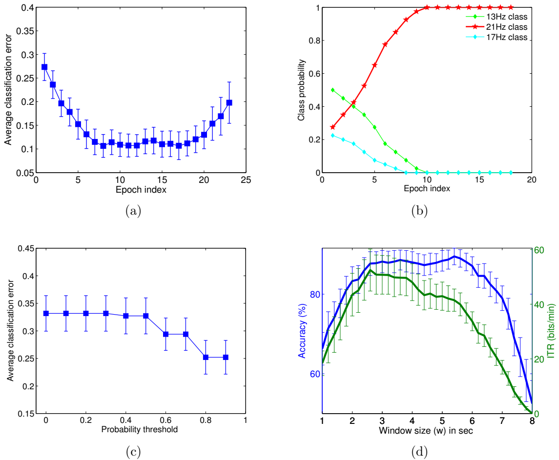
Figure 5.8: Evaluation of the online algorithm parameters. 5.8(a) shows the decrease of the average classification error over all subjects during the successive epochs after the beginning of the trial. 5.8(b) is an example taken from the subject with the best performance showing how the probability of the actual class varies with epoch position from beginning of trial. The groundtruth class probability is represented with a thick-and-star line, while other classes probability lines are thin-and-diamond. 5.8(c) shows the variation of the average classification error for different probability threshold ( 0 \leq \vartheta < 1 ) and its influence on the classifier output (Algorithm 3 step 6). 5.8(d) shows how the average online performance varies with respect to the epoch size ( w ). It shows both the classification accuracy (left y-axis) and the ITR (right y-axis). In 5.8(a), 5.8(c), and 5.8(d), the bars represent the error of the mean i.e. standard deviation divided by the square root of n - 1 , n = number of samples.
