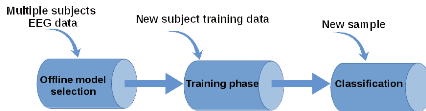
Figure 3.8: Adopted machine learning pipeline. It consists of 3 main phases: 1) Offline model selection: A number of preprocessing and classifiers are tested on a collection of data from multiple subjects, the best combination is selected. 2) Training phase: Classifier parameters are trained for each new subject before classification. 3) Classification: A new [unseen] sample is preprocessed similarly to training data, then classified.
