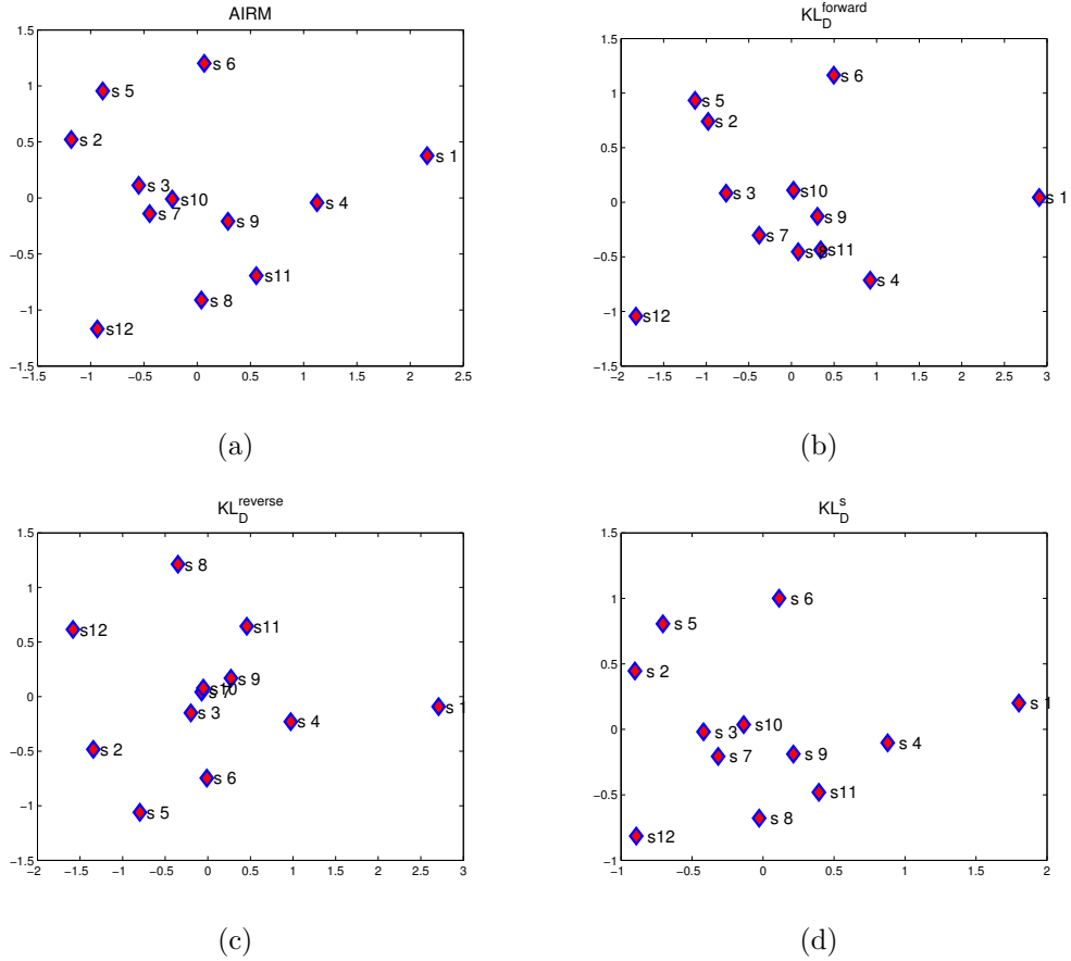
Figure 6.6: 2-D representation of affinity (or similarity) between subjects based on the 4 metrics: 6.6(a): Affine Invariant Riemannian distance, 6.6(b): Kullback-Leibler using forward divergences, 6.6(c): Kullback-Leibler using reverse divergences, 6.6(d): the symmetric version of KL divergence.
