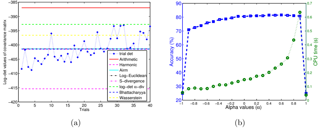
Figure 5.6: (a): Swelling effect of Arithmetic mean shown through log-determinant values. Training trials are taken from the 13 Hz class of the subject with the highest BCI performance. Log-determinant values are given for each trial covariance (points), and for means of Table 5.1 (horizontal lines). (b): Classification accuracy and CPU time, obtained with \alpha -divergence for -1 \leq \alpha \leq 1 .
