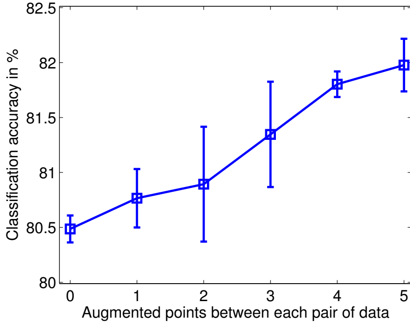
Figure 6.3: Mean classification accuracy in % across all subjects for different levels of data augmentation. At 0, there is no augmented data. At 1, one artificial data is interpolated between each pair of original data within each class, and so forth
