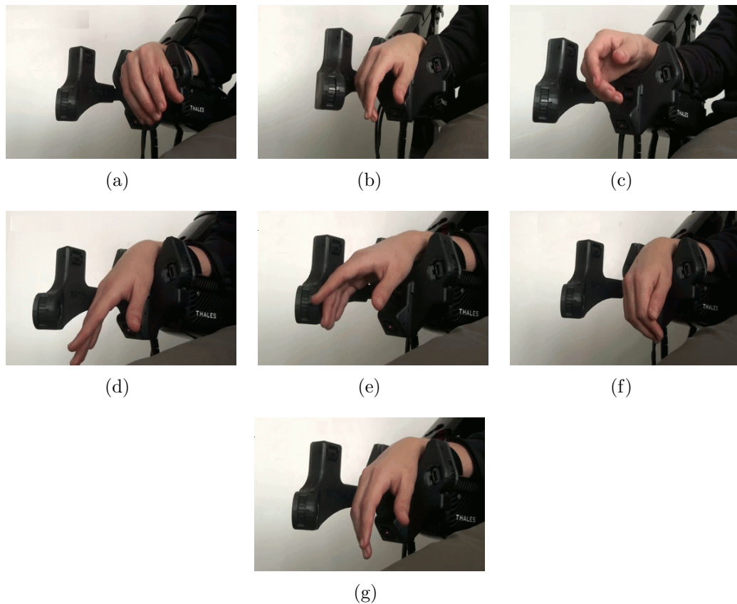
Figure 4.2: The 3D touchless interface and a user's hand positions for different commands: (a) left, (b) right, (c) up, (d) down, (e) forward, (f) backward, (g) rest. The IR-sensors are in the black plastic housing on the right side of the hand and around the wrist. Another symmetrical plastic housing has been realised for left-handed users.
