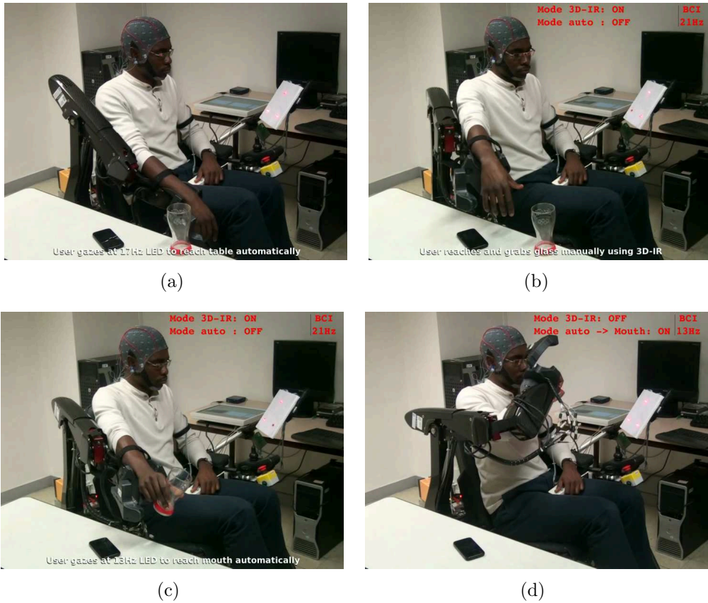
Figure 4.8: Subject sitting on the ESTA wheelchair. His arm is supported by the exoskeleton, and the left hand is lying on the touchless interface. On his right-hand side is the SSVEP stimulation board. He is fitted with an EEG cap for brain signals recording. Next to the exoskeleton, an object is put on a table. (a) The subject is in resting position. He is gazing at the 17 Hz LED to trigger an automatic trajectory to the table. (b) Subject has reached the table and is using the touchless interface to reach and grab the glass (c) Glass in hand, the user gazing at the 13 Hz LED to activate the automatic trajectory to mouth. (d) The arm reaches the mouth while the touchless interface is deactivated.
