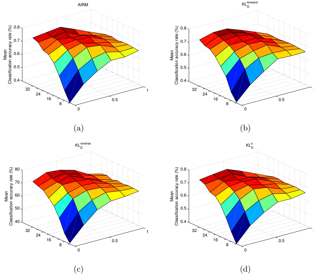
Figure 6.7: Mean classification accuracy for 12 subjects. Grid search with different values of n \in \{4, 8, 12, 16, 20, 24, 28, 32\} on the x-axis and different values of \lambda \in \{0, 0.2, 0.4, 0.6, 0.8, 1\} on the y-axis. The results are obtained using 4 metrics to measure similarity between subjects: 6.7(a) AIRM, 6.7(b) D_{KL}^{\text{forward}} , 6.7(c) D_{KL}^{\text{reverse}} , 6.7(d) D_{KL}^{\text{symmetric}}
