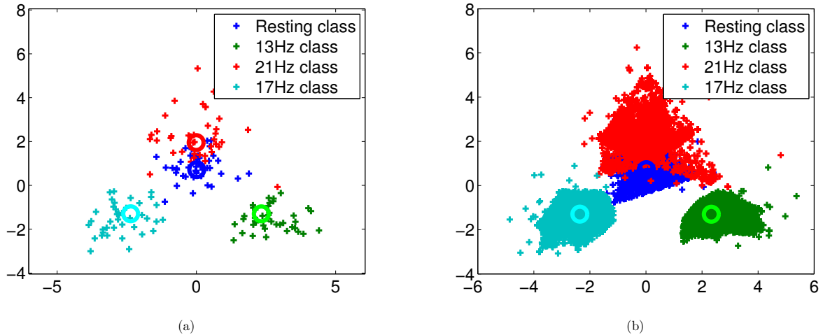
Figure 6.2: Mapping of covariance matrices of trials from each class on the tangent space (5.1.2). Matrices on the tangent space are vectorised and the 2 most significant components from PCA are used to obtain the 2-D representation. The covariance matrices of original data (a) and augmented data (b).
