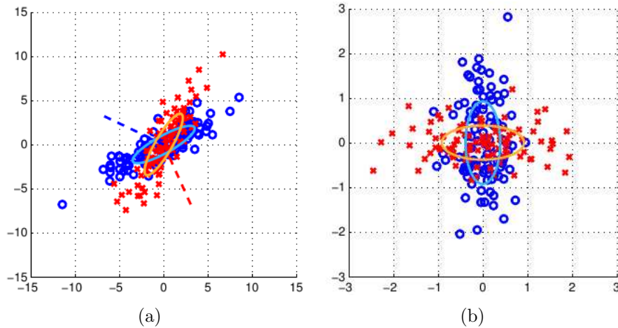
Figure 3.2: CSP effect on class distribution. CSP is applied on a 2D toy data set containing samples from two classes marked with red crosses and blue circles. (a) Samples distribution is shown before CSP filtering. The ellipses show estimates of each class covariance. It can be seen that the two classes are highly correlated. The dashed lines show the direction of the CSP projections \mathbf{w}_j ( j = 1, 2 ). (b) Distributions after CSP projections. The two distributions are orthogonal, showing that the two classes are uncorrelated. Each axis gives the largest variance in one class and the smallest in the other. [Image from Blankertz et al., 2008].
