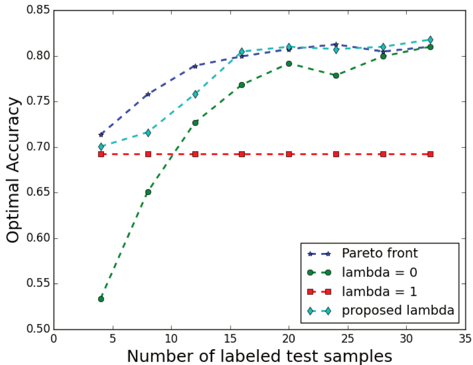
Figure 6.9: Optimal performance (Pareto front) obtained through a grid search is compared with the performance with \lambda = 0 , \lambda = 1 , and \lambda as proposed in (6.3.5).
