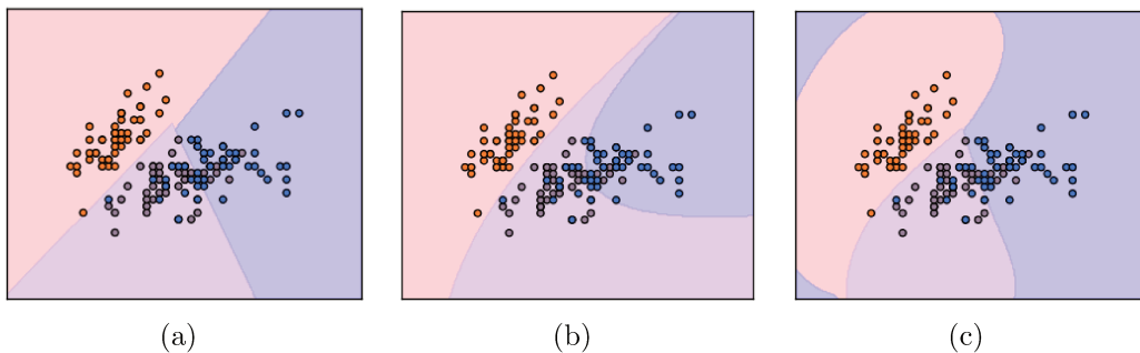
Figure 3.7: Multiclass SVM classification with different kernels on 2D projection of the iris dataset. The decision surface separating three classes are shown. The x-axis and y-axis represent sepal length and sepal width respectively. (a) Linear kernel, (b) polynomial kernel of order 3, (c) RBF kernel [Pedregosa et al., 2011].
