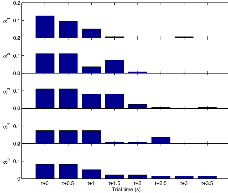
Figure 4.5: Evaluation of the online performances of the proposed BCI algorithm. The error rates for all five subjects are indicated as a function of time, with t+0 indicating the first prediction made (after t_W = 3 s). The error rates are averaged on all classes.
