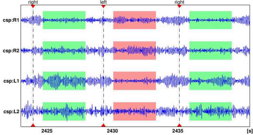
Figure 3.3: Effect of CSP filtering. A continuous EEG signal containing two right-hand imagery epochs and one left-hand imagery is filtered using four CSP filters ( \mathbf{w}_j ): csp:R1, csp:R2, csp:L1, and csp:L2. The resulting signals from csp:R1 and csp:R2 have large variance during left hand imagery, while signals from csp:L1 and csp:L2 have large variance during right hand imagery. [Image from Blankertz et al., 2008].
