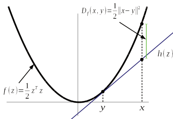
Figure 5.1: Geometry of the Bregman divergence with the seed function f(z) = \frac{1}{2}z^T z . h(z) is a hyperplane tangent to f(z) at y . While it accurately represents f(y) , it underestimates f(x) . The Bregman divergence measures how much the representation of f(x) on h(z) diverges from f(x) (in green).
