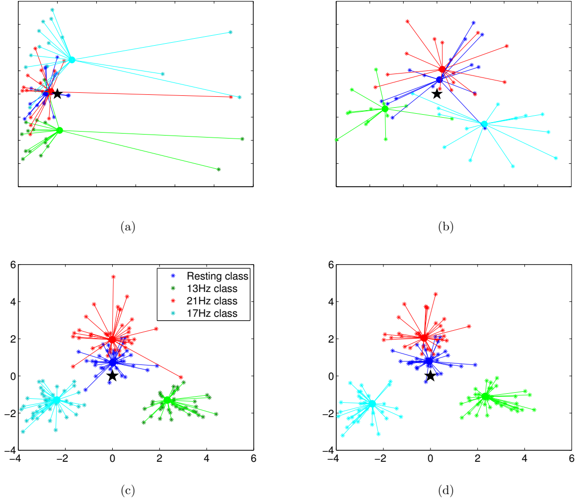
Figure 5.4: Scatter plot of covariance matrices for all trials mapped on the tangent space. The distance between each trial covariance matrix \Sigma_i and its Riemannian mean class \Sigma_\mu^{(k)} is shown as connection line. The black star represents the Riemannian mean of all trials. Subject with lowest BCI performance, (5.4(a)) before and (5.4(b)) after Riemannian potato filtering. Subject with highest BCI performance, (5.4(c)) before and (5.4(d)) after Riemannian potato filtering.
