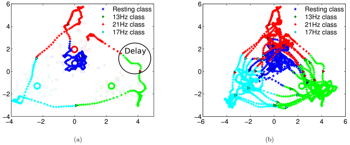
Figure 5.9: The covariance matrices trajectory during a 4-class SSVEP online recording. The circles represent class centres. The triangles mark the beginning of the experiment of a new trial whose class is indicated by the triangle’s colour. 5.9(a) shows the first 7 trials. The first 3 trials are from the resting class, the remaining are respectively class 13 Hz, 17 Hz, and 21 Hz. 5.9(b) shows the entire recording. Data are taken from the subject with the highest BCI performance.
