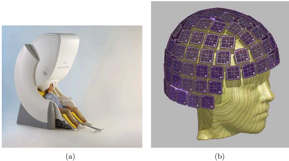
Figure 2.6: Elekta MEG acquisition system. (a) A MEG shield chamber for electromagnetic isolation (b) MEG sensors configuration. Each sensor location is equipped with three sensors: a magnetometer that measures normal field component, and two orthogonal planar gradiometers that measure gradient components [Team, 2016].
