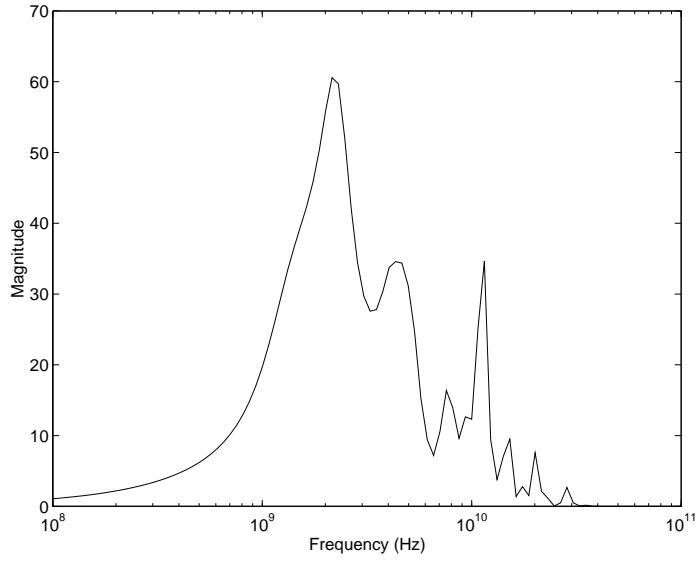
Figure 8.8: Frequency Response of Example 8.2
