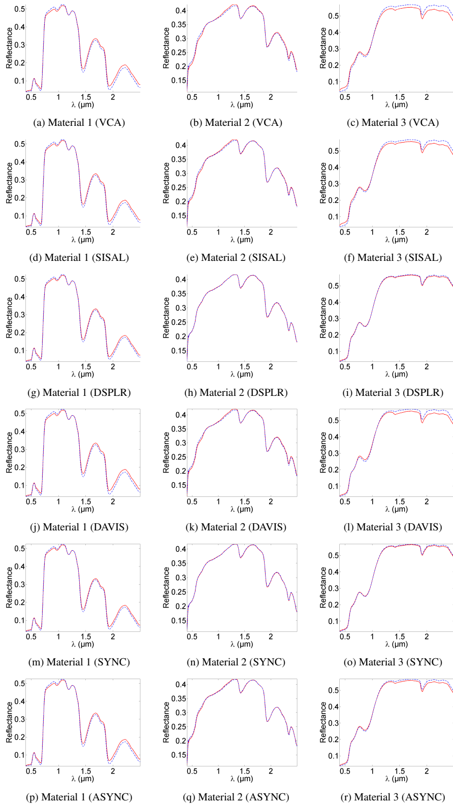
Figure 4.3.: Endmembers (red lines) recovered by the different methods from the synthetic dataset composed of R = 3 endmembers. The true endmembers are given in each figure in blue dotted lines for comparison.
