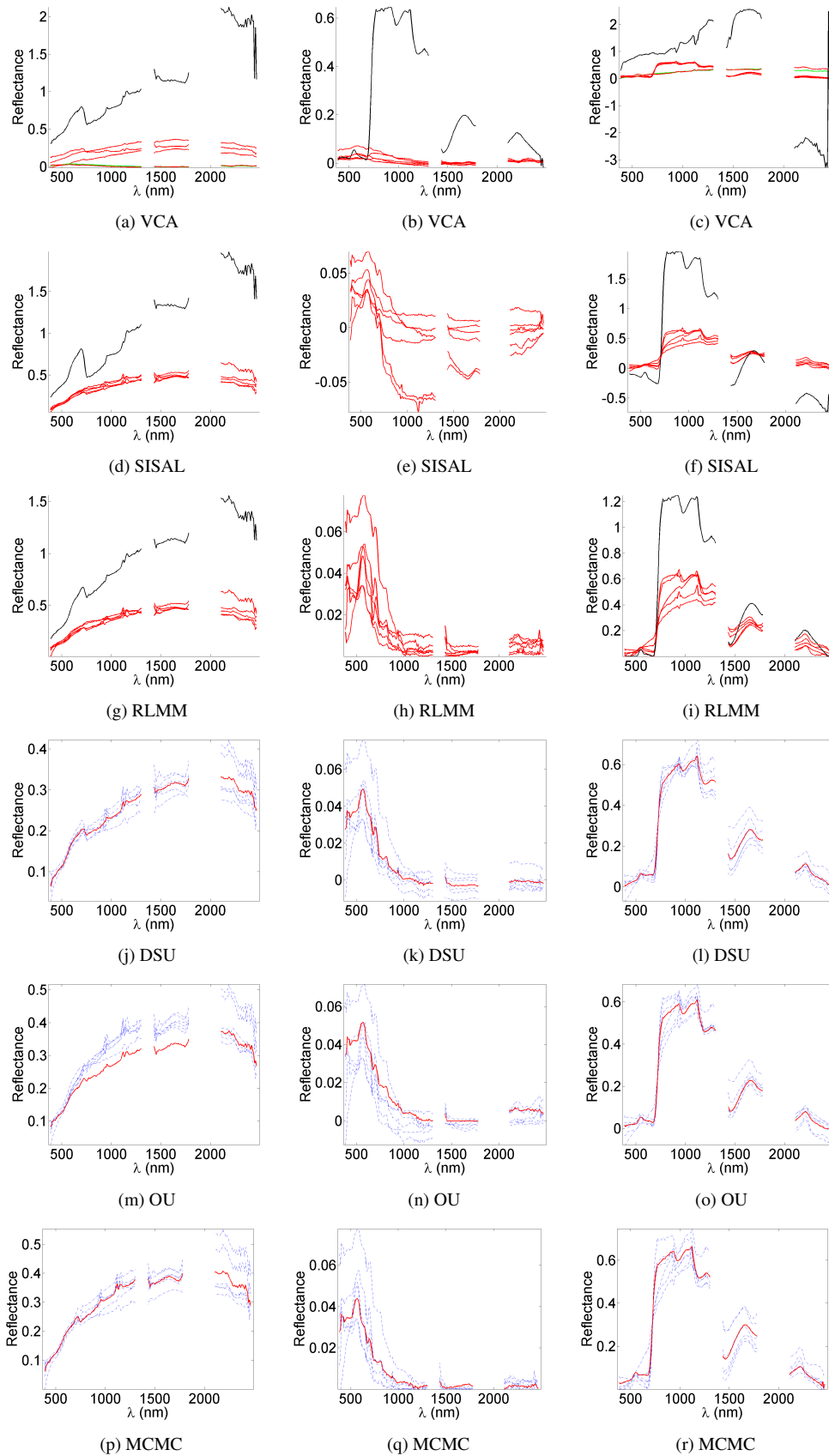
Figure 2.12.: Endmembers ( \mathbf{m}_r , red lines) and their variants affected by variability ( \mathbf{m}_r + \mathbf{d}\mathbf{m}_{r,t} , blue dotted lines) recovered by the different methods from the real dataset depicted in Fig. 2.8. Signatures corresponding to different time instants are represented in a single figure to better appreciate the variability recovered from the data. The spectra represented in black correspond to signatures corrupted by outliers, while those given in green represent endmembers which have been split into several components by the associated estimation procedure.
