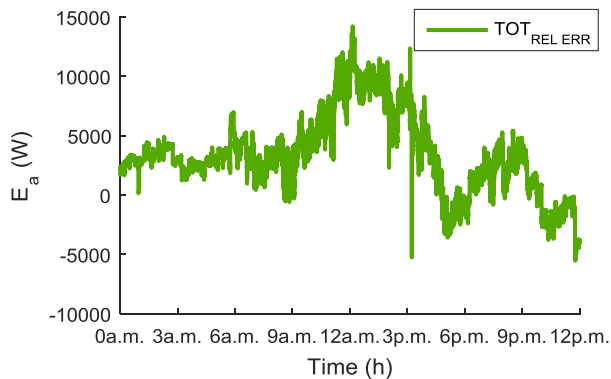
Fig. V.51 Absolute error between forecasted and real values of total microgrid power ( \epsilon_a^{PV+C} )
