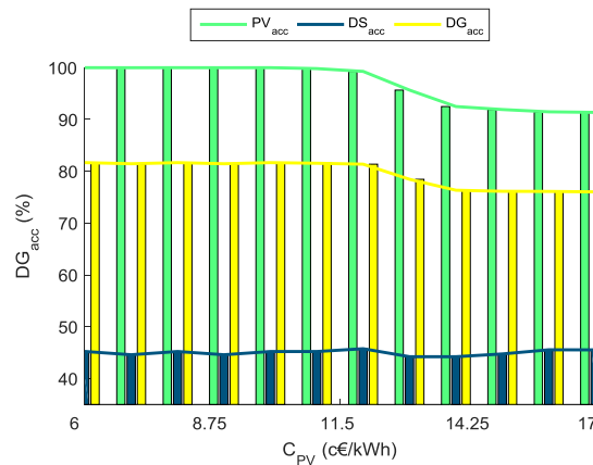
Fig. III.31 Influence of CPV variation on DG_{acc} , PV_{acc} , DS_{acc}
