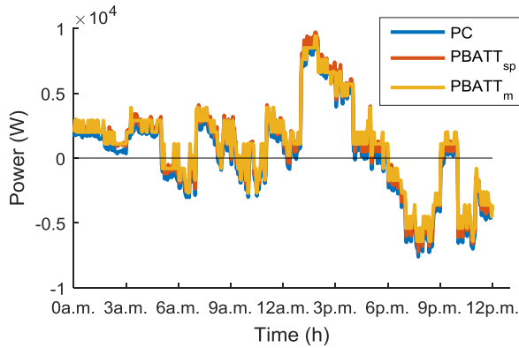
Fig. V.37 Comparison between P_C , P_{BATT_{sp}} and P_{BATT_m} with intra-day re-optimizations
