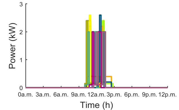
Fig. III.25 Appliance activation for case study 1
