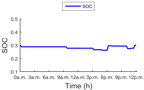
Fig. III.24 ESS SOC for case study 2
