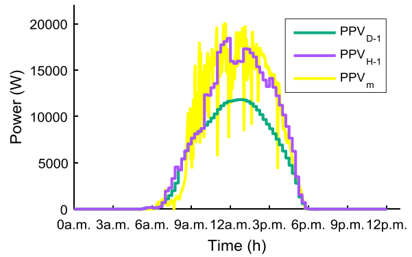
Fig. V.85 Comparison between D-1, final re-forecasted and measured PV profiles
