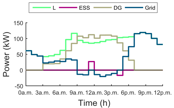
Fig. III.11 Microgrid aggregated daily profiles (grid exchange, consumption, generation and storage)
