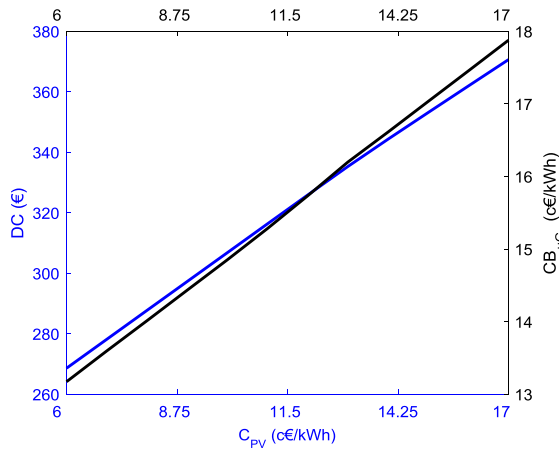
Fig. III.30 Influence of CPV variation on DC and CB_{\mu G}
