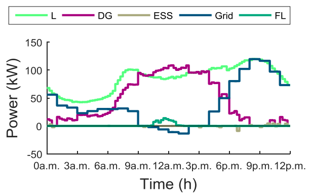
Fig. III.15 Microgrid aggregated daily profiles (grid exchange, consumption, generation and storage) for case study 1
