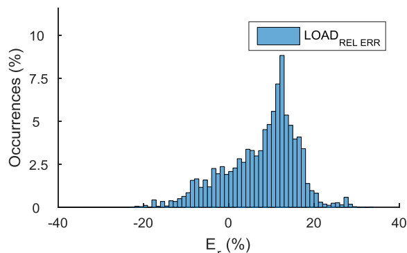
Fig. V.50 Distribution of \epsilon_a^C on microgrid P_n
