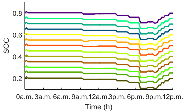
Fig. III.37 Influence of SOC_{start}/SOC_{end} variation on battery SOC
