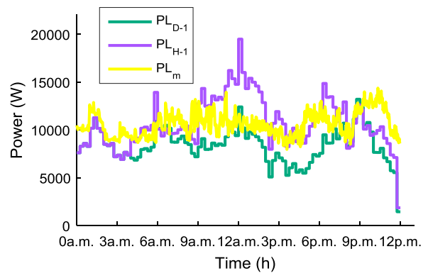
Fig. V.40 Comparison between D-1, final re-forecasted and measured consumption profiles
