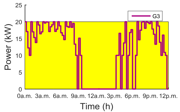
Fig. III.23 DS input and output of group 3 for case study 2
