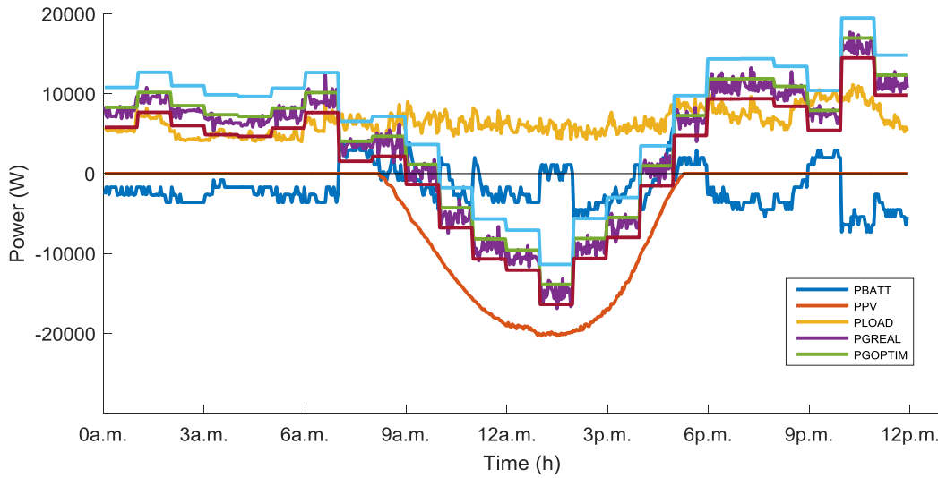
Fig. V.64 Real power profiles of photovoltaic, battery, consumption and grid exchange in t_m with intra-day re-optimizations
