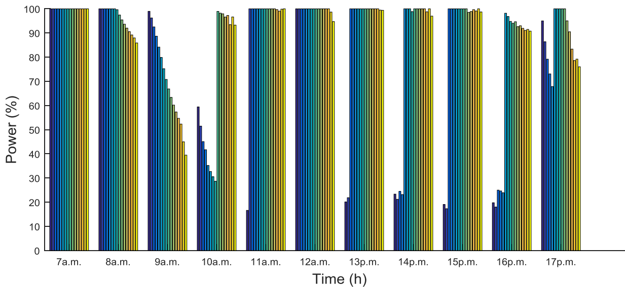
Fig. IV.37 Influence of PPV_{max} in the hourly power accepted for Microgrid 2
