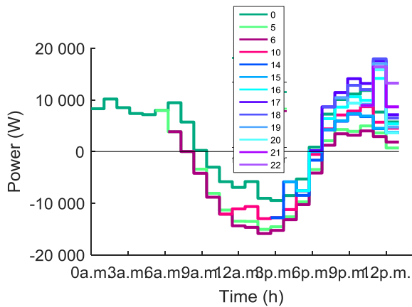
Fig. V.19 Net microgrid's power scheduled with intra-day re-optimizations
