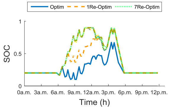
Fig. IV.29 SOC of ESS in Microgrid 2 for CLAM
