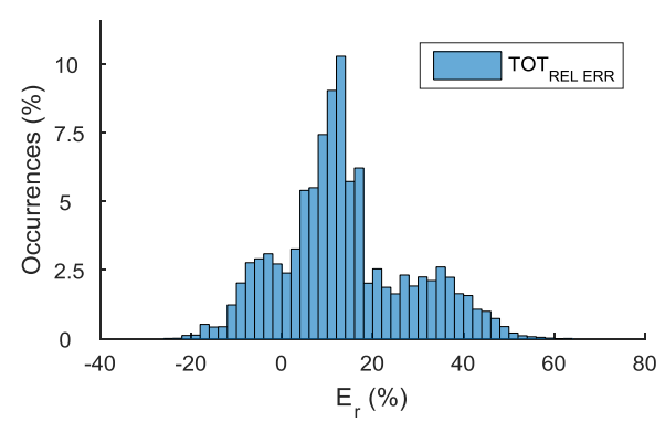
Fig. V.75 Distribution of \epsilon_a^{PV+C} on microgrid P_n
