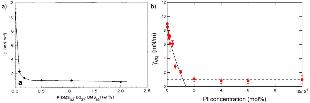
Figure 2.6: a) Interfacial tension (in mN/m) between PEO 35 ( M_n = 32000 g/mol) and PDMS 100 ( M_w = 177000 g/mol) for different concentrations of pre-made P(DMS 32 -EO 37 -DMS 32 ) copolymers (in wt%) in the PEO phase (from [128]). b) Interfacial tension between PEG 400 ( M_w = 400 g/mol) and reactive PDMS ( M_w = 2000 g/mol) for different concentrations in platinum Pt (in mol%) in the PEG phase which allows the reaction between the PEG and the reactive PDMS (adapted from [122]).
