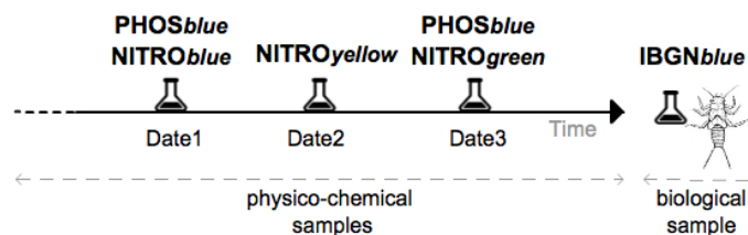
Figure 7.15: Hydro-ecological sequence
