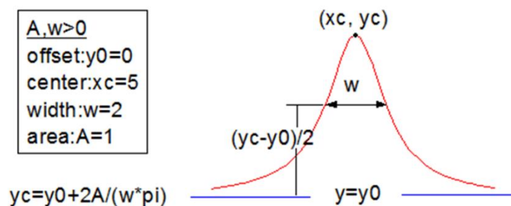
Equation 1 : Equation of a single Lorentzian function
