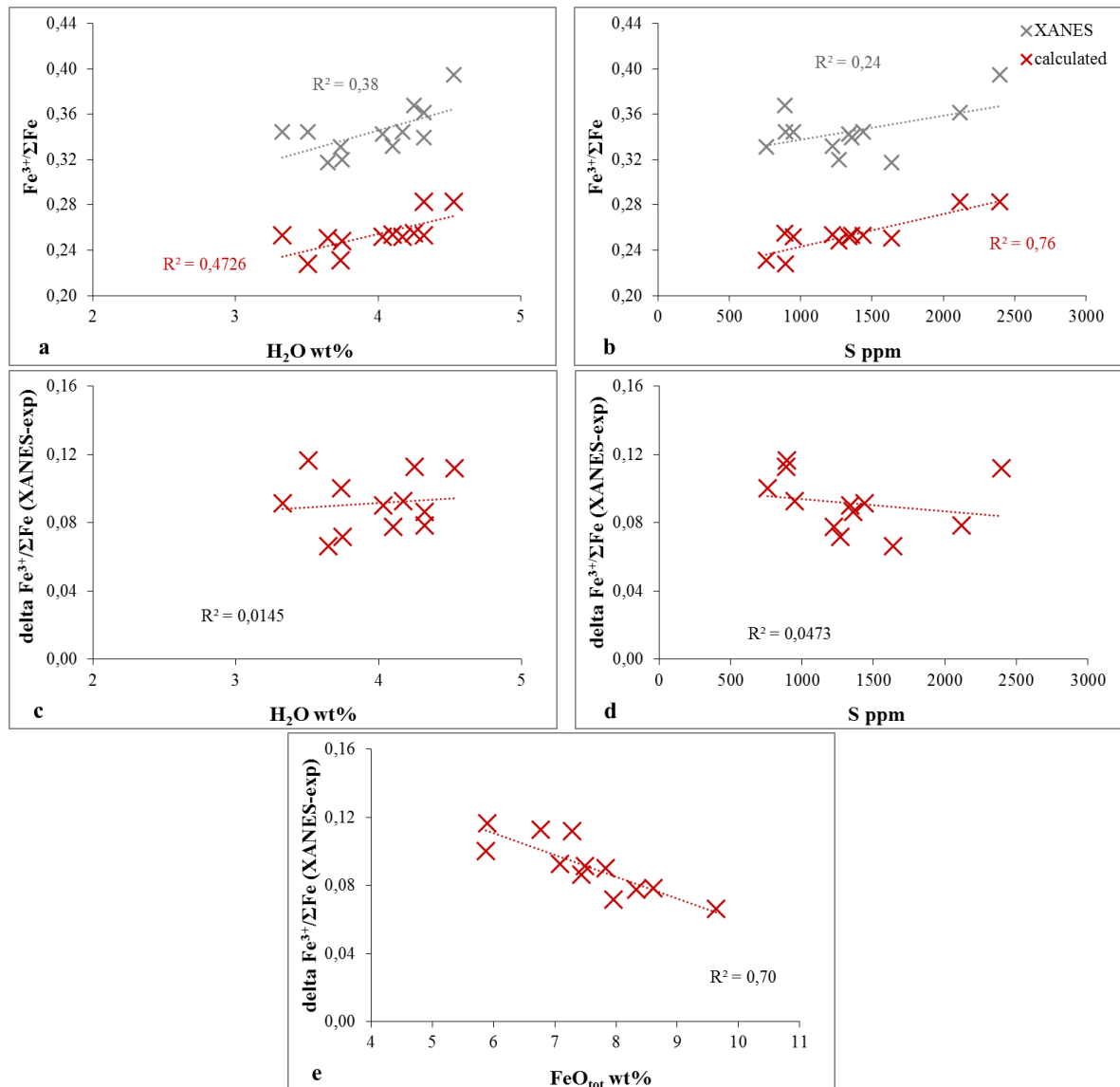
Fig. 4.23 - a-b) Fe 3+ /ΣFe ratios estimated by XANES spectroscopy (gray symbols) and those previously calculated from the experimental f_{\text{O}_2} (using Kress and Carmichael, 1991) in the experimental glasses (red symbols), versus H 2 O and S contents. The difference between XANES Fe 3+ /ΣFe ratios and experimental Fe 3+ /ΣFe ratios versus H 2 O (c), S (d) and FeO tot (e) contents in the experimental glasses.
