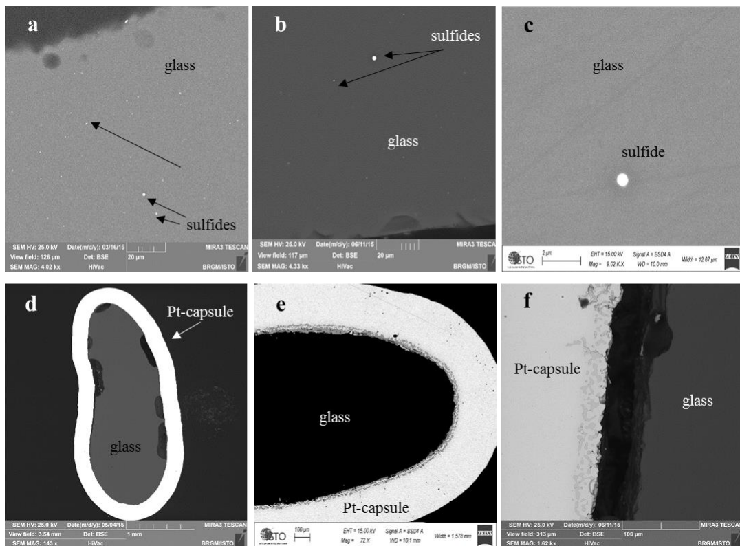
Fig. 4.16 - Backscattered electron images of experimental products: a-b-c) glasses (1702#3-2704#4 - 1902#1) with small sulfide globules. d) Bubbles located at the glass-capsule interface (2703#3); e-f) reaction rims (S-Pt-Fe) in the Pt capsules.
