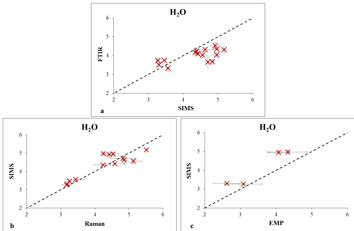
Fig A5.4 - H 2 O contents (reported in wt.%) in the experimental glasses determined by several methods: a) FTIR versus SIMS; b) SIMS versus Raman; c) SIMS versus EMP.
