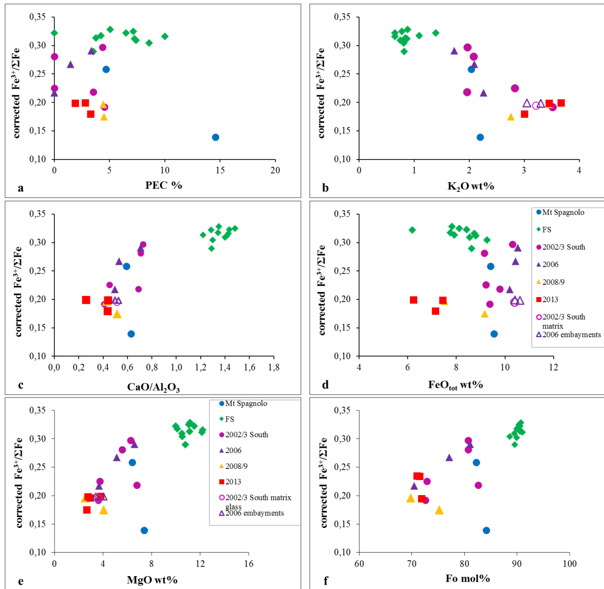
Fig. 4.24 - a) Plot of Fe 3+ /ΣFe ratios with calculated amount of post-entrapment crystallization (in %) for each melt inclusion. b) Fe 3+ /ΣFe ratios versus K 2 O contents, used as index of melt differentiation. c) Fe 3+ /ΣFe ratios versus CaO/Al 2 O 3 ratio and d) FeO tot content. The absence of correlation between the Fe 3+ /ΣFe ratios and PEC shows that post-entrapment processes are unlikely to have exerted a strong influence on the measured Fe oxidation state. The slight correlation with K 2 O contents and CaO/Al 2 O 3 ratio indicate a possible change in the Fe 3+ /ΣFe ratio with differentiation.
