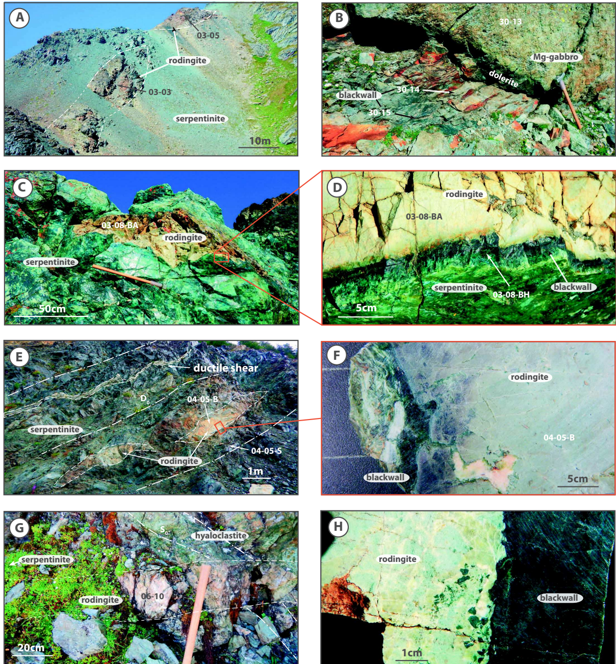
Fig. 1-2: Photographs of rodingites, gabbros and associated blackwalls in the field. A) Rodingite dike crosscutting mantle rocks (serpentinites). B) Contact between a massive gabbro and its chlorite-blackwall. Note the dolerite forming the chilled margin demonstrating slow cooling. C) Typical sigmoidal shape of rodingite in serpentinite. D) Close up photograph of the same dike as for C) highlighting the thin blackwall between the dike and the serpentinite. E) Sigmoidal dike of rodingite with ductile shear) enclosed in a decametric scale shear-zone. F) Rodingite with mylonitized contact. Serpentine and blackwall are both mylonitized by a ductile transtensional event. G) Hyaloclastite laying on serpentinite (not visible here) and crosscut by a rodingite dike. Dykes can develop after basalt flow extrusions on exhumed mantle. H) Close-up photograph of a thick blackwall.
