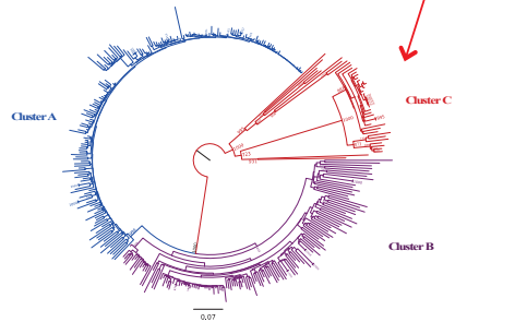
The SIRE lineage contains three families, A, B and C in C. canephora . Longer branches for family C suggest that it is older than the two others.
