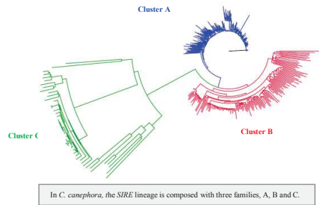
In C. canephora , the SIRE lineage is composed with three families, A, B and C.
