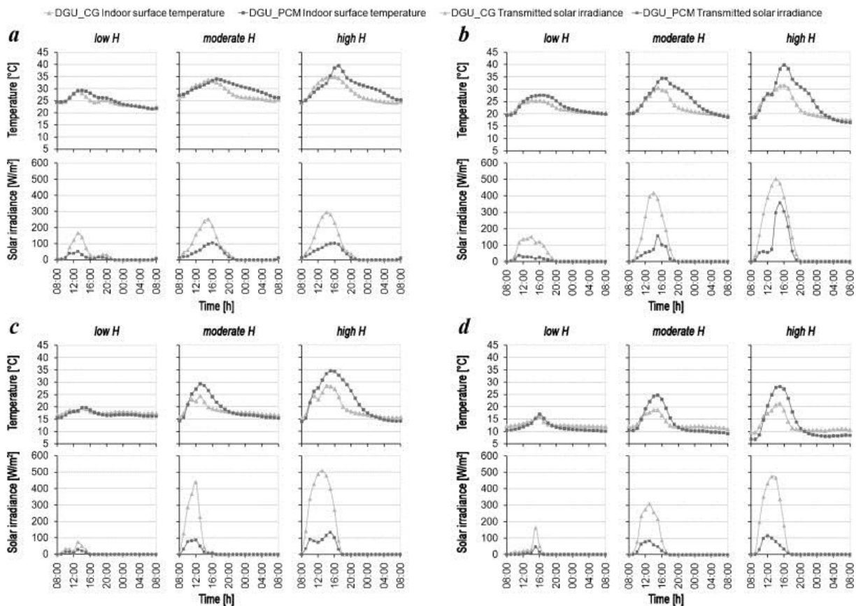
Figure 2.13 – Goia et al. summer (a), mid-season (warm period) (b), mid-season (cold period) (c), and winter (d) – surface temperatures ( \vartheta_{surf}^{PCM} and \vartheta_{surf}^{CG} ) and transmitted irradiances ( I_t^{PCM} and I_t^{CG} ).
