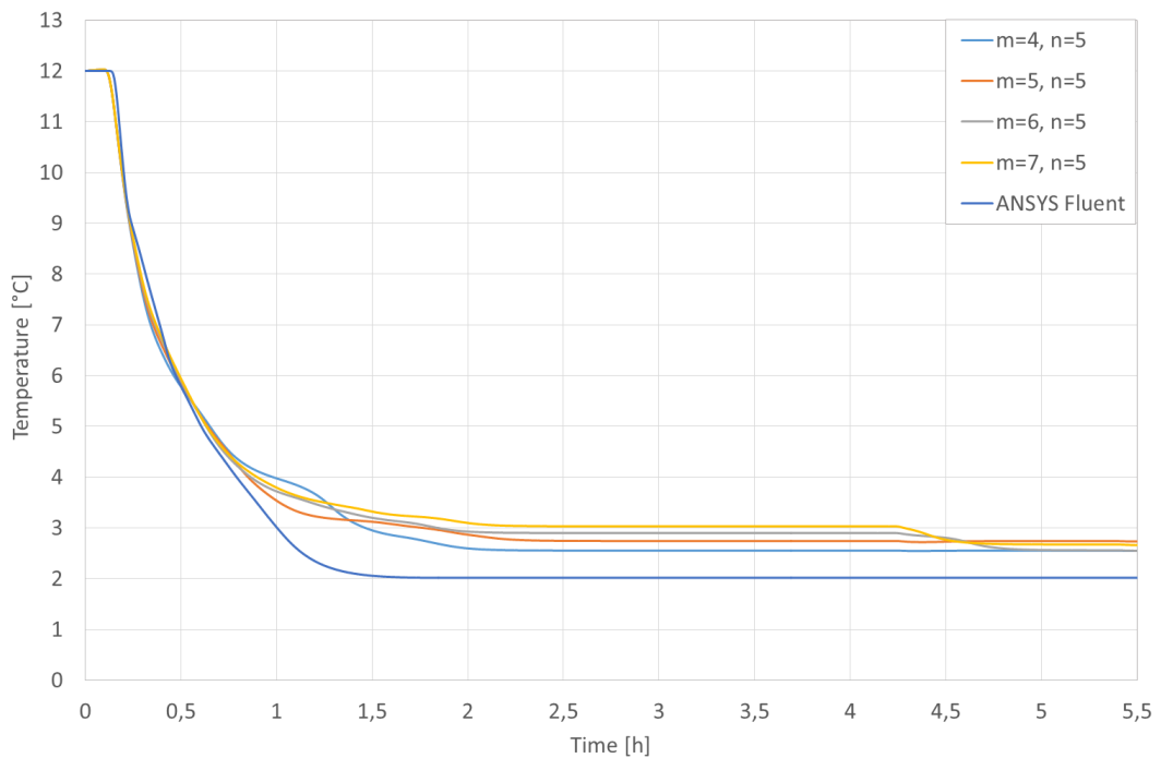
Figure 4.13 - Comparison of the temperature curves obtained with the two different software in the first step of the 0.00045 kg/s water flow rate for the same point obtained using different crosswise discretization and the same lengthwise discretization ( n = 5 ).
