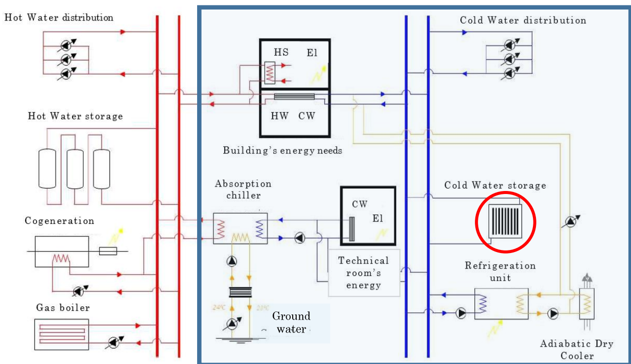
Figure 6. 1 - Scheme of the HVAC system of HIKARI. The HIKARI cooling systems set is indicated into the blue square, in particular the thermal energy storage system analysed in this work is indicated in the red circle.
