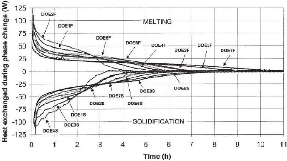
Figure 2. 8 - Zalba’s et al. unit’s heat transfer during phase change for different configurations.
