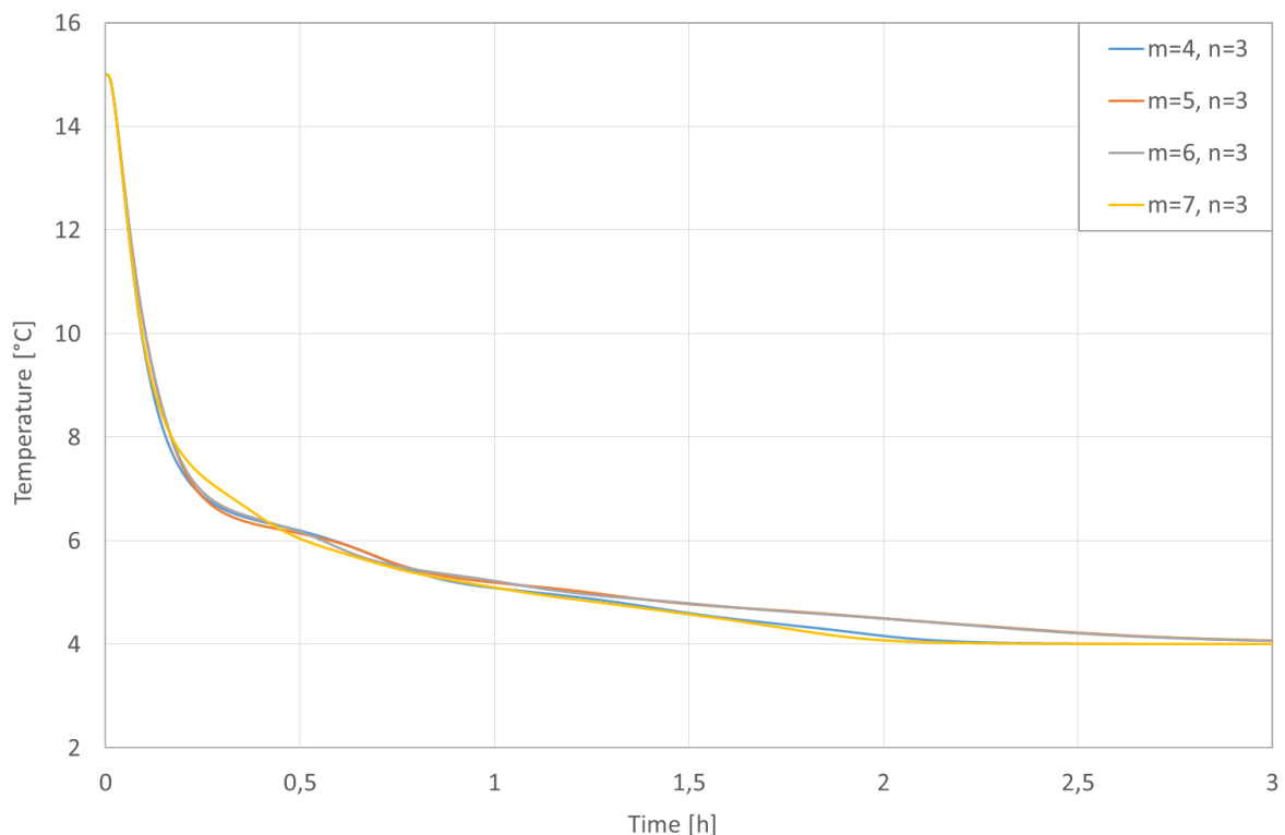
Figure 3. 15 - Example of difference between the temperature curves obtained in the same control volume ( i = w, j = n ) with various models lengthwise discretized in 3 nodes and crosswise discretized between 4 and 7 nodes.
