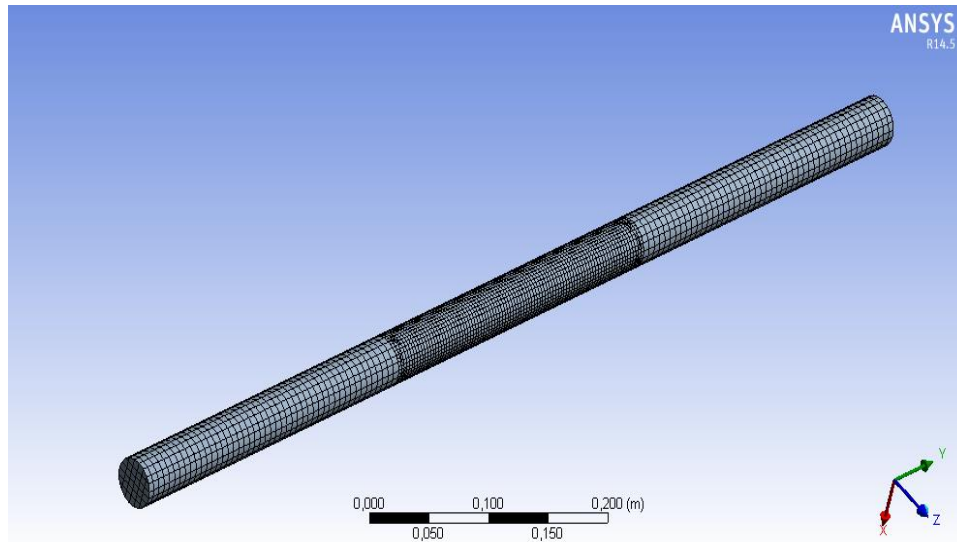
Figure 4. 3 -Meshing of the model realized through the Mesh interface.
