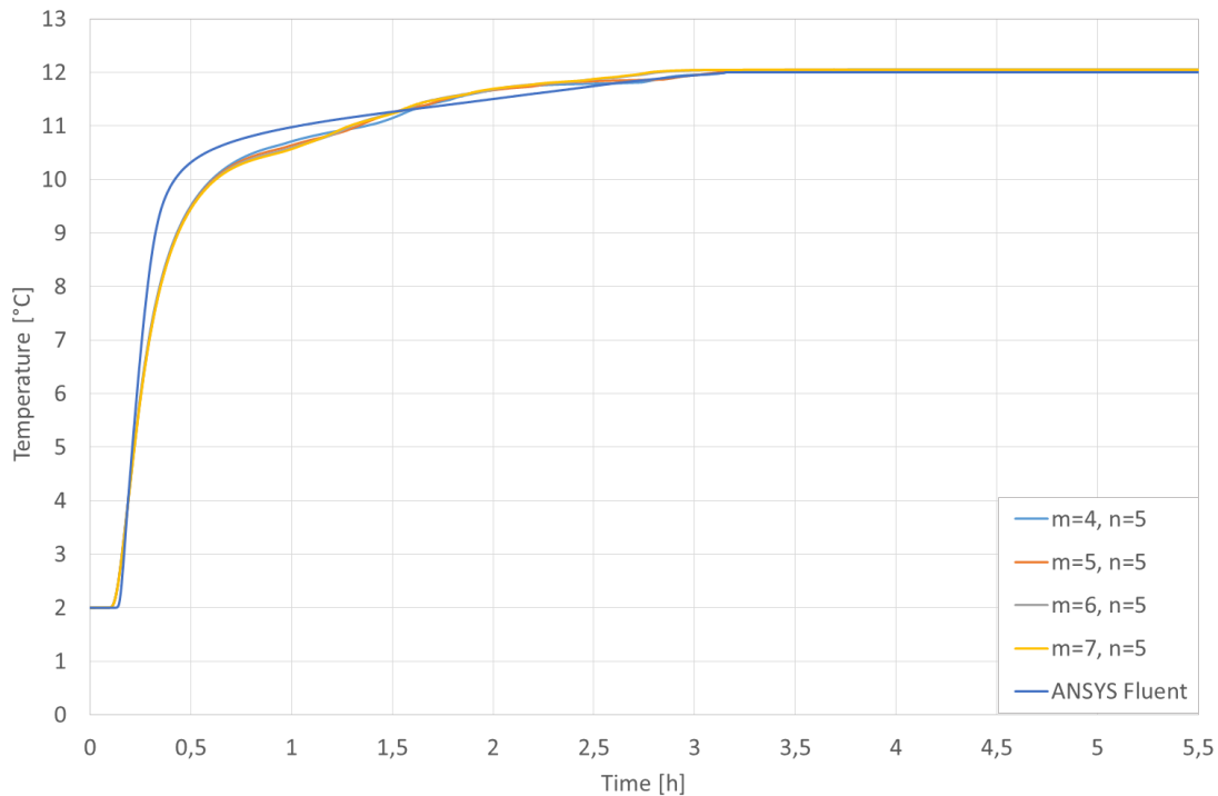
Figure 4.15 - Comparison of the temperature curves obtained with the two different software in the second step of the 0.00045 kg/s water flow rate for the same point obtained using different crosswise discretization and the same lengthwise discretization ( n = 5 ).
