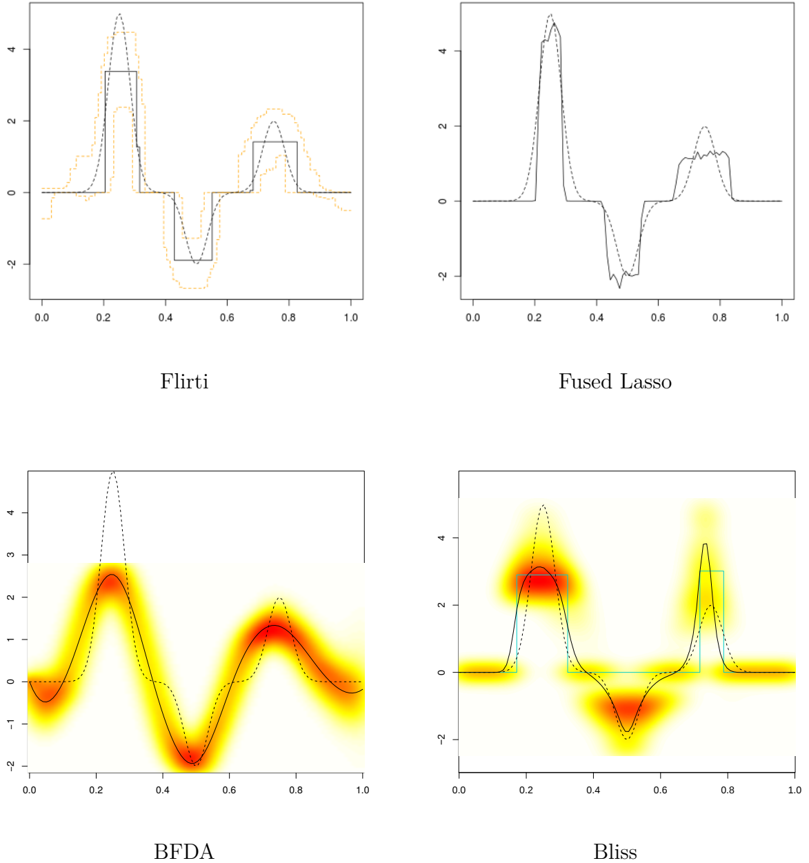
Figure 2.5: Estimates of the coefficient function on Dataset 13 ( r = 3 , \zeta = 1 )). For each plot, the black dotted line is the true coefficient function (Smooth, in this case) and the solid black lines are the estimates of each method. Concerning the Flirti plot, the orange dotted lines correspond to the confidence bands of the estimate. For the Bayesian methods (BFDA and Bliss) a representation of the marginal posterior distributions of \beta(t) are represented using heat maps, as described in Section 2.2.7. Red (resp. white) colour is used to represent high (resp. low) posterior densities. For the Bliss plot, the solid black line is the L^2 -estimate and the light blue line is the stepwise Bliss estimate.
