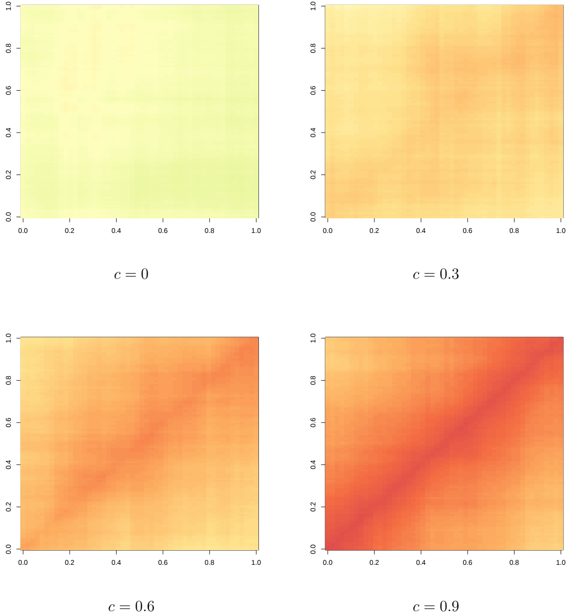
Figure 2.8: Cross-covariance matrix between the curves x_{i1}(\cdot) and x_{i2}(\cdot) detailed in Section 2.3.5 for different values of c . Each point (t, t') represents the cross-covariance between x_{i1}(t) and x_{i2}(t') . Red (resp. yellow) represents high (resp. low) cross-covariance.
