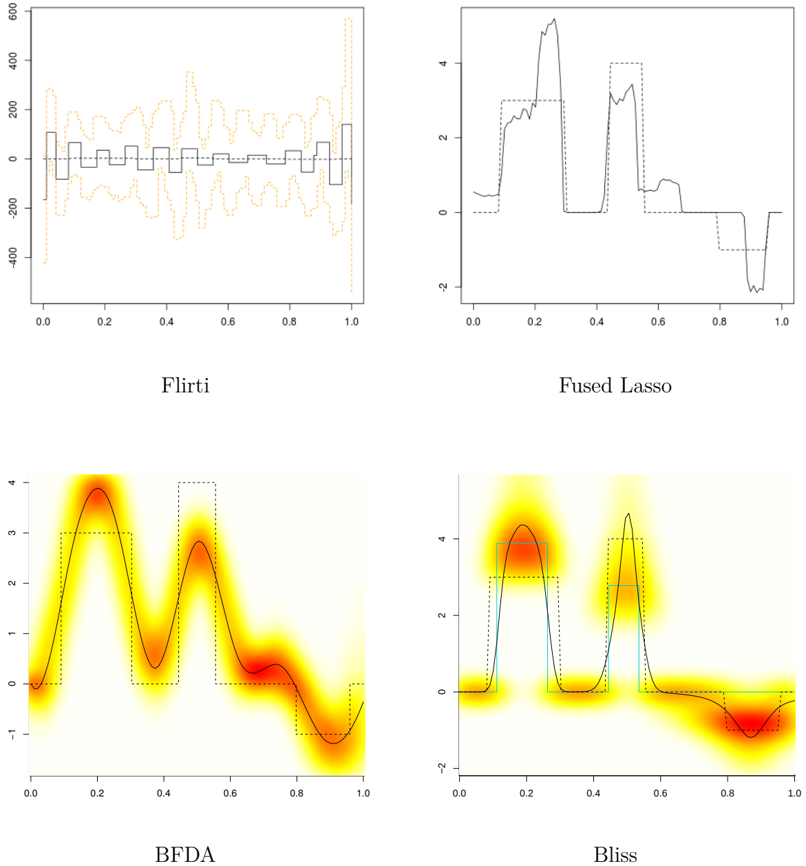
Figure 2.4: Estimates of the coefficient function on Dataset 4 ( r = 3 , \zeta = 1 ). For each plot, the black dotted line is the true coefficient function (Step function, in this case) and the solid black lines are the estimates of each method. Concerning the Flirti plot, the orange dotted lines correspond to the confidence bands of the estimate. For the Bayesian methods (BFDA and Bliss) a representation of the marginal posterior distributions of \beta(t) are represented using heat maps, as described in Section 2.2.7. Red (resp. white) colour is used to represent high (resp. low) posterior densities. For the Bliss plot, the solid black line is the L^2 -estimate and the light blue line is the stepwise Bliss estimate.
