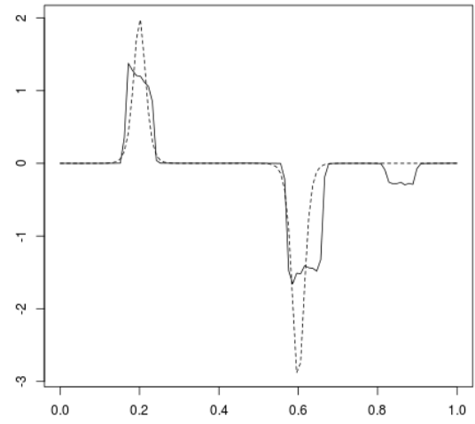
Fused Lasso
