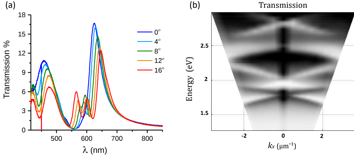
Figure 3.9: (a) The zero-order transmission spectra as a function of incident angle of the light in TM mode. Spectra were taken every 4° up to 16° for hexagonal array in Ag ( a_0 = 400 nm, hole diameter = 205 nm, film thickness = 200 nm). (b) The energy-momentum dispersion of the same spectra present in (a) in addition to their symmetric values for negative angles. The bright lines represent peaks and dark ones represent dips.
