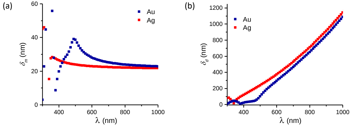
Figure 3.4: The spatial extension of SPPs into the metal \delta_m (a) and dielectric \delta_d (b) media as calculated from equation (3.3) for Au-air and Ag-air interfaces.
