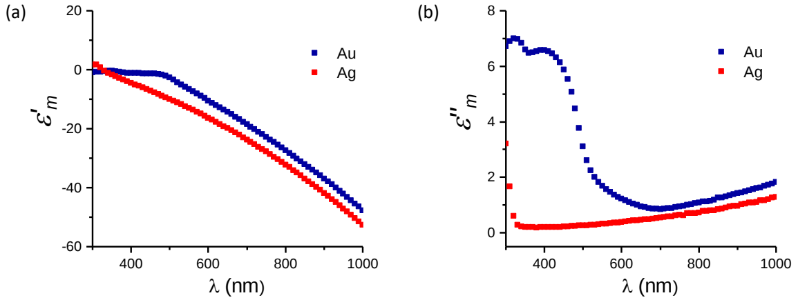
Figure 3.2: The real (a) and imaginary part (b) of the permittivity of silver (Ag) and gold (Au) as a function the wavelength \lambda . The values were calculated from the complex index of refraction taken from reference [101]. 101
