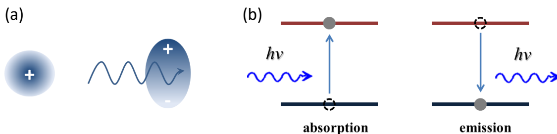
Figure 1.1: Schematic representation of basic light-matter interaction. (a) Atom with a positively charged center and its electronic cloud before and after its interaction with light which leads to the formation of a transient dipole moment. (b) Successive absorption and emission of a photon of energy h\nu by a two-level atom/molecule.
