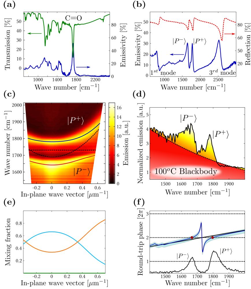
Figure 3.9 – (a) Emissivity spectrum of a 2 \mu\text{m} thick film of PMMA on a Si substrate at 100°C (blue curve). The transmission spectrum of PMMA on a Ge substrate is shown for comparison (green curve). (b) Emissivity spectrum of the strongly coupled cavity at 100°C (blue curve), and simulated cavity reflection spectrum using the transfer matrix calculation of Fig. 3.8(b). (c) Angle-resolved TE emission spectrum of the strongly coupled cavity and coupled-oscillators dispersions obtained from the previously determined parameters with a thermal expansion of 0.115 \mu\text{m} of the 2 \mu\text{m} thick active layer. The corresponding Hopfield coefficients for |P^- \rangle are shown in (e), with the photonic fraction (cyan), the vibrational fraction (orange) and the non-RWA terms (green). (d) Normal incidence emission over absorption ratio (black curve), compared to the expected blackbody distribution (black dashed curve). The absorption is calculated from the fit of the cavity transmission spectrum measured at 100°C. (f) Round-trip phase accumulation of the cavity photon with (blue curve) and without (black line) the absorber. The polaritonic resonances (black transmission spectrum) occurs at the positions indicated by the red dots, where the phase accumulation equals 4\pi .
