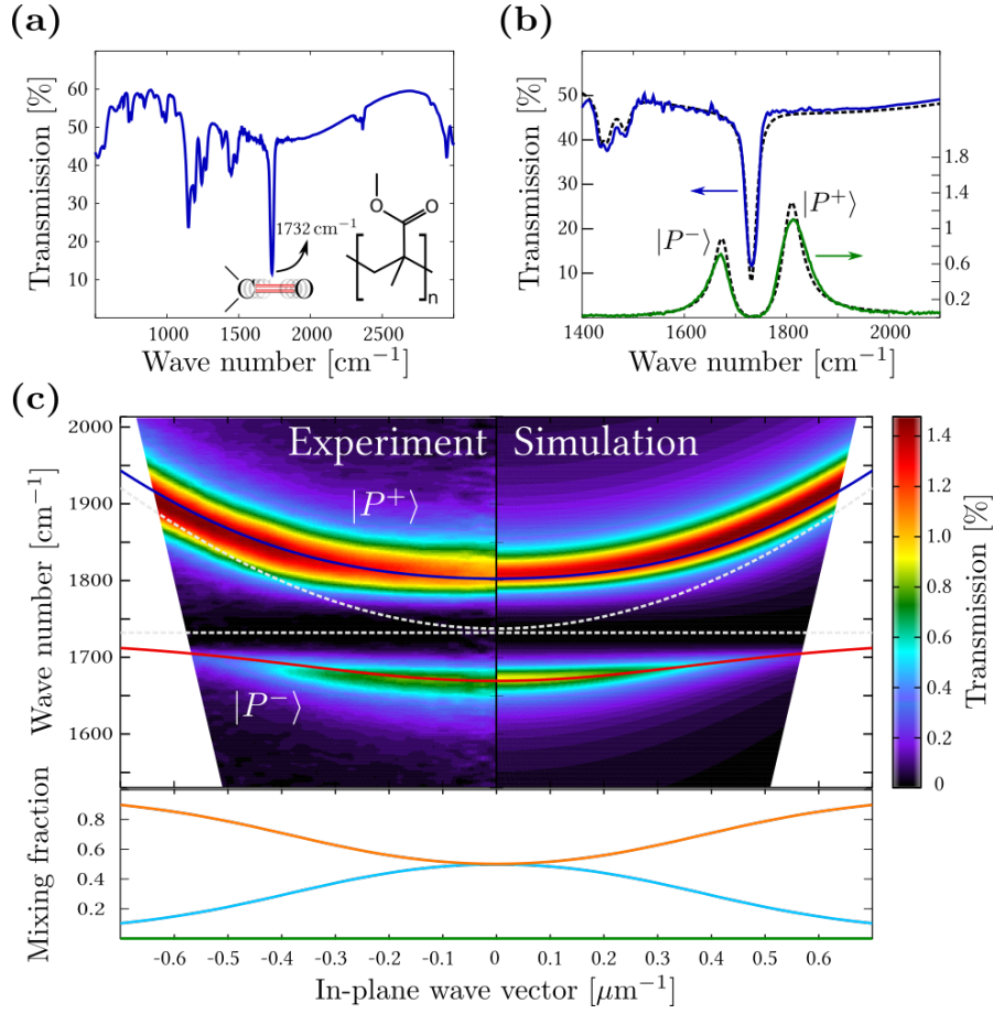
Figure 3.8 – (a) IR transmission spectrum of a 2 μm thick PMMA layer (molecular structure in inset) spin-coated on top of a Ge substrate. (b) IR transmission spectra of the resonantly coupled PMMA cavity (green curve), compared to the bare PMMA transmission spectrum (blue curve). The transfer matrix predictions are shown by the black dashed curves. (c) Angle-resolved transmission spectra measured under TE illumination (left) and the corresponding transfer matrix prediction (right). The solid curves are the fitted solution of the coupled oscillators model (3.21) and the white dashed curves are the dispersions of the corresponding uncoupled modes. The lower panel shows the photonic ( |w_-|^2 , cyan curve) and the vibrational fractions ( |x_-|^2 , orange curve) composing the lower polaritonic state. The non-RWA terms |y_-|^2, |z_-|^2 are shown in green.
