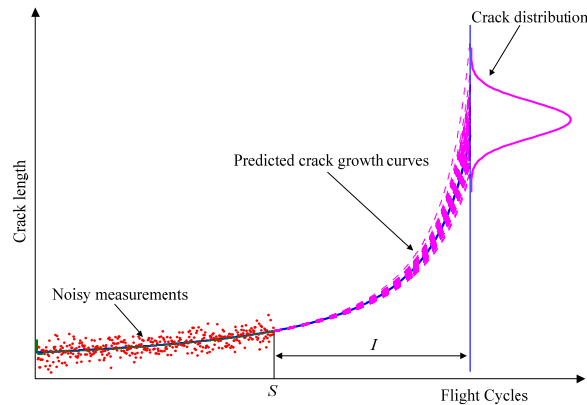
Figure 4-1 Schematic diagram of predicting crack size using Monte Carlo method
