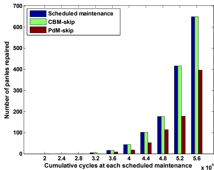
Figure 5-10 Comparison of maintenance strategies in terms of the number of repaired panies at each scheduled maintenance stop
