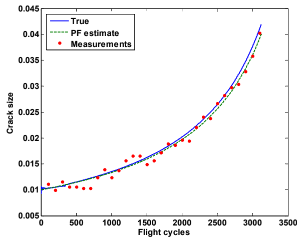
Figure 3-12 Crack size estimation by PF, in the case of only C is estimated in the case of estimating “ m ” and “ C ” simultaneously
