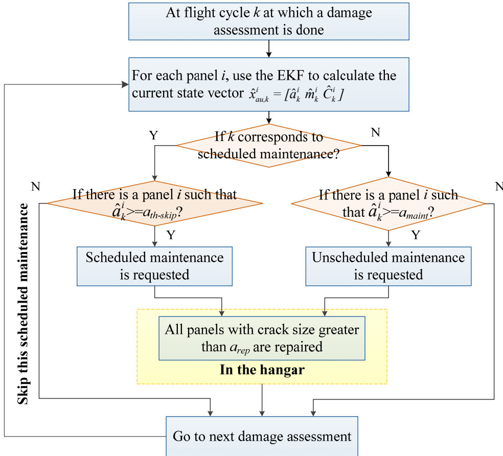
Figure 5-7 Flow chart of CBM-skip
