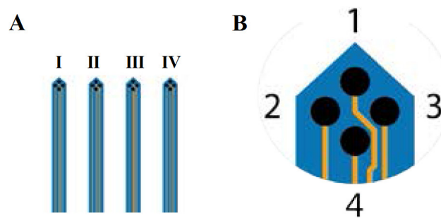
Figure 41: Silicon probe structure with 16 channels. (A) Four parallel shanks of the probe (I-II-III-IV) were used to record activities from a large area with 150 \mu\text{m} spacing between each shank (B) Four recording sites (1,2,3,and 4; each having 15 \mu\text{m} diameter) were positioned in a diamond shape separated with \sim 20 \mu\text{m} distance in our custom design, which gave different voltage recordings that helped spike sorting (see Figure 21 and 22).
