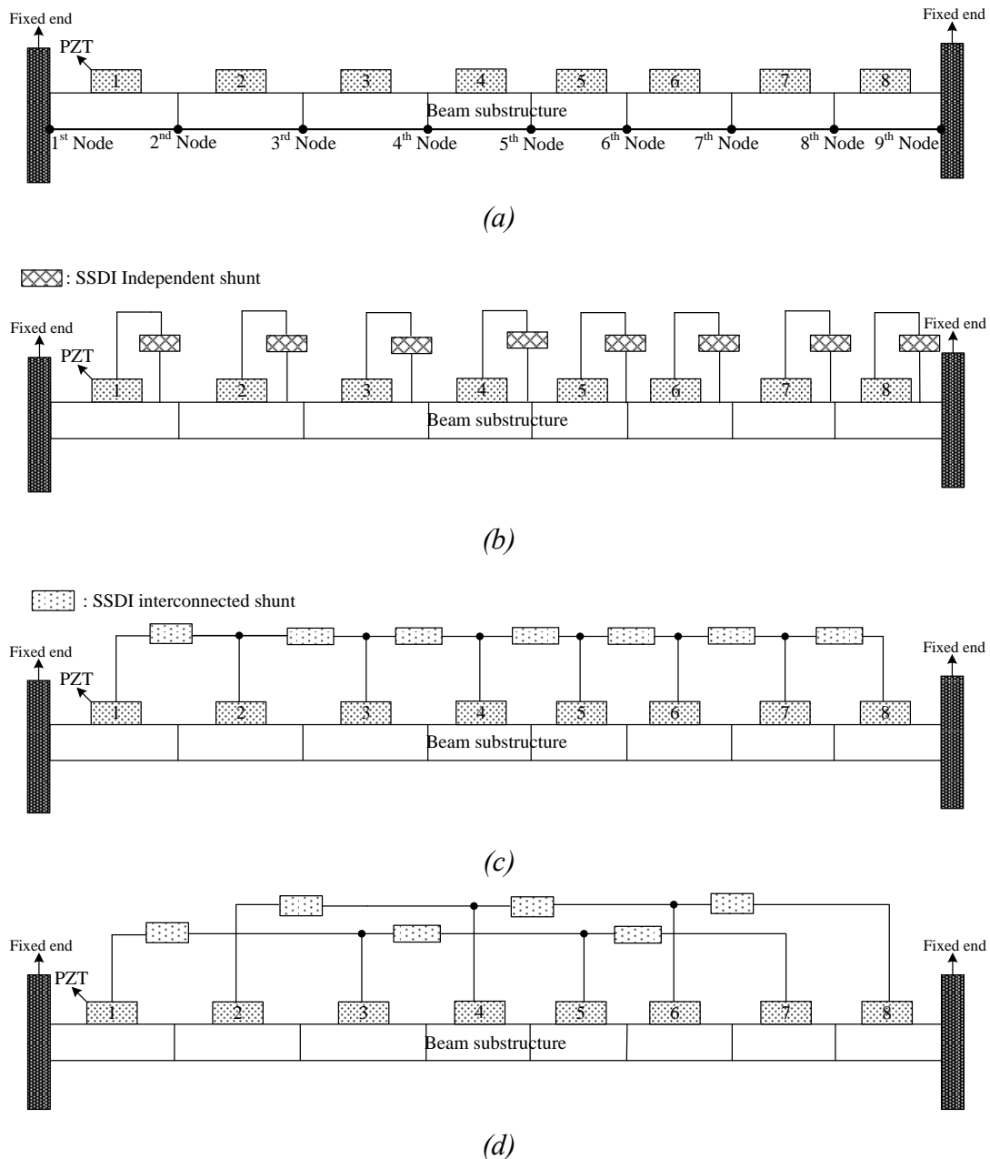
Figure 5.15 Clamped-clamped piezoelectric periodic beam (a) in open circuit condition; (b) with SSDI independent electrical networks; (c) with SSDI 1-level interleaved-interconnected electrical networks; (d) with SSDI 2-level interleaved-interconnected electrical networks.
