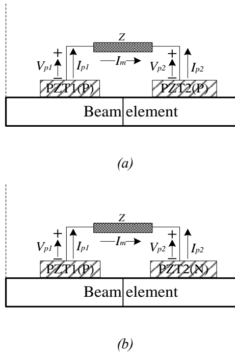
Figure 3.43 (a) Dual-connected periodic cell i with PP configuration; (b) Dual-connected periodic cell i with PN configuration. Z is the SSDI impedance.
