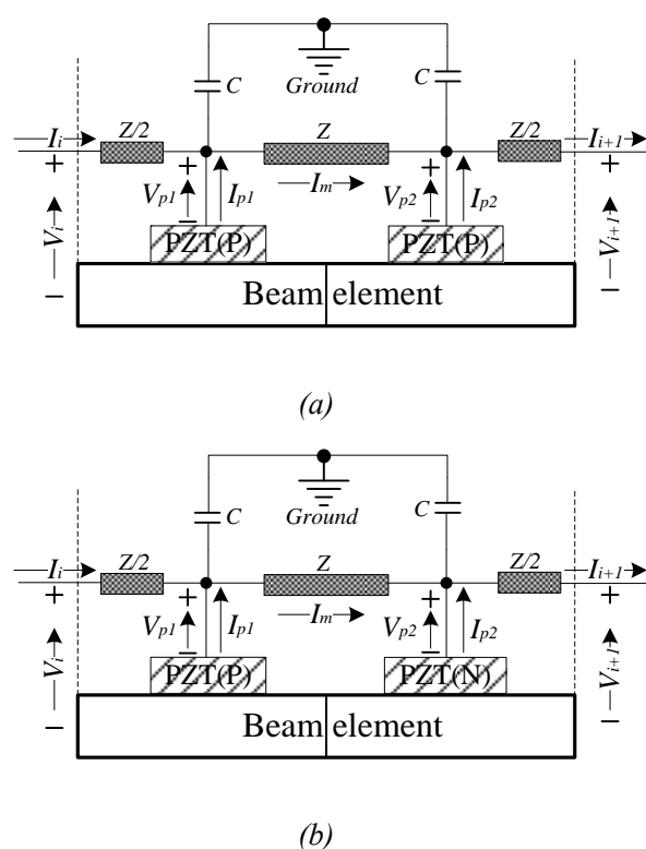
Figure 3.39 (a) Hybrid-Capacitance interconnected periodic cell i with PP configuration; (b) Hybrid-Capacitance interconnected periodic cell i with PN configuration. Z is the SSDI impedance.
