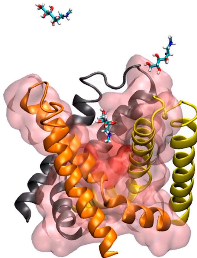
Movie S1. Permeation of 3 \text{NMDG}^+ molecules through the open pore of zP2X4 model (10 ns with C = 0.15 \text{ M} and V_m = -1.5 \text{ V} ).
