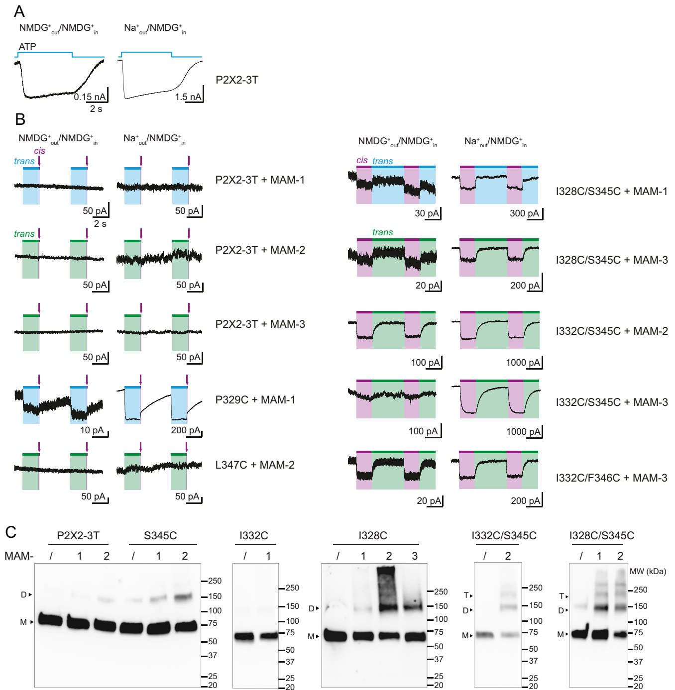
Fig. S6. Molecular mechanism of NMDG + permeation through the lens of opto-tweezers. (A) Macroscopic ATP (30 μM)-gated currents recorded at −60 mV from HEK-293 cells expressing the P2X2–3T. Cells were first bathed in extracellular NMDG + solution (NMDG + out /NMDG + in , Left ) and then rapidly exchanged to extracellular Na + solution (Na + out /NMDG + in , Right ). (B) Macroscopic light-gated currents recorded at −60 mV from HEK-293 cells expressing the indicated mutants treated with the indicated MAMs. Recordings were made as described in A. Illumination was carried out, as indicated, at 365 nm (violet bars) and 455 nm (blue bars) or 530 nm (green bars) to elicit the cis and trans states of the azobenzene, respectively. Short illuminations (80 ms) are indicated by violet arrows. For single mutants treated, cells were briefly preirradiated at 365 nm (80 ms) before recordings. (C) Western blot analysis of cell-surface MAM cross-linking of the indicated P2X2–3T constructs expressed in TSA-201 cells, after treatment with MAM-1, MAM-2, MAM-3, or without MAM (indicated by /). Monomer, dimer, and trimer are indicated.
