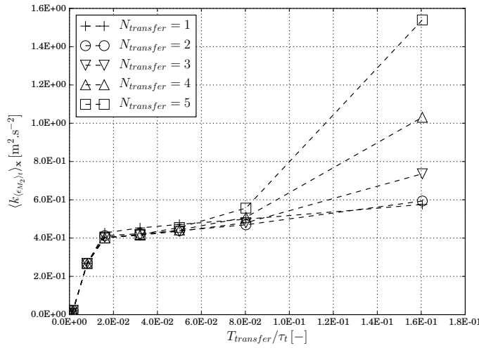
FIGURE 6.7: Measure of the divergence between LES_1 and LES_2 with 192^3 elements with several MR-LES parameters
