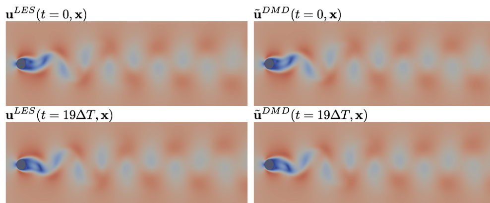
FIGURE 5.8: Reconstruction of the velocity field with four modes and the mean
