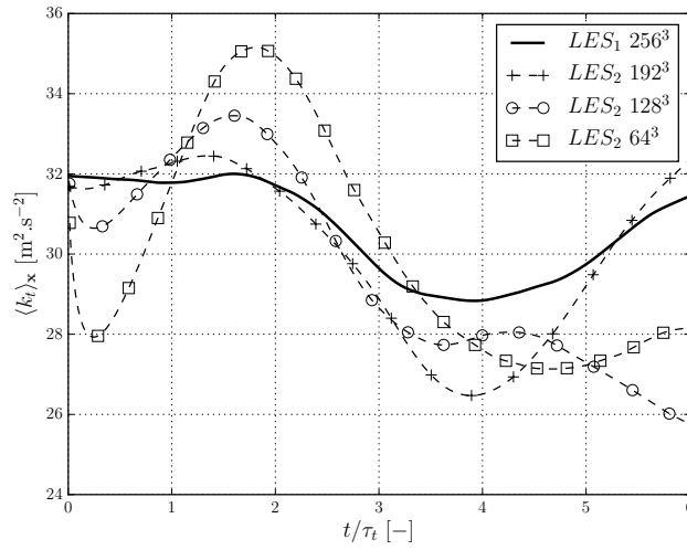
FIGURE 6.6: Off-equilibrium of the average kinetic energy on both LES level
