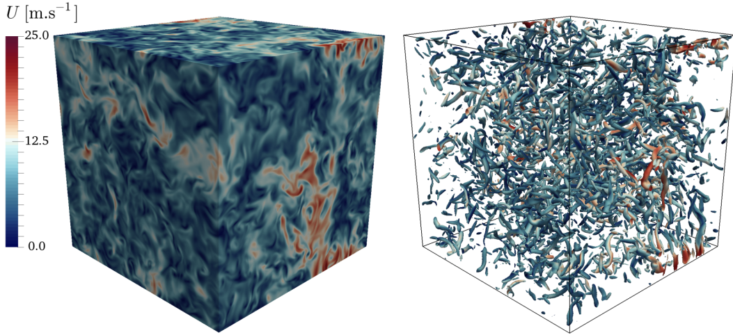
FIGURE 6.4: Instantaneous velocity field (left) and Q-criterion colored by the velocity magnitude of the resulting turbulent flow with the linear forcing source term
