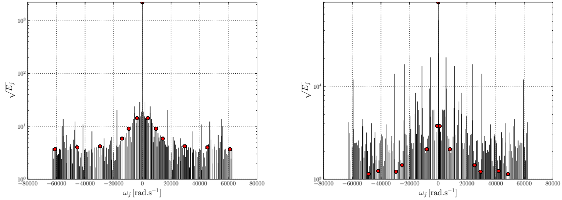
FIGURE 5.15: Energy of the modes for the passive scalar z_{M_0} (left) and the velocity field \mathbf{u}_{M_0} (right)
