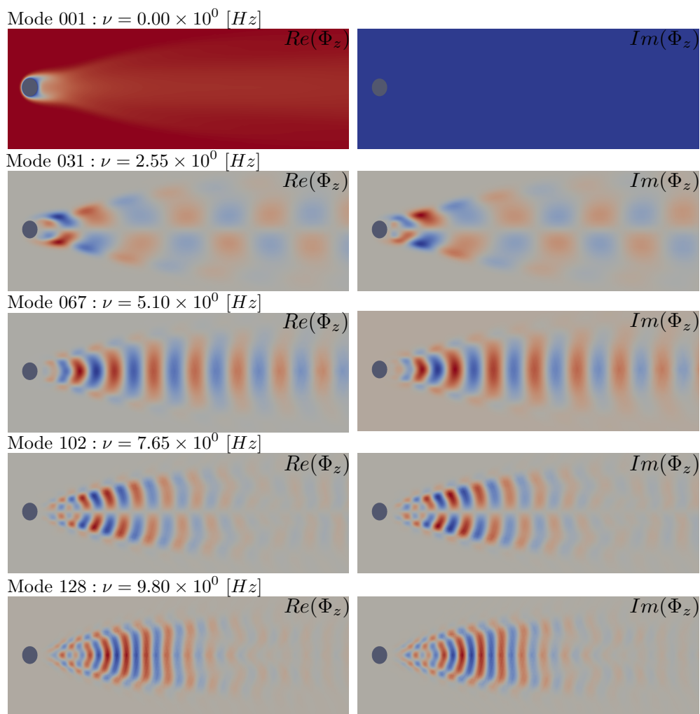
FIGURE 5.12: Dominant DMD modes for the scalar field
