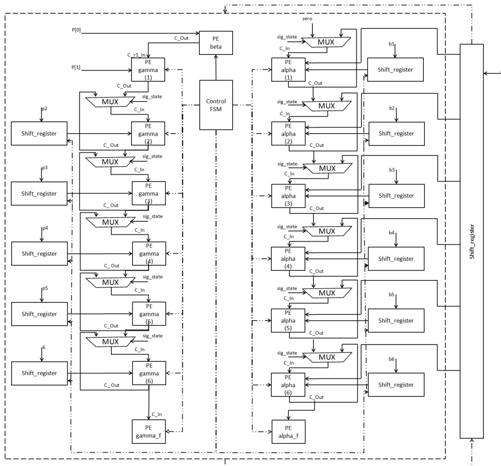
FIGURE C.14 – Proposed Montgomery modular multiplication architecture for the NW-16 version.
