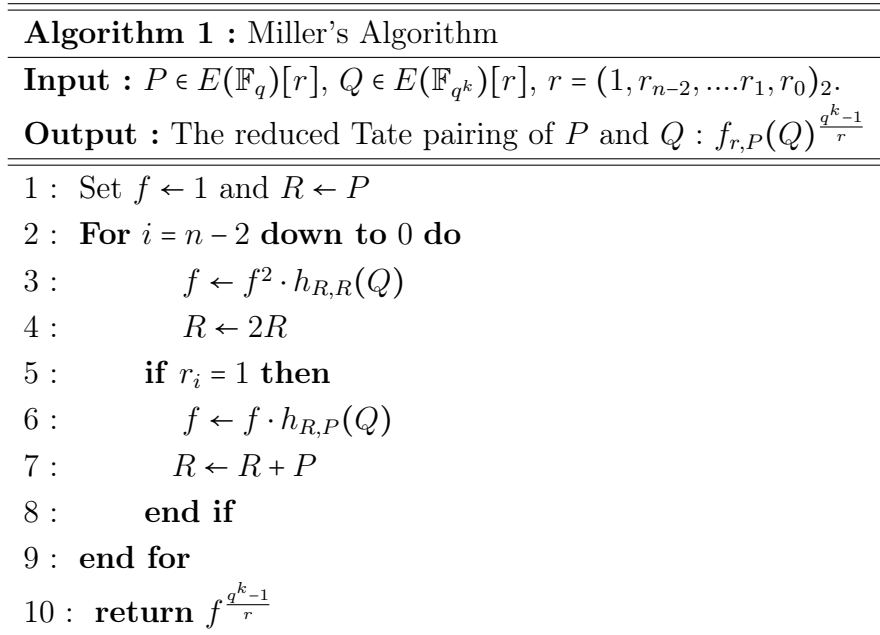
FIGURE D.1 – The Miller algorithm for the computation of the reduced Tate pairing
