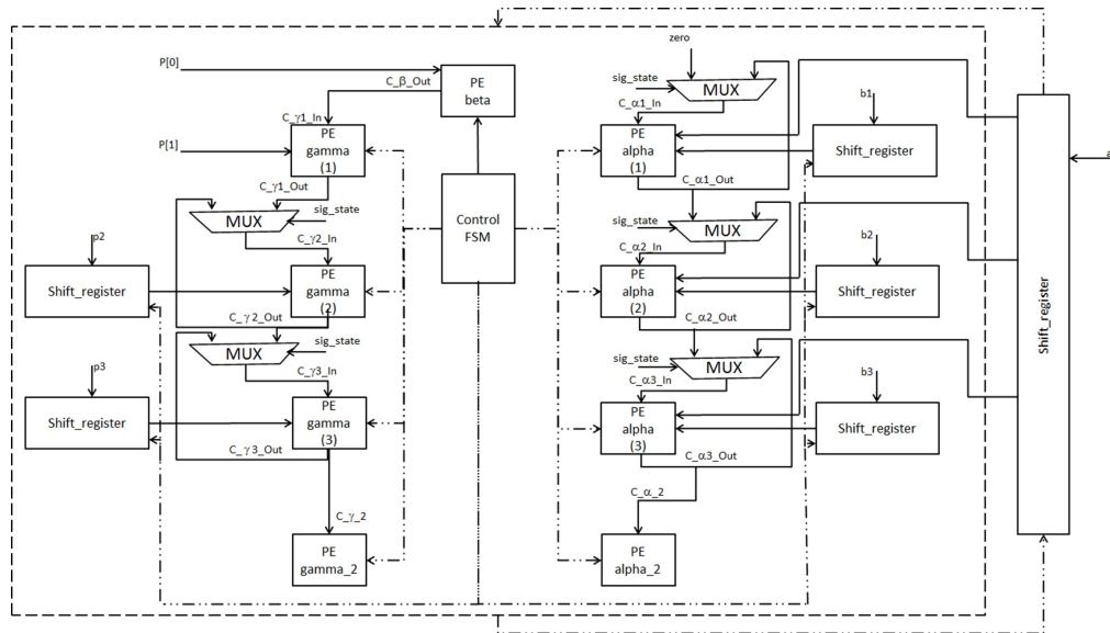
FIGURE C.10 – Proposed Montgomery modular multiplication architecture.
