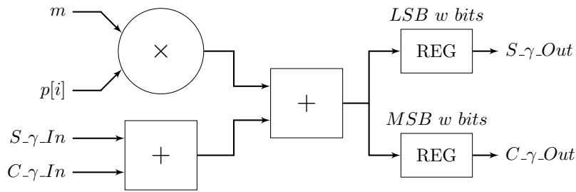
FIGURE C.6 – Gamma Processing Element internal architecture.
