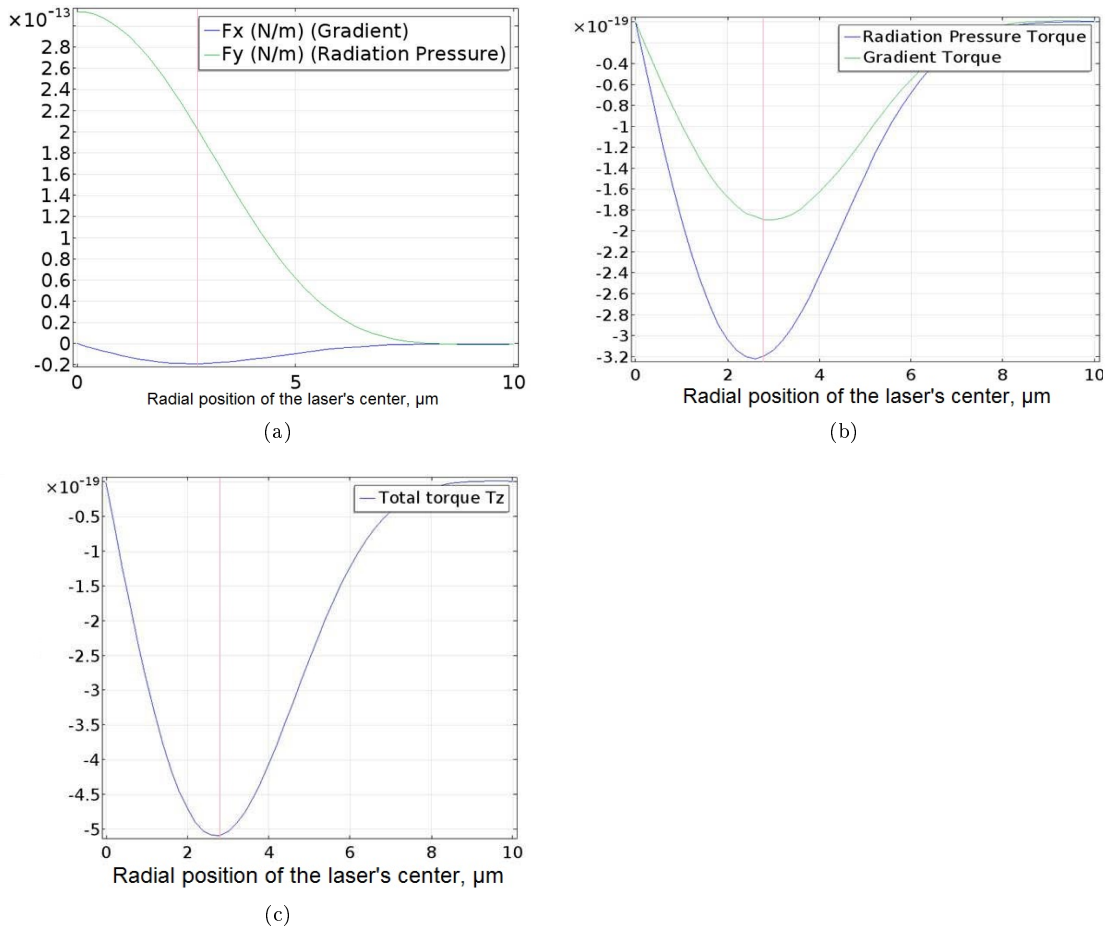
Figure 4.30: (a) Forces appearing in light-matter interaction: radiation pressure (green) and gradient (blue) forces appear along and perpendicular to structure's symmetry axis correspondingly. Negative sign of gradient force just means that its direction is opposite with direction of X axis in used coordinate system. (b) Torques appearing in light-matter interaction due to radiation pressure (blue) and gradient (green) forces. (c) Resulting torque. On all plots rose vertical line shows the edge of the structure, which has a diameter of 5.5\ \mu\text{m} . Calculations were done for the laser diameter of 2\ \mu\text{m} , power of 100\ \mu\text{W} and wavelength of 900\ \text{nm} .
