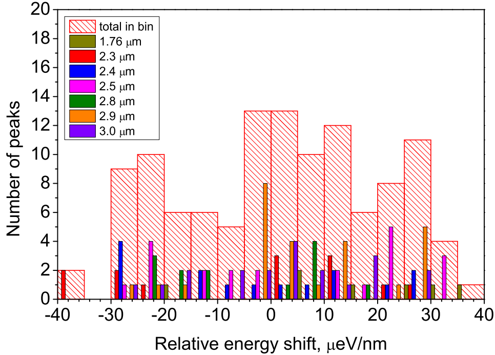
Figure 3.29: The shaded red histogram demonstrates the distribution of peaks' relative energy shifts in \mu\text{eV} per nm of tip's displacement for 7 photonic wires with diameters of 1.76\ \mu\text{m} (dark yellow), 2.3\ \mu\text{m} (red), 2.4\ \mu\text{m} (blue), 2.5\ \mu\text{m} (magenta), 2.8\ \mu\text{m} (dark green), 2.9\ \mu\text{m} (orange), 3.0\ \mu\text{m} (violet) with the size of the bin equals to 5\ \mu\text{eV}/\text{nm} . Independent columns shows the amount of peaks for each structure in certain bin.
